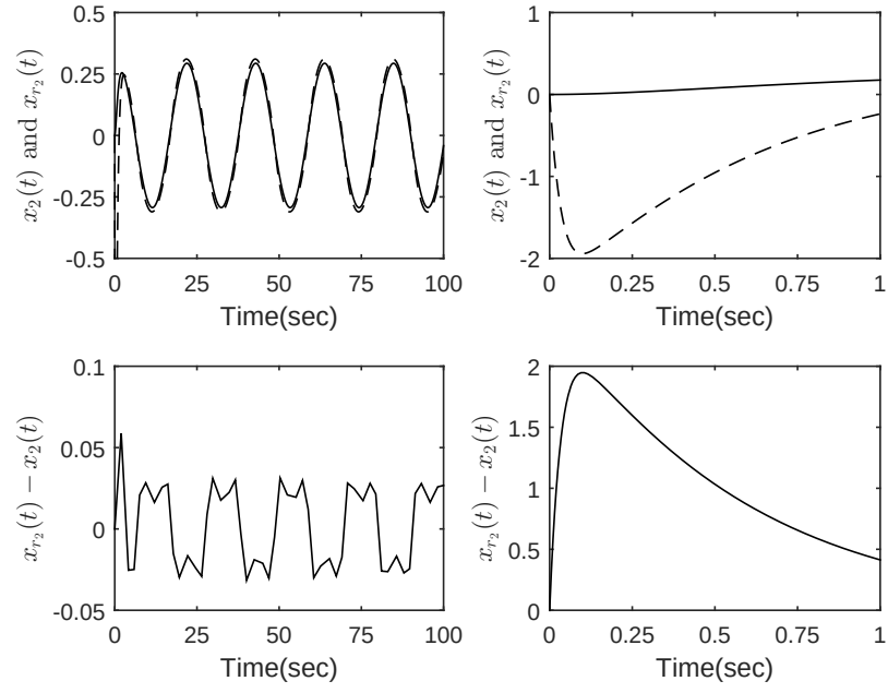
Figure 5.6: Tracking control performance for x_2(t) under 10 sub-domains approach. Top left panel: responses of x_2(t) (Solid line) and x_{r2}(t) (Dash line) from 0 to 100 seconds. Top right panel: responses of x_2(t) (Solid line) and x_{r2}(t) (Dash line) from 0 to 1 second. Bottom left panel: response of x_{r2}(t) - x_2(t) from 0 to 100 seconds. Bottom right panel: response of x_{r2}(t) - x_2(t) from 0 to 1 second.
