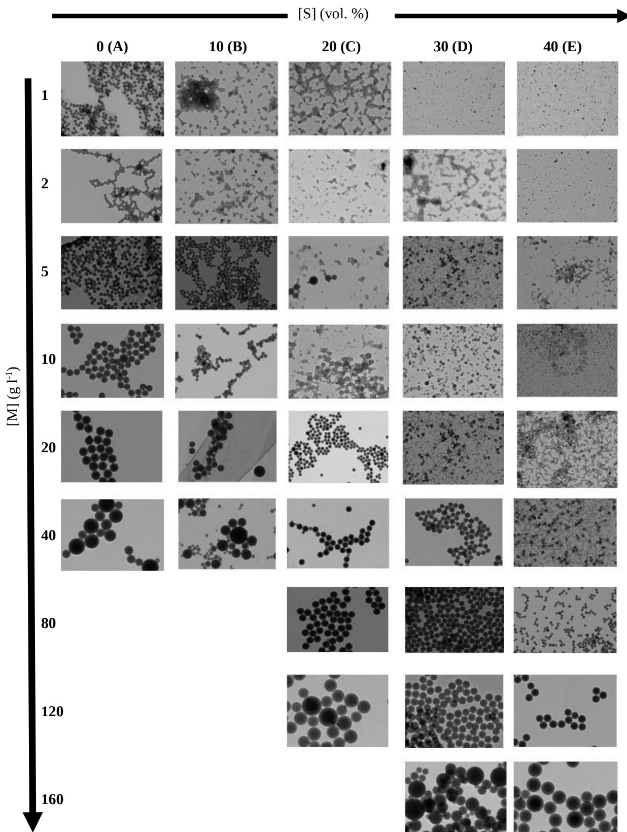
Figure 8.4 TEM micrographs of particles produced by EFEP in the presence of various amount of [S] at different monomer concentrations, [M], (T = 80°C).
