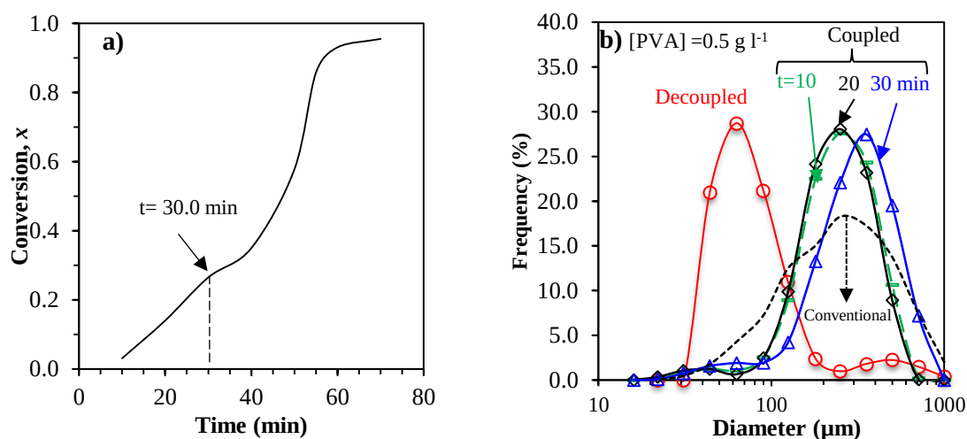
Figure 4.7 a) Variations in conversion versus time. b) Comparison of particle size distributions obtained via coupled two-stage protocols at [\text{PVA}] = 0.5 \text{ g l}^{-1} at different reduction time with the corresponding decoupled and conventional suspension polymerisation ( N_E = 700 \text{ rpm} and N_P = 250 \text{ rpm} ).
