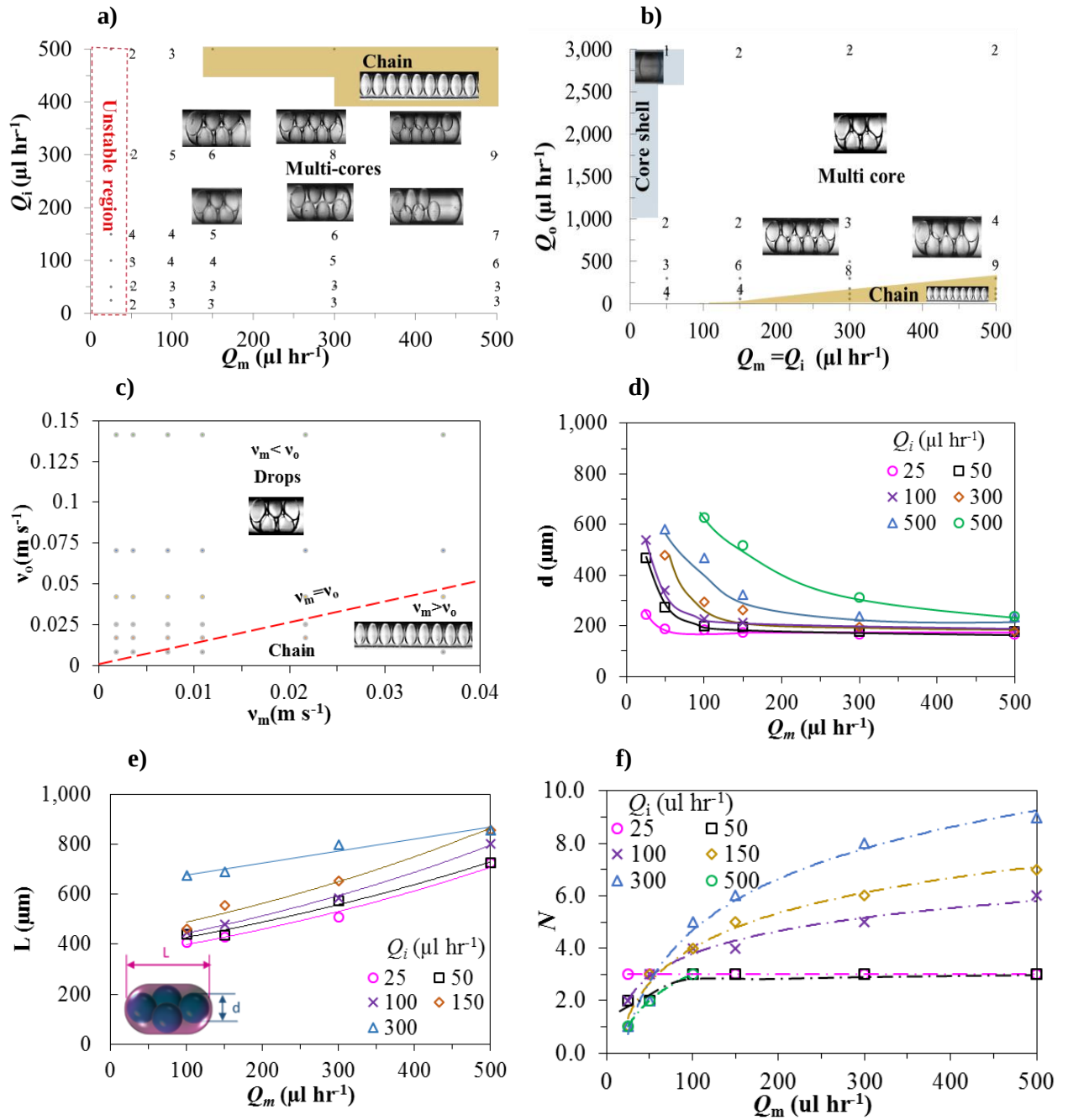
Figure 6.7 Phase maps showing different domains of double drops with controllable number of cores a) in terms of Q_i vs Q_m at a fixed Q_o = 300 \mu\text{l hr}^{-1} and b) in terms Q_o vs Q_m = Q_i . The inset numbers represent the number of internal droplets. The ellipsoid internal droplets is just an optical effect [204]. c) The velocity of the outer phase v_o versus that of the middle phase v_m . The red dotted-line shows the critical transition velocity for drops formation mechanism. d), e) and f) Show variations in the diameter of core, shell axial length, and number of cores, respectively, with Q_m at different Q_i ( Q_o = 300 \mu\text{l hr}^{-1} ).
