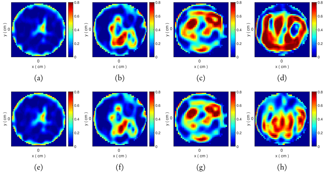
Figure 5.5: Reconstructed images of \sigma_s without and with optimisation of initial guess for 4 phantoms in 2 mm. (a-d) Reconstructions with a fixed initial guess representative of normal breast tissue average properties ( \epsilon_\infty = 5.76, \Delta\epsilon = 5.51, \sigma_s = 0.0802 ); (e-h) Reconstructions with an optimised initial guess
