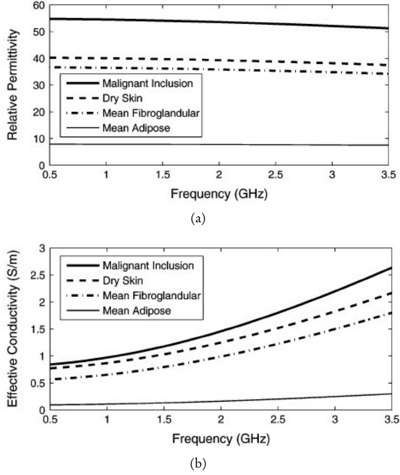
Figure 2.2: Frequency dependence of the single-pole Debye tissue models used in the numerical breast phantoms. (a) \epsilon_r and (b) \sigma_{eff} . The curves for adipose and fibroglandular tissues represent the mean of the full mapping range from the raw MRI data.
