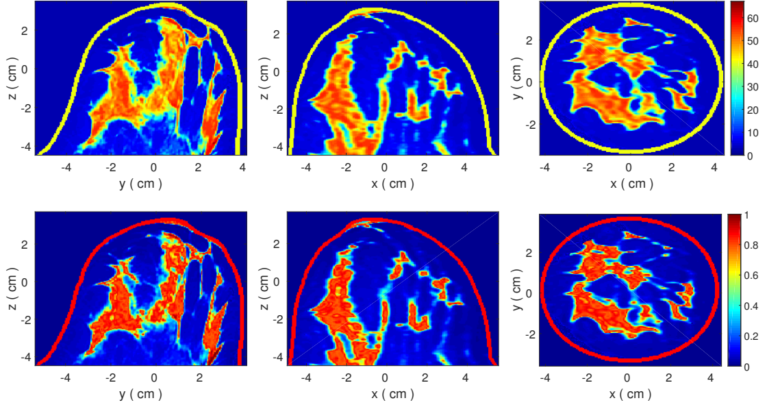
Figure 2.5: Relative permittivity and effective conductivity of the heterogeneously dense 3-D numerical breast phantom distributions at 1.0 GHz. (a) \epsilon_r in y-z plane. (b) \epsilon_r in x-z plane. (c) \epsilon_r in x-y plane. (d) \sigma_{eff} in y-z plane. (e) \sigma_{eff} in x-z plane. (f) \sigma_{eff} in x-y plane.
