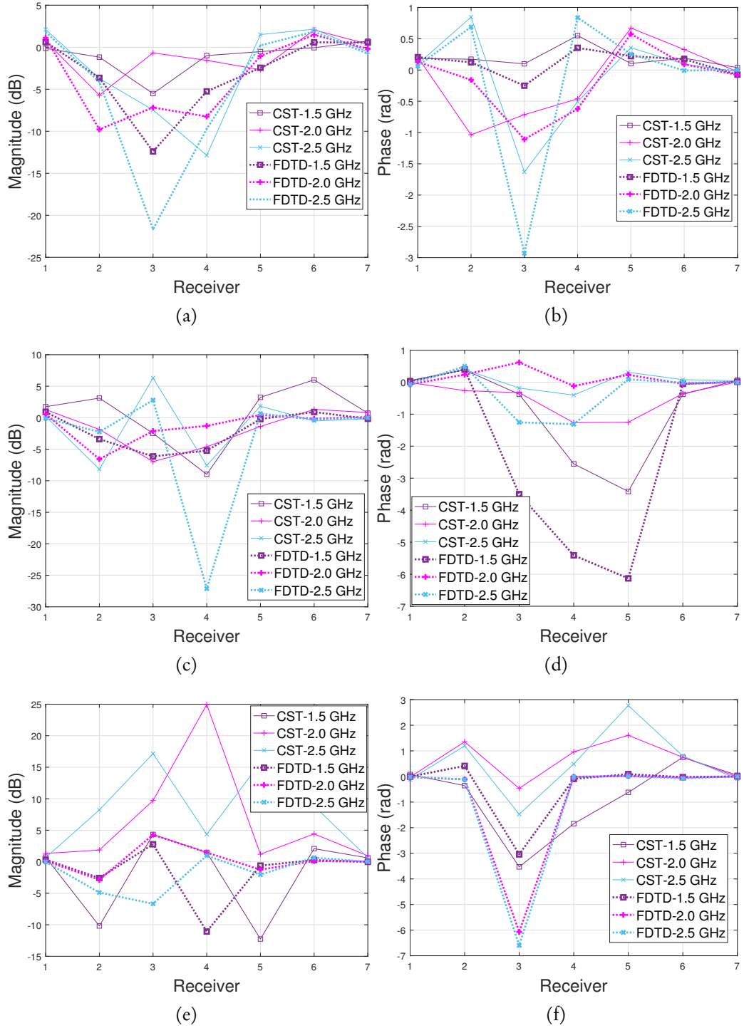
Figure 6.7: Comparison of the measurement differences (with target versus without target) between 3-D and 2-D simulations in condition of the transmitter 1. (a-b) in coupling medium of Triton X-100; (c-d) in coupling medium of 90% corn syrup; (e-f) in coupling medium of 80% Glycerine.
