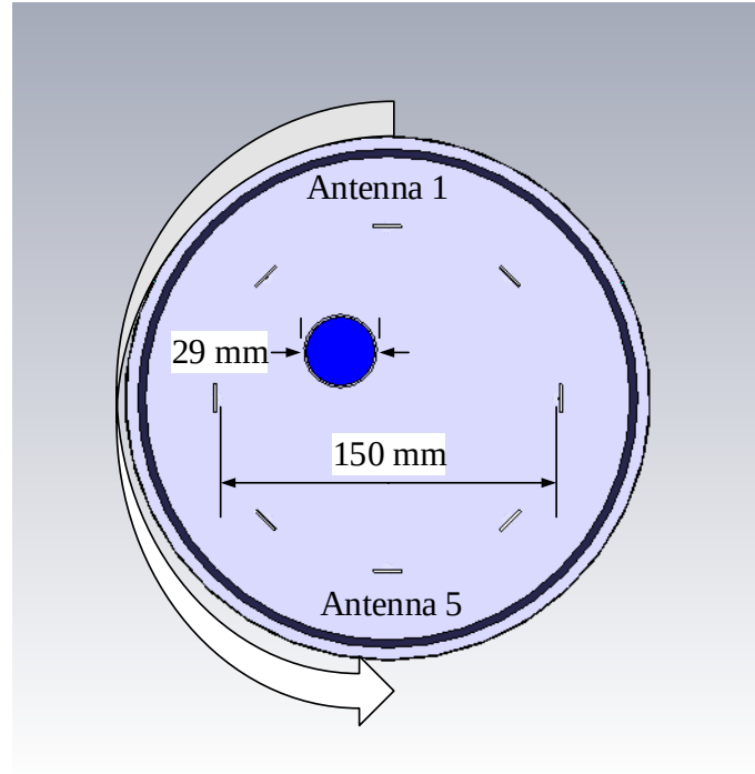
Figure 6.6: Geometry of the eight-antenna system with a simple target in a cylinder filled with pure water.
