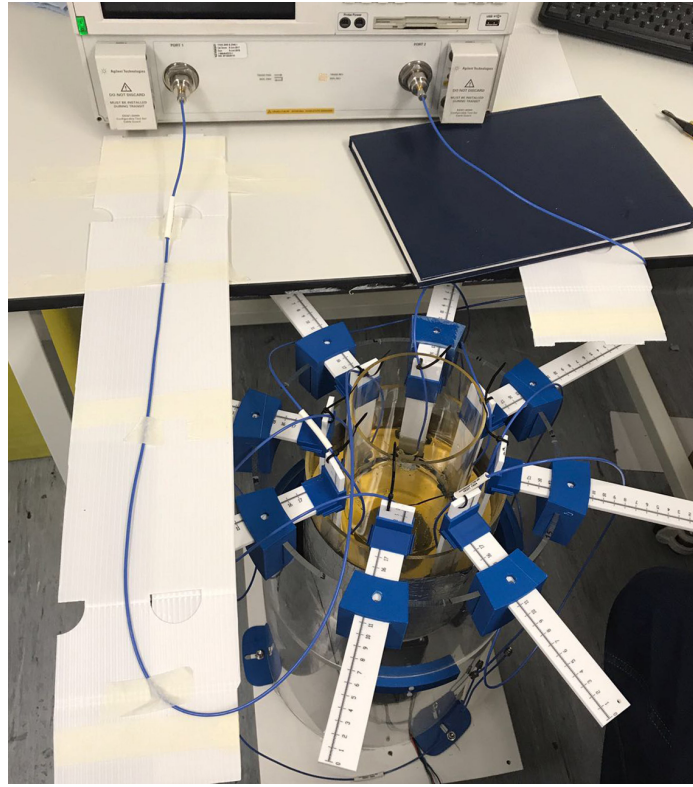
Figure 6.14: Photo of our experimental MWI system
