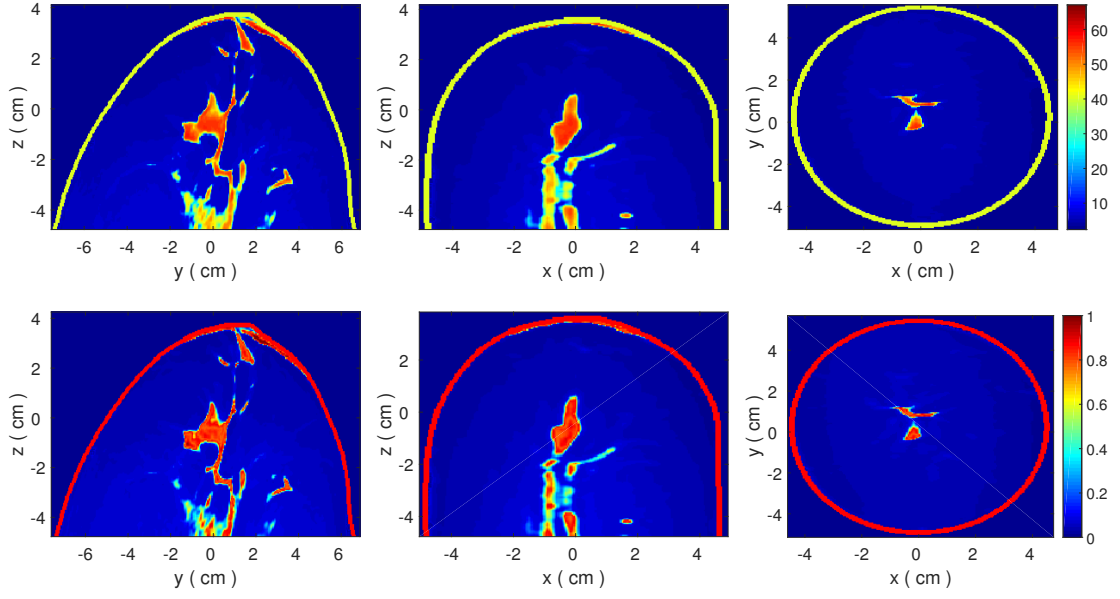
Figure 2.3: Relative permittivity and effective conductivity of the mostly fatty 3-D numerical breast phantom distributions at 1.0 GHz. (a) \epsilon_r in y-z plane. (b) \epsilon_r in x-z plane. (c) \epsilon_r in x-y plane. (d) \sigma_{eff} in y-z plane. (e) \sigma_{eff} in x-z plane. (f) \sigma_{eff} in x-y plane.
