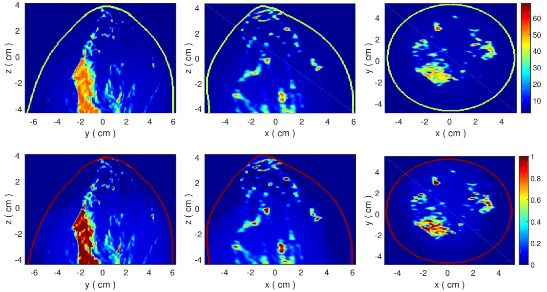
Figure 2.4: Relative permittivity and effective conductivity of the scattered fibroglandular 3-D numerical breast phantom distributions at 1.0 GHz. (a) \epsilon_r in y-z plane. (b) \epsilon_r in x-z plane. (c) \epsilon_r in x-y plane. (d) \sigma_{eff} in y-z plane. (e) \sigma_{eff} in x-z plane. (f) \sigma_{eff} in x-y plane.
