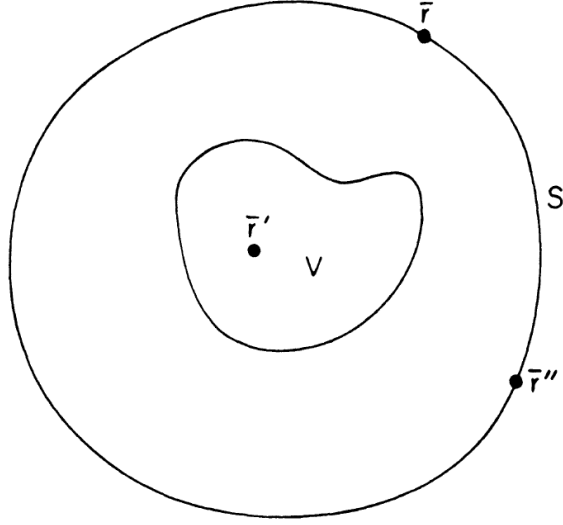
Figure 2.9: An inverse scattering experiment where the measurement data are obtained at \bar{r} on S and the transmitter is at \bar{r}''
