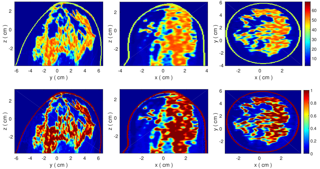
Figure 2.6: Relative permittivity and effective conductivity of the very dense 3-D numerical breast phantom distributions at 1.0 GHz. (a) \epsilon_r in y-z plane. (b) \epsilon_r in x-z plane. (c) \epsilon_r in x-y plane. (d) \sigma_{eff} in y-z plane. (e) \sigma_{eff} in x-z plane. (f) \sigma_{eff} in x-y plane.
