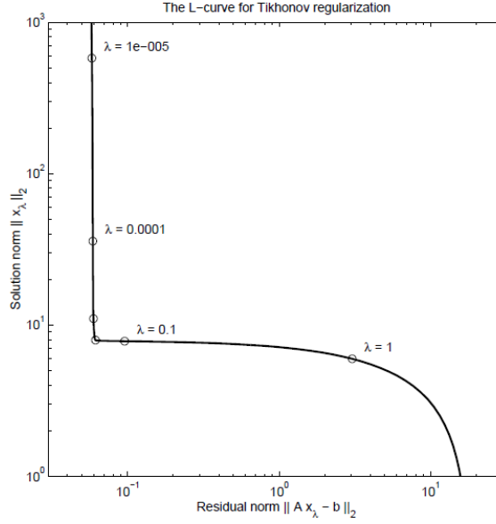
Figure 4.1: An example of L-curve plot
