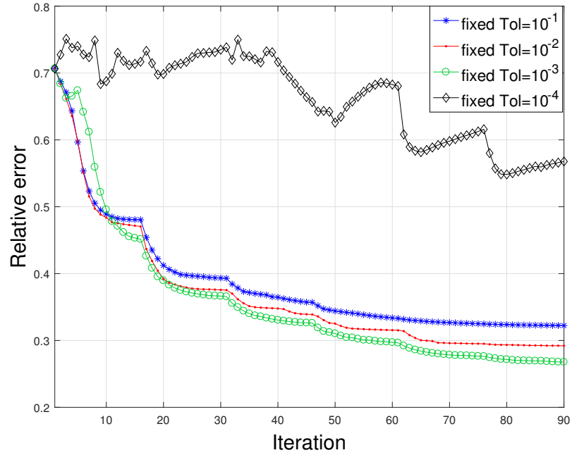
Figure 3.3: Comparison of the results in different tolerance values with known skin in 90 iterations by TwIST method and frequency hopping method.
