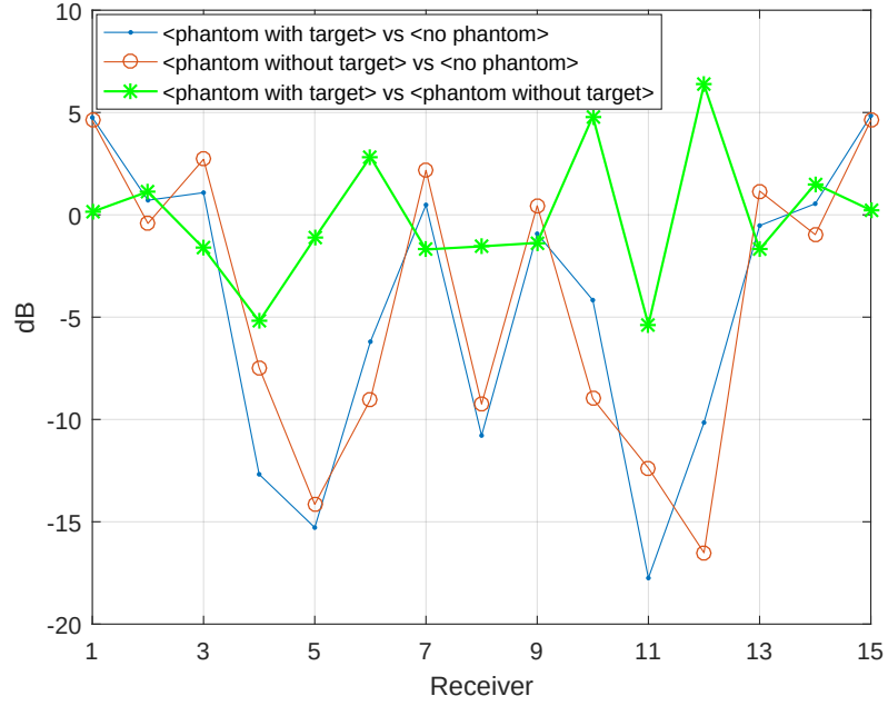
Figure 6.4: Measured amplitudes of the signals scattered from the target and phantom, the phantom alone, and their difference. The data was measured by the receiver at 15 different angles surrounding the phantom evenly, as the transmitter is fixed at the same position.
