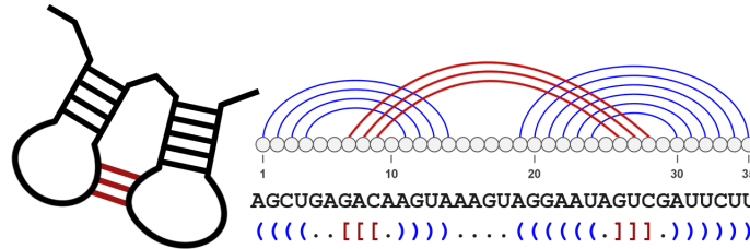
Fig. 2.6 Kissing hairpin pseudoknot.
