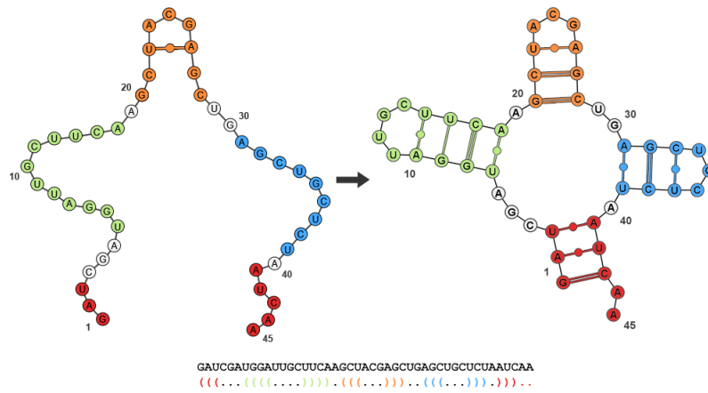
Fig. 2.8 RNA secondary structure dot-bracket representation.
