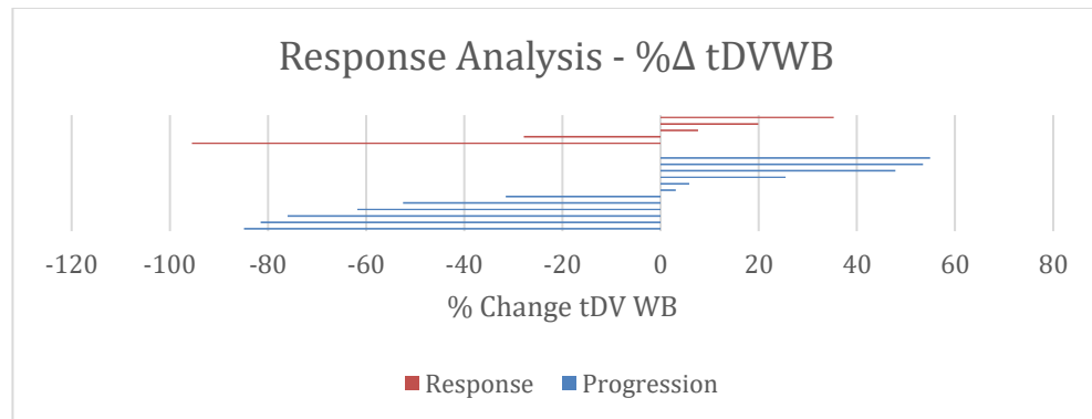
Figure 13-3: WB DW-MRI; \% \Delta tDV WB Parameters; Response Analysis; Waterfall plot of all patients
