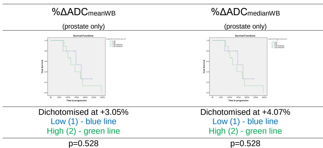
Figure 13-20: WB DW-MRI; PFS Analysis; \% \Delta WB ADC Parameters; Prostate patients only; KM Analysis
