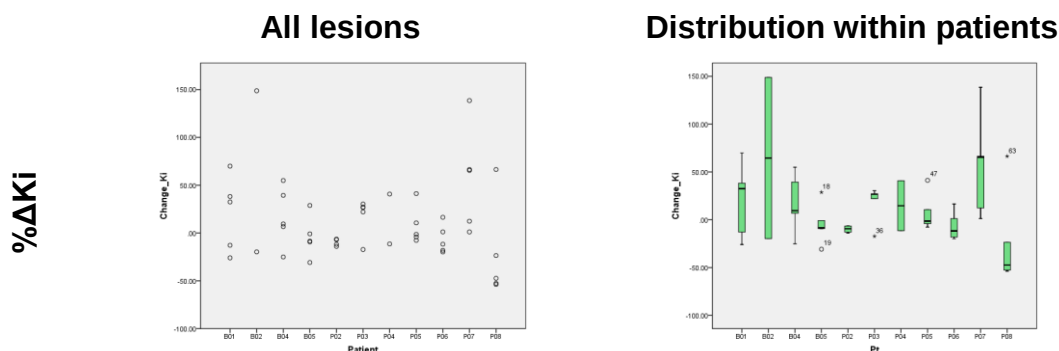
Figure 3-21: 18 F-Fluoride Per-lesion analysis; % \Delta Ki
