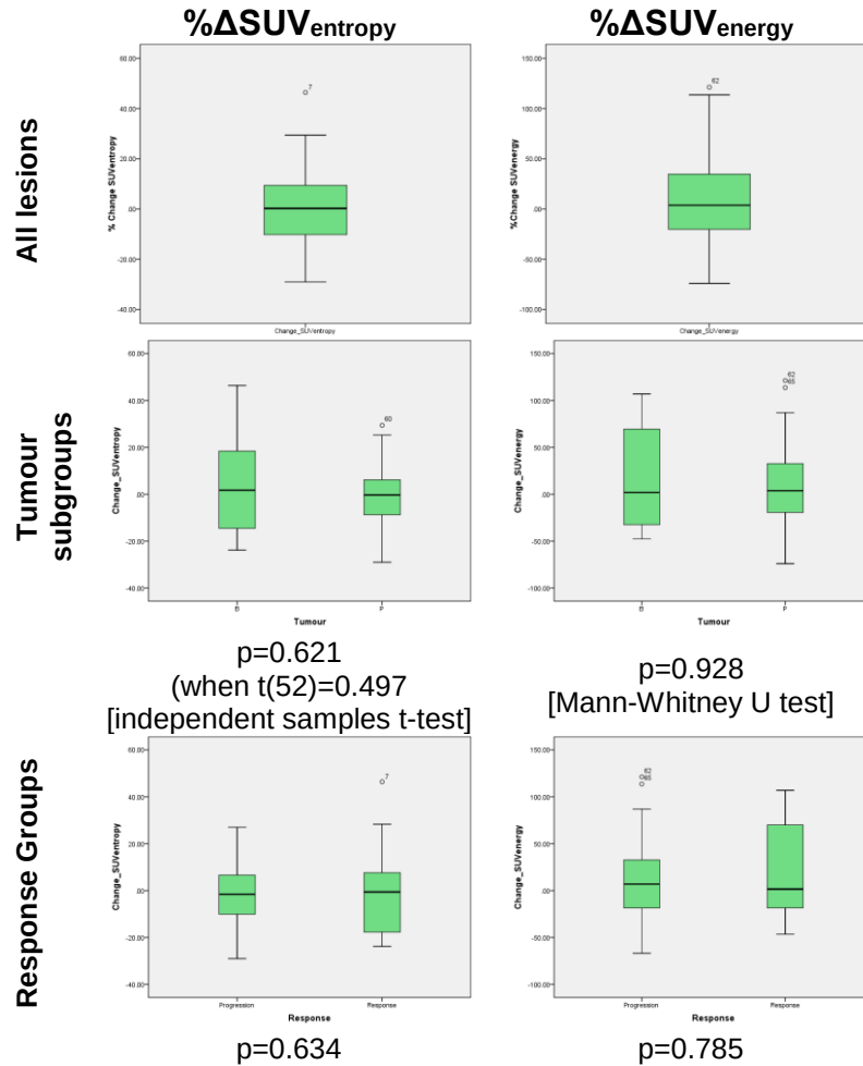
Figure 3-18: 18 F-Fluoride PET Per-lesion analysis; Descriptive statistics of %Δ SUV Heterogeneity Parameters (B - Breast cancer patients; P – Prostate cancer)
