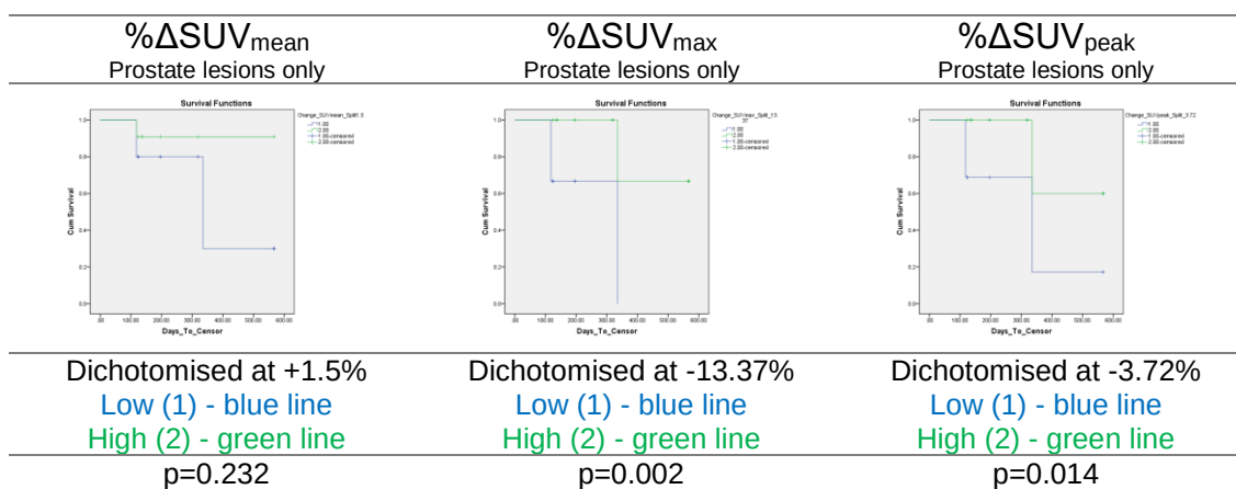
Figure 4-8: 18 F-Fluoride PET Per-lesion analysis; \% \Delta SUV Parameters; OS analysis with KM analysis and log rank for comparison; Prostate lesions only
