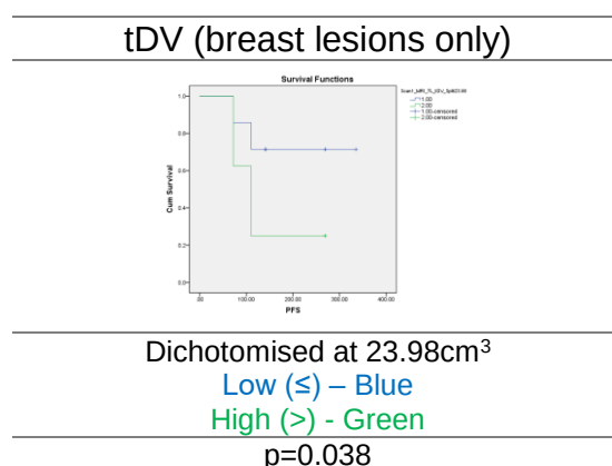
Figure 10-12: DW-MRI Per-lesion Analysis; KM PFS Analysis; Baseline tDV; Breast lesions
