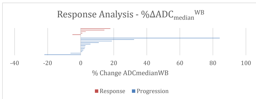
Figure 13-2: WB DW-MRI; \% \Delta \text{ADC}_{\text{medianWB}} Parameters; Response Analysis; Waterfall plot of all patients
