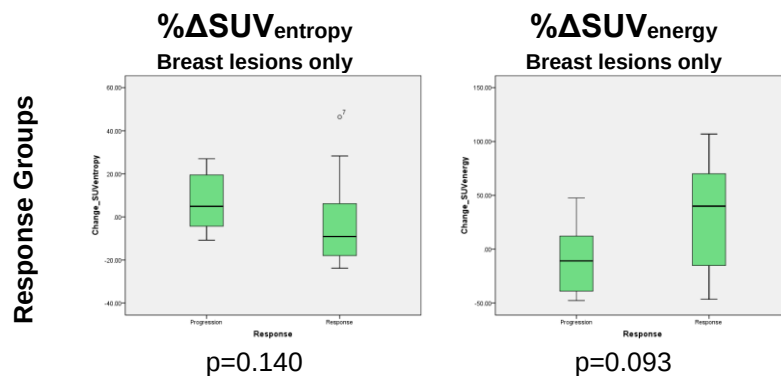
Figure 3-19: 18 F-Fluoride PET Per-lesion analysis; Descriptive statistics of %Δ SUV Heterogeneity Parameters; breast lesions only; comparisons with Mann-Whitney U tests
