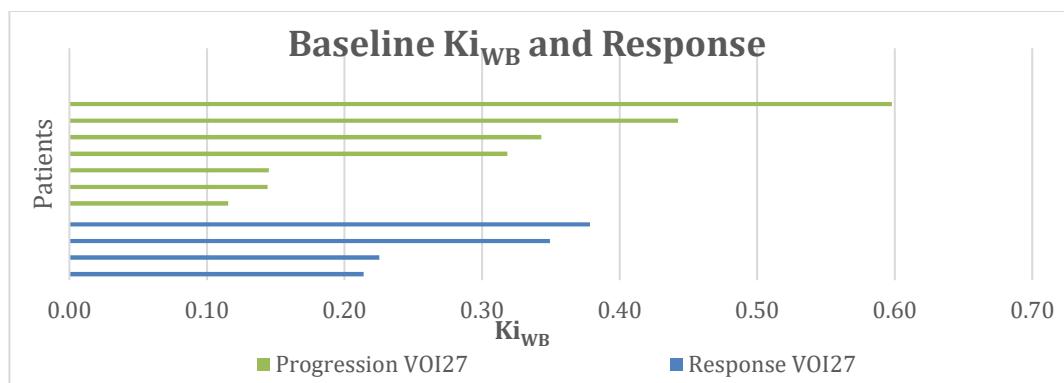
Figure 8-8: 18 F-Fluoride PET; Whole-Body Analysis; Baseline Ki_{WB}^{VOI27} ; all patients split into response groups (Progression=Green; Response=Blue)
