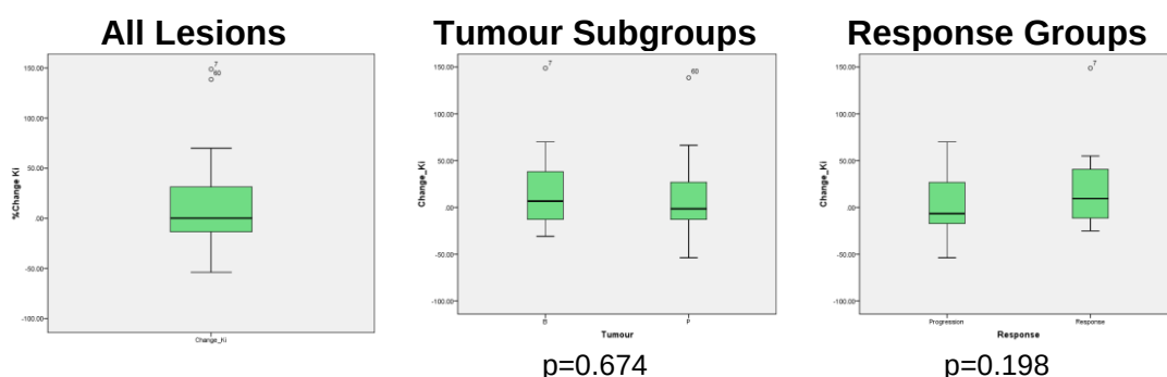
Figure 3-22: 18 F-Fluoride PET Per-lesion analysis; Descriptive statistics of % \Delta Ki (B - Breast cancer patients; P – Prostate cancer)
