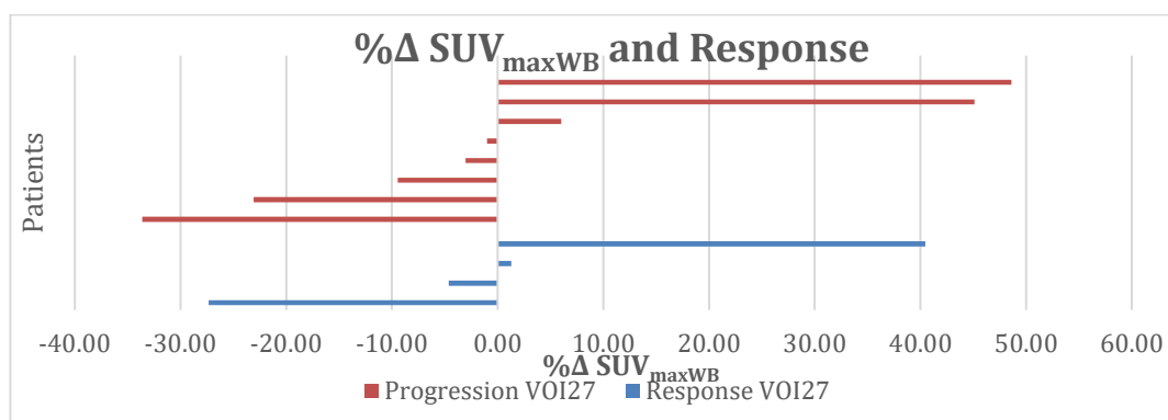
Figure 8-10: 18 F-Fluoride PET; Whole-Body Analysis; %ΔSUV maxWB VOI27 ; all patients split into response groups
