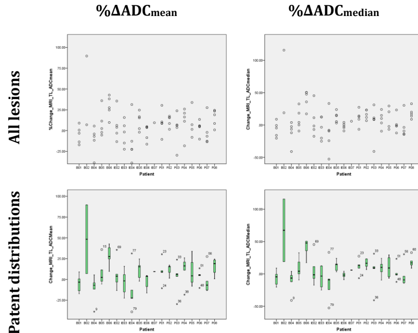
Figure 9-7: DW-MRI Per-lesion Analysis; % \Delta ADC Parameters (% \Delta ADC mean -left, % \Delta ADC median -right); TOP – all lesions for all patients; BOTTOM – ADC distributions for all patients
