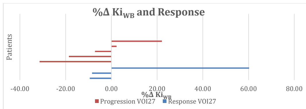
Figure 8-16: 18 F-Fluoride PET; Whole-Body Analysis; %ΔK iWB VOI27 ; all patients split into response groups
