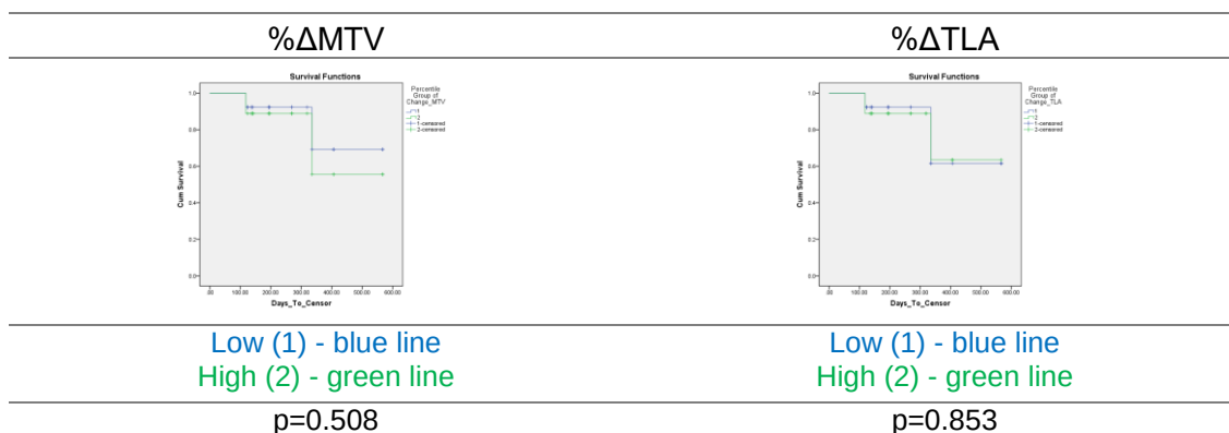
Figure 4-9: 18 F-Fluoride PET Per-lesion analysis; \% \Delta Volumetric Parameters; OS analysis with KM analysis and log rank for comparison; All lesions
