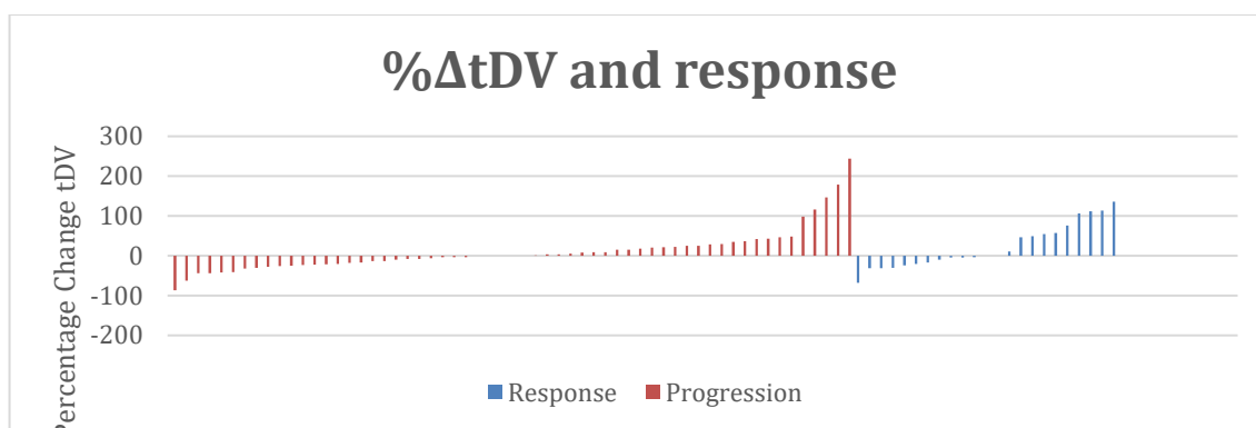
Figure 9-13: DW-MRI Per-lesion Analysis; Waterfall plot for %ΔtDV Parameters; Response analysis
