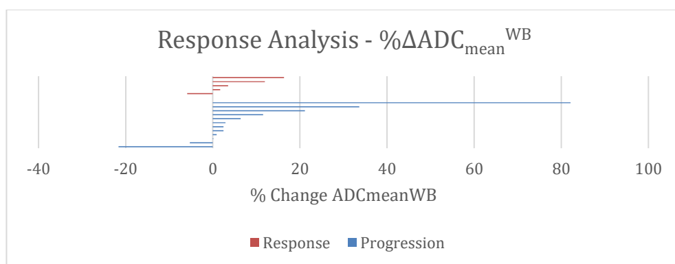
Figure 13-1: WB DW-MRI; \% \Delta \text{ADC}_{\text{meanWB}} Parameters; Response Analysis; Waterfall plot of all patients
