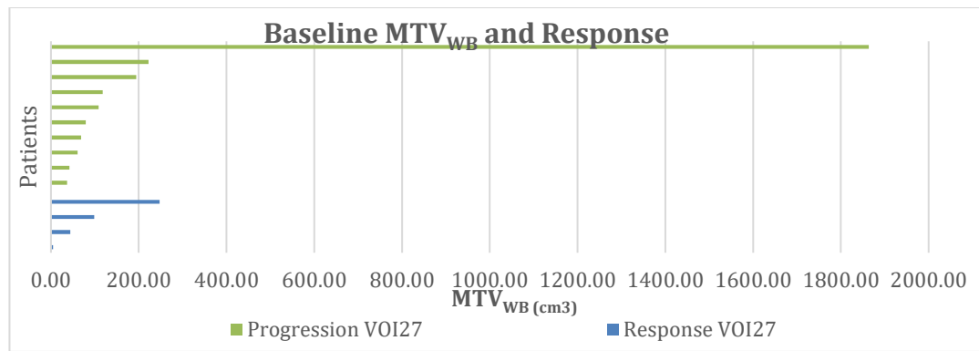
Figure 8-4: 18 F-Fluoride PET; Whole-Body Analysis; Baseline MTV WB VOI27 ; all patients split into response groups (Progression=Green; Response=Blue)
