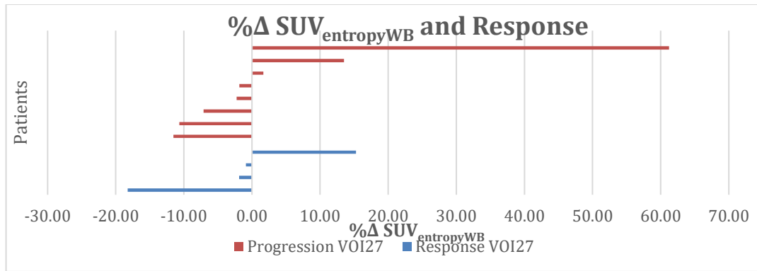
Figure 8-14: 18 F-Fluoride PET; Whole-Body Analysis; %ΔSUV entropyWB VOI27 ; all patients split into response groups
