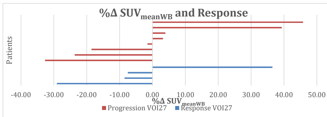
Figure 8-9: 18 F-Fluoride PET; Whole-Body Analysis; %ΔSUV meanWB VOI27 ; all patients split into response groups
