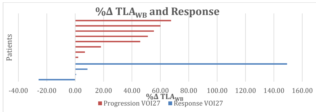
Figure 8-13: ^{18}\text{F} -Fluoride PET; Whole-Body Analysis; \% \Delta \text{TLA}_{\text{WB}}^{\text{VOI27}} ; all patients split into response groups (Progression=Grey; Response=Blue)
