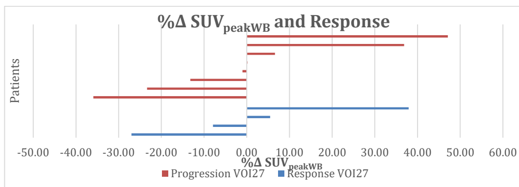
Figure 8-11: 18 F-Fluoride PET; Whole-Body Analysis; %ΔSUV peakWB VOI27 ; all patients split into response groups
