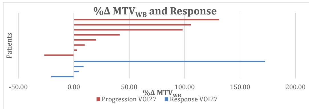
Figure 8-12: ^{18}\text{F} -Fluoride PET; Whole-Body Analysis; \% \Delta \text{MTV}_{\text{WB}}^{\text{VOI27}} ; all patients split into response groups (Progression=Grey; Response=Blue)
