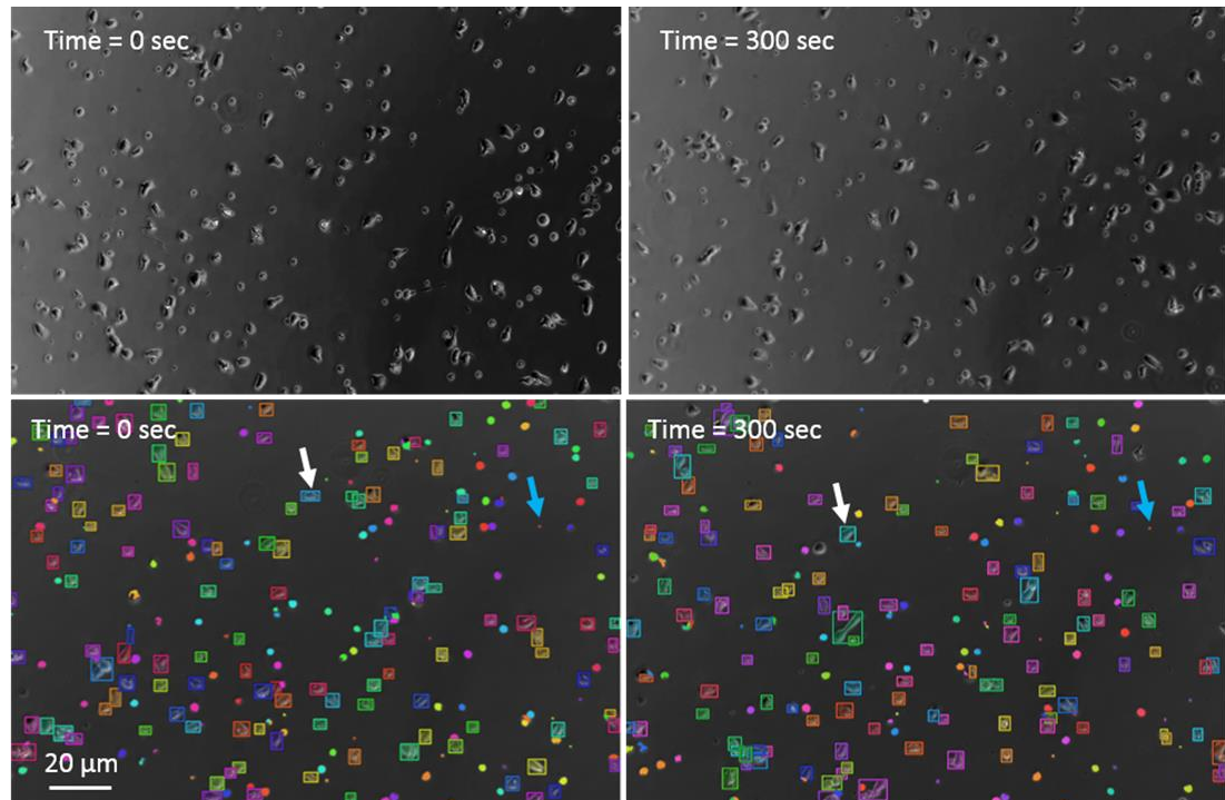
Figure 5-1: Phase contrast movies and automatic tracking stills. Boxes denote cells undergoing tracking,. The white arrow denotes a cell that has been tracked, and the blue arrow a piece of debris that has been ignored.
