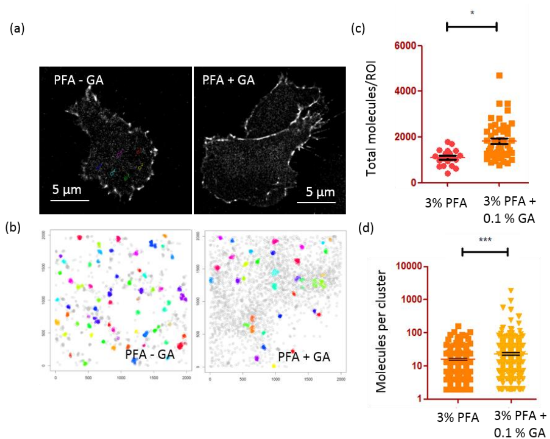
Figure 3-4: Effects of glutaraldehyde inclusion during cell fixation. A) Pointillist maps of cells fixed with PFA alone (left) or PFA + 0.1 % GA. b) example regions with clusters identified in arbitrary colours. c) plots showing total molecules per region and d) the number of molecules per cluster. n = 12 cells and 62 regions of interest. *P < 0.01 , ***P < 0.0001.
