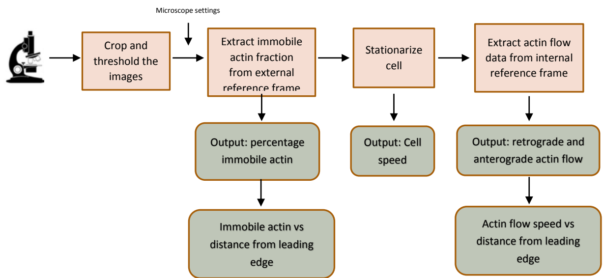
Figure 2-6: STICS analysis flow diagram showing output summary and metrics taken from actin vector fields.
