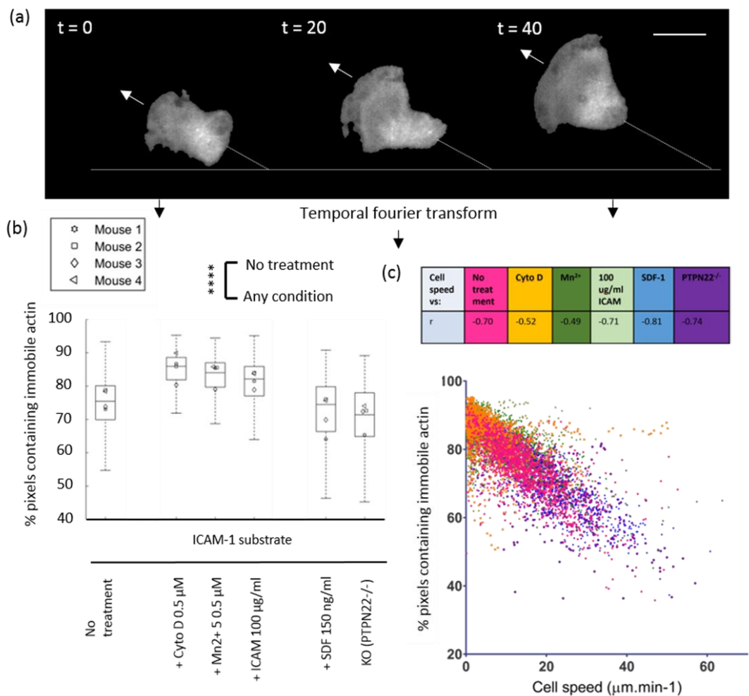
Figure 4-13: Percentage of pixels containing immobile actin is inversely correlated to cell speed. a) Still from a TIRF movie (external reference frame) of IaGFP in a migrating T cell. White arrow = direction of migration. Dashed white line shows displacement in the external reference frame. b) plot of percentage of total pixels containing > 50 % immobile actin for each condition. c) plot of percentage pixels containing immobile actin versus individual cell speeds. Individual conditions are colour coded in the table, their spearman's r values listed.
