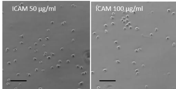
Figure 4-5: 10 x phase contrast movie frames showing cells migrating on different concentrations of ICAM-1 on the coverslip. Migrating cells on a 50 \mu\text{g/ml} or 100 \mu\text{g/ml} ICAM-1 surface. Scale bar 40 \mu\text{m} .
