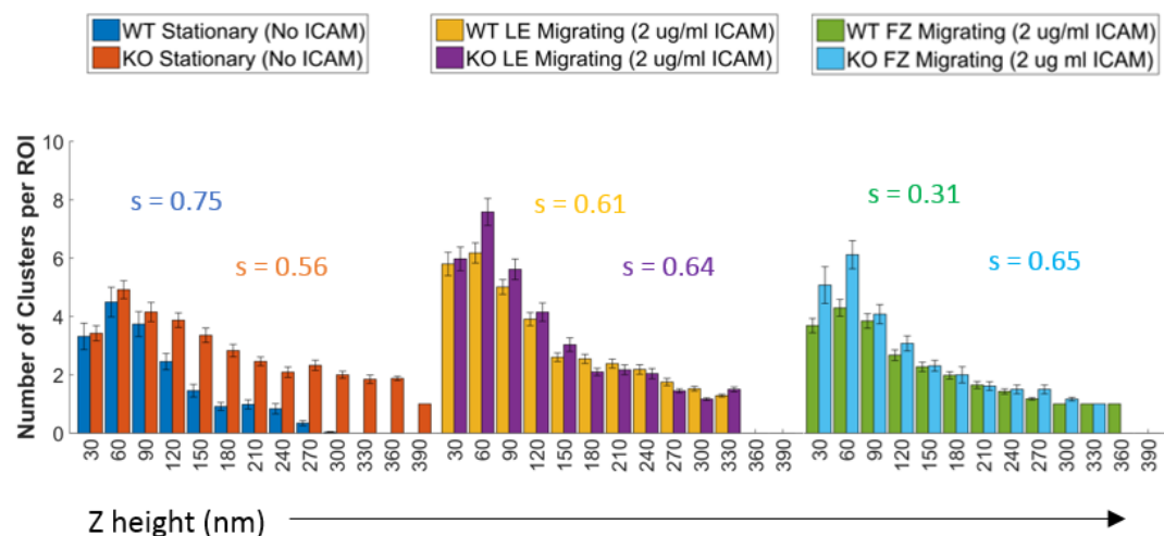
Figure 6-9: Number of pY3197FAK clusters per region plotted against z height: stationary cells and the leading edge/focal zone of migrating cells that were proficient or deficient for PTPN22 imaged by iPALM and analysed using 3D Bayesian cluster analysis. The leftmost plots are conditions: PTPN22+/+ and KO stationary (0 ICAM-1). In the middle are PTPN22+/+ and KO leading edge migrating cells. On the right are PTPN22+/+ and KO focal zone of migrating cells. Skewness values are colour coded for each plot. N = 3 mice, 20 cells and 200 ROIs per condition.
