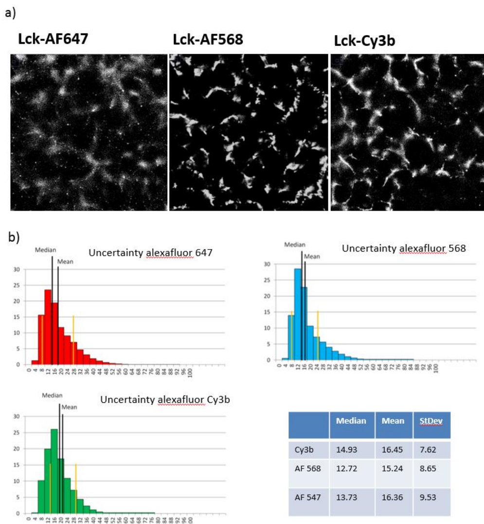
Figure 3-19: Pointillist STORM maps of Lck labelled with three different fluorophores A) The staining pattern of Lck stained with alexafluor 568 and Cy3b were compared with the best fluorophore for STORM: alexafluor 647. B) Uncertainty is the same for Lck tagged with af 647, Cy3b or af 568. Each localisation has a precision level or “uncertainty” based chiefly on the number of photons emitted. Uncertainty values for the three fluorophores tested here for two colour STORM were very similar.
