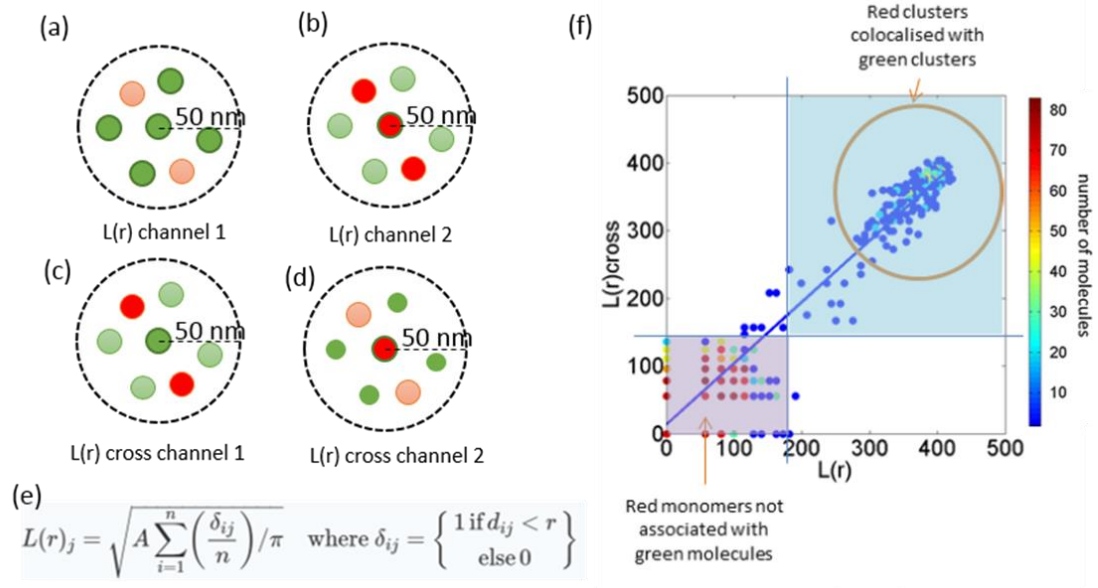
Figure 6-25: Rossey colocalization method. a and b) a search radius of 50 nm is drawn around each point j , for each channel. Ripley's K analysis (e) is carried out for each point, and L(r) derived. c) shows cross analysis, where red points are counted centred around each green point j , and vice versa (d). f) Example figure adapted from Rossey et al. L(r) cross vs L(r) . Plot shows a very strong correlation, indicating a high degree of co-clustering. The pseudo-colour represents the number of individual molecules at each position.
