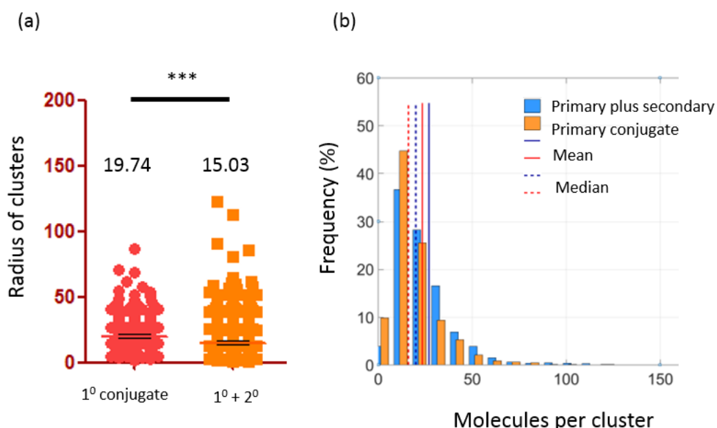
Figure 3-7: Comparison of the size of clusters and number of molecules per cluster when using labelled primary antibodies versus primaries and labelled secondaries. A) plot of the radius of clusters and b) the molecules per cluster in each method.
