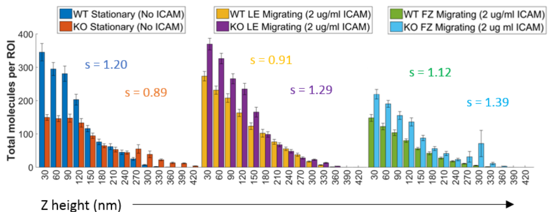
Figure 6-7: Total pY3197FAK molecules per region plotted against z height, stationary cells and the leading edge/focal zone of migrating cells that were proficient or deficient for PTPN22 imaged by iPALM and analysed using 3D Bayesian cluster analysis. The leftmost plots are conditions: PTPN22 +/+ and KO stationary (0 ICAM-1). In the middle are PTPN22 +/+ and KO leading edge migrating cells. On the right are PTPN22 +/+ and KO focal zone of migrating cells. Skewness values are colour coded for each plot. N = 3 mice, 20 cells and 200 ROIs per condition.
