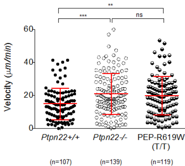
Figure 1-10: PTPN22 -/- and PEP-R619W murine T-cells migrate faster than PTPN22 +/+ . Plot shows velocities (µm/min) of individually tracked (ImageJ manual tracking plugin) effector T-cells migrating on glass coated with 2µg/ml mrlCAM-1.
