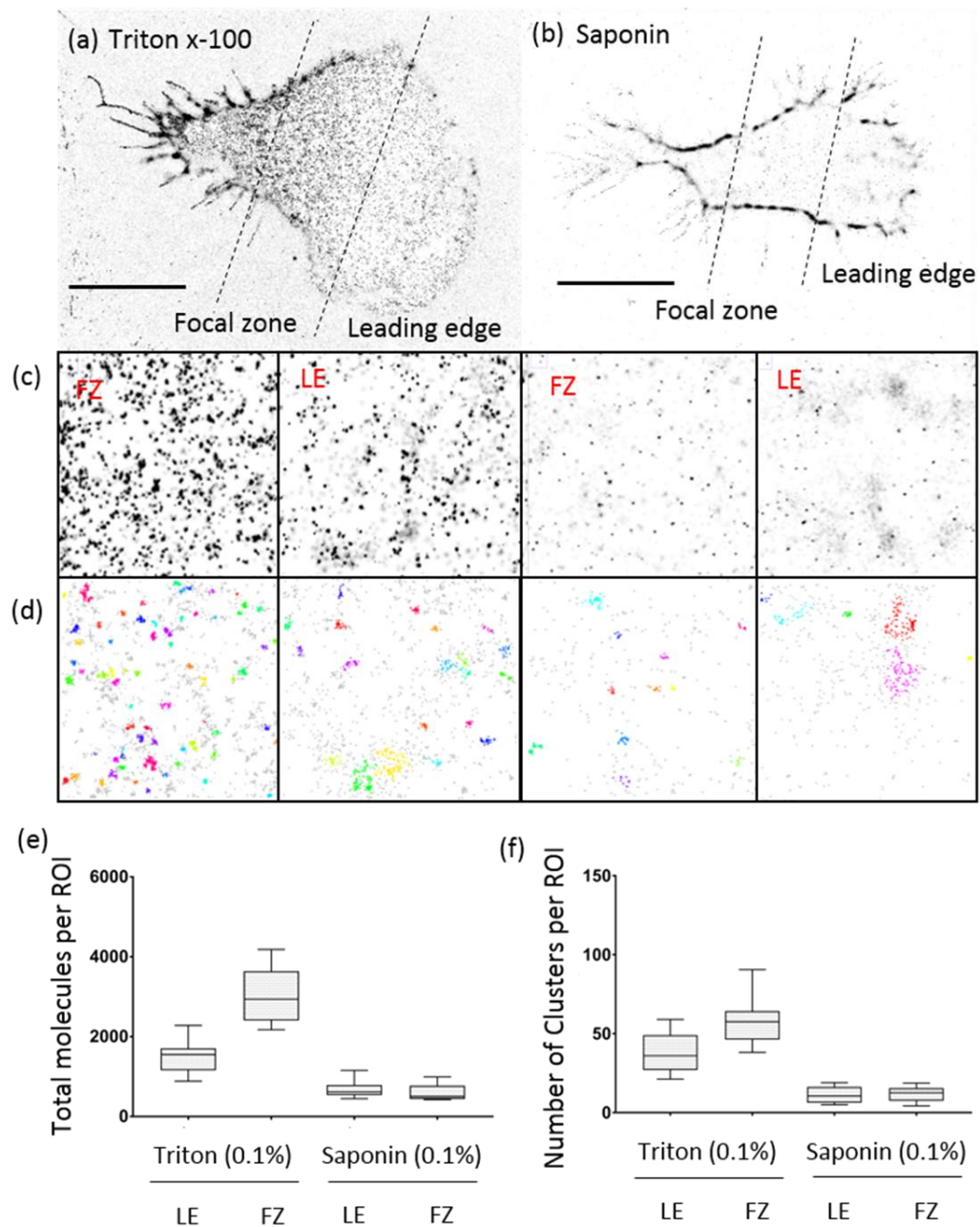
Figure 6-12: Triton permeabilisation allows pY416 Src antibody into cells, whereas saponin staining prevents this. Migrating T cells were fixed and permeabilised with triton (a) or saponin (b) for 10 minutes at 0.1 %. Cells were stained with pY416 Src, an antibody to an intracellular target and imaged by dSTORM (zoomed regions shown in (c) and analysed by Bayesian cluster analysis: example cluster maps are shown in (d). E) plot of total molecules and f) number of clusters in triton treated versus saponin treated cells. Scale bar 4 \mu\text{m} .
