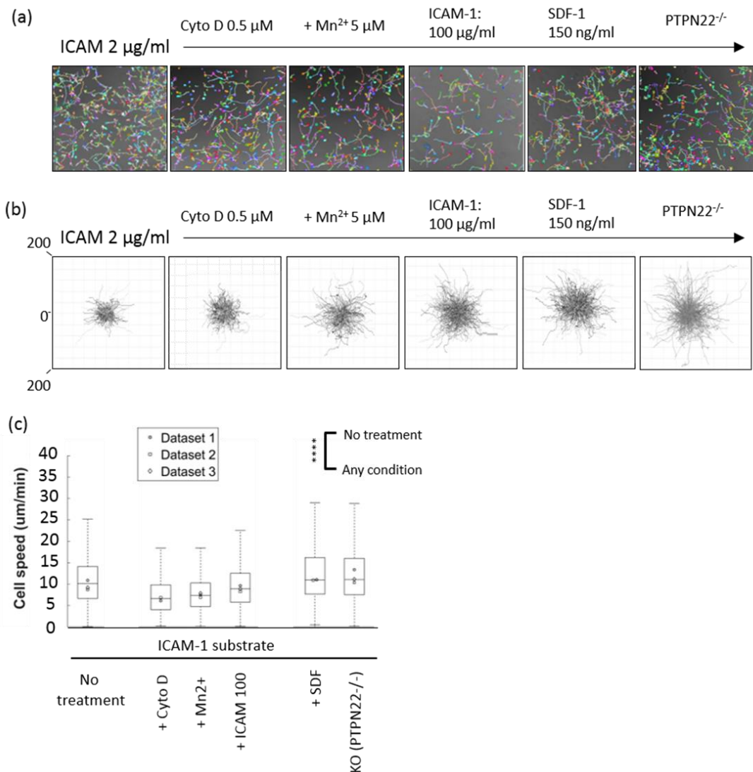
Figure 5-3: Cell speeds derived from automatic tracking for migrating cells using in STORM experiments. a) example tracked cells for each condition. b) example spider diagrams for each condition. c) box plot showing median cell speed under each condition with interquartile range. n = \sim 500 cells per condition from 3 mice. *** P < 0.00001 .
