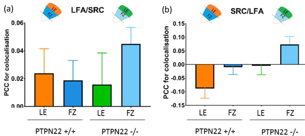
Figure 6-29: Pearson's correlation coefficient for clusters of LFA-1 colocalised with pY416 SRC, and clusters of pY416 SRC colocalised with clusters of LFA-1.
