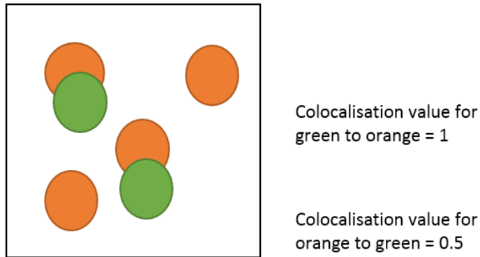
Figure 6-26: Explanation of asymmetric colocalization analysis.
