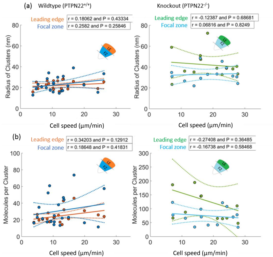
Figure 6-22: p397FAK cluster density is correlated with cell speed in PTPN22 +/+ cells, and not in PTPN22 -/- cells. Mean cluster metrics per cell were plotted against mean cell speed (dots). Linear regression (solid line with dotted confidence intervals) and Pearson's analysis provide an r value for each metric vs cell speed plot. This is done in PTPN22 +/+ cells (entire left column, orange and blue) and PTPN22 -/- KO cells (entire right column, green and light blue) for the radius of clusters (a) or the number of molecules per cluster (b). n = 21 PTPN22 +/+ and 14 KO cells from a mixed culture derived from 3 mice per condition.
