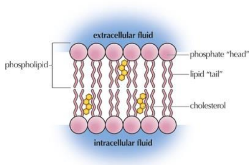
Figure 23 Structure of phospholipids bilayer. (Figure taken from reference 69 )
