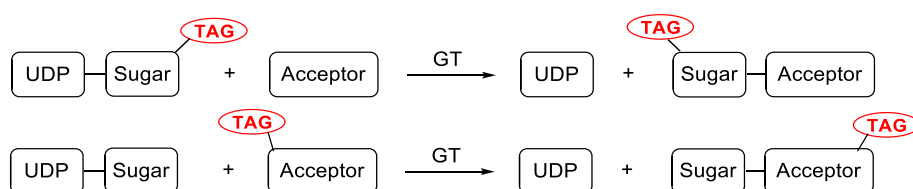
Figure 70 Non-natural substrate, like labelled donor or substrate: the enzyme activity can be determined depending on the product formation by spectrophotometric or fluorescent methods.
