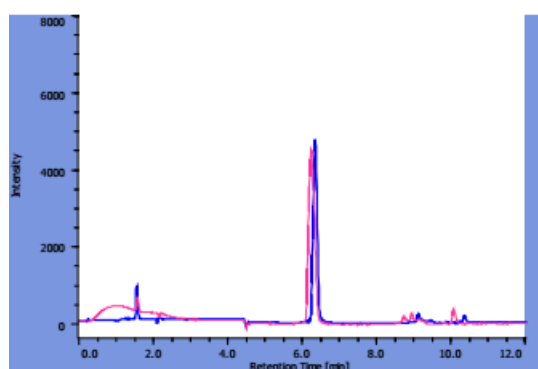
Figure 63 Chromatograms of sample of reaction solution (including 29 , H-1 and enzyme). Samples were removed from the solution in Eppendorf, followed by the addition of methanol. The mixtures were centrifuged for 15 min at 1000 rpm. The supernatants (100 \mu L) were then used for the HPLC analysis. The impurity signal appeared between t_R 1 to 3 min reduced greatly.
