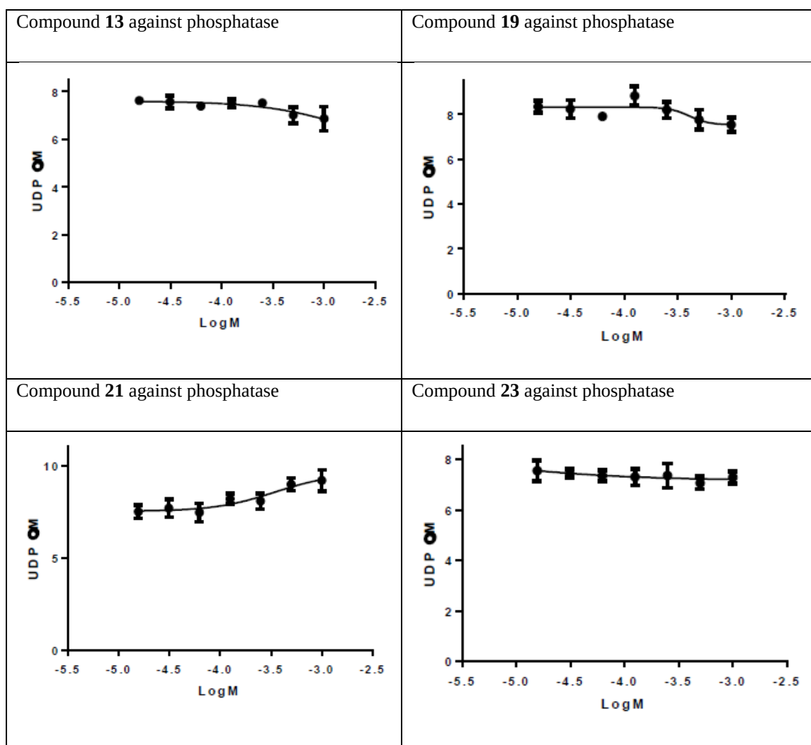
Figure 41 Control experiment of active nucleoside derivatives towards phosphatase Conditions: compound 13 , 19 , 21 or 23 (0 to 1mM), acceptor (GlcNAc, 5 mM), UDP-Gal donor (28 \mu M), \text{MnCl}_2 (5 mM), Chicken egg-white lysozyme (CEL, 1 mg/mL), calf-intestinal alkaline phosphatase (CIP, 10 U/mL), DMSO (10%), buffer (13 mM HEPES, pH = 7.0, 50 mM KCl) were incubated on a 96-well plate at 30 °C with shaking for 20 min. The reaction was stopped by the addition of malachite reagents, and the absorbance was recorded at 620 nm after 30 min. All concentrations are final concentrations. Bars indicate mean values \pm S.D. of triplicate experiments
