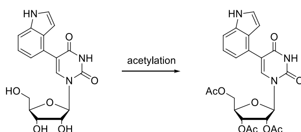
Scheme 8 Synthesis of acetylated 5-indole uridine. Reagents and conditions: acetic anhydride, 4-Dimethylaminopyridine (DMAP), pyridine, rt, 4h, 77%.
