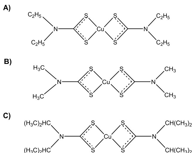
Figure 1.7: Structures of Cu-DTC complexes. A) copper (II) diethyldithiocarbamate (Cu-(DEDTC) 2 ); B) copper(II) dimethyldithiocarbamate (Cu-(DMDTC) 2 ); C) copper (II) diisopropyldithiocarbamate (Cu-(DPDTC) 2 ).
