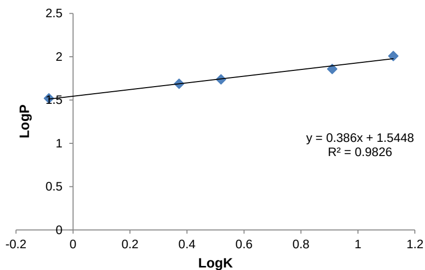
Figure 6.5: Correlation between the literature logP values of Cu(10) , Cu(11) , Cu(21) , Cu(22) and Cu(23) and their experimental logKs measured by HPLC. A C_{18} column was used as the stationary phase and a water + 0.1 % (v/v) TFA (60 %) / acetonitrile + 0.1 % (v/v) TFA (40 %) isocratic system as the mobile phase.
