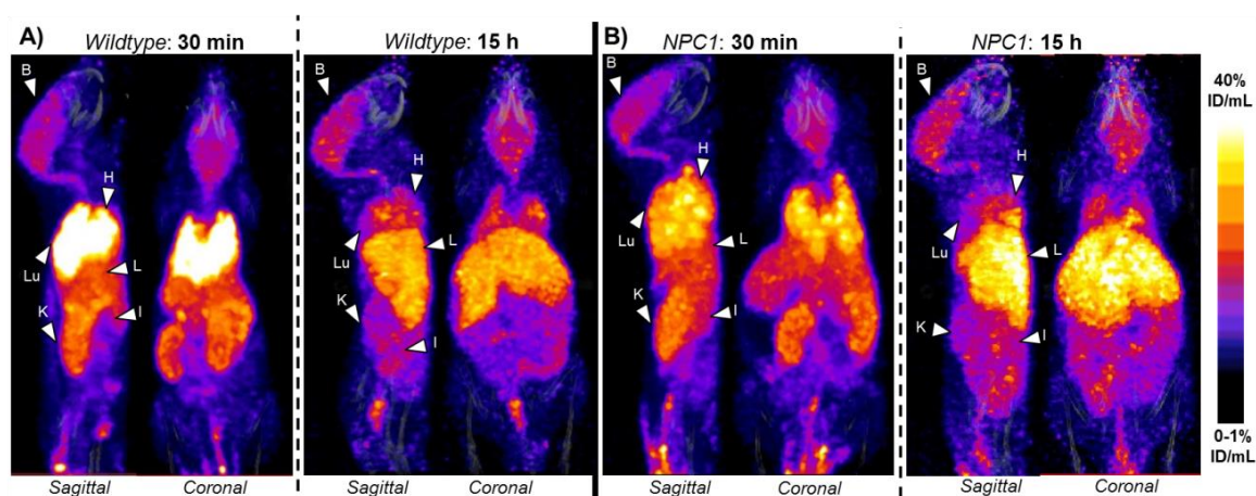
Figure 5.1: Exemplar sagittal and coronal views of PET/CT MIPs of 6-week-old female wildtype controls (A) and age-matched NPC1 ^{-/-} transgenic mice (B) at 30 min and 15 h post-injection of ^{64}\text{Cu} -GTSM. PET imaging revealed high accumulation of ^{64}\text{Cu} radioactivity in the heart, lungs, liver, kidneys, intestines and brain at 30 min after injection of the tracer in all mice. While ^{64}\text{Cu} accumulation decreased in the heart, lungs and kidneys over time, the concentration of radiocopper in the liver and intestines increased. Brain uptake of ^{64}\text{Cu} remained relatively constant over time in both animal groups. Organs are indicated by arrows: B = brain; Sp = spine; H = heart; Lu = lungs; L = liver; K = kidneys; I = intestines. All MIPs were scaled to 0-1 %ID/mL (min) and 40 %ID/mL (max).
