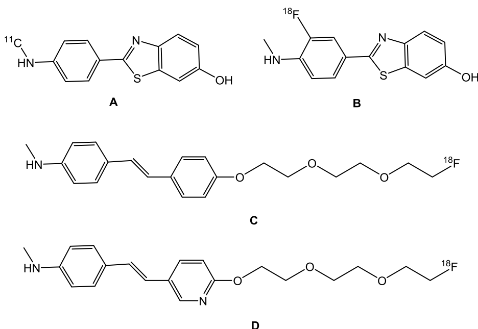
Figure 3.1: Chemical structures of ^{11}\text{C} -PIB (A), ^{18}\text{F} -Flutemetamol (B), ^{18}\text{F} -Florbetaben (C) and ^{18}\text{F} -Florbetapir (D).
