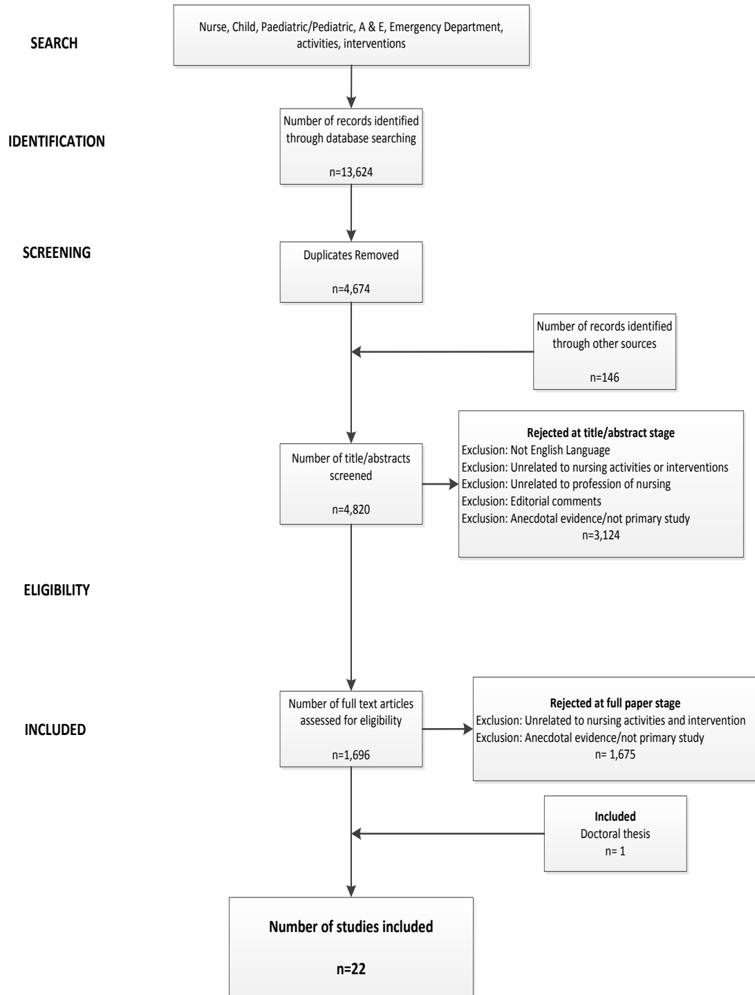
Figure 2.1 Search strategy
