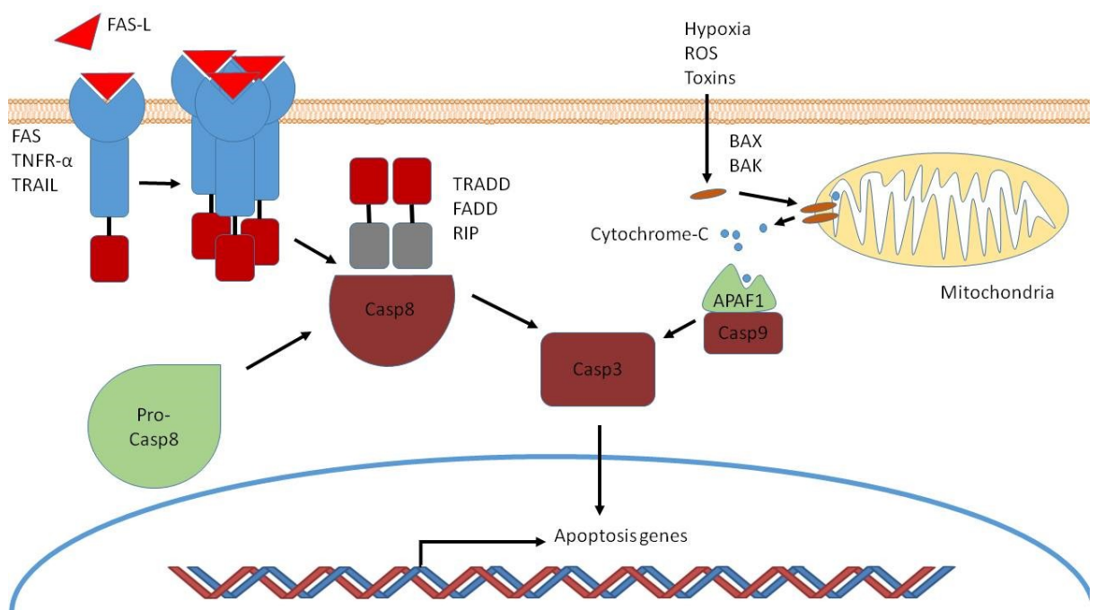
Figure 1.11 Apoptosis.
