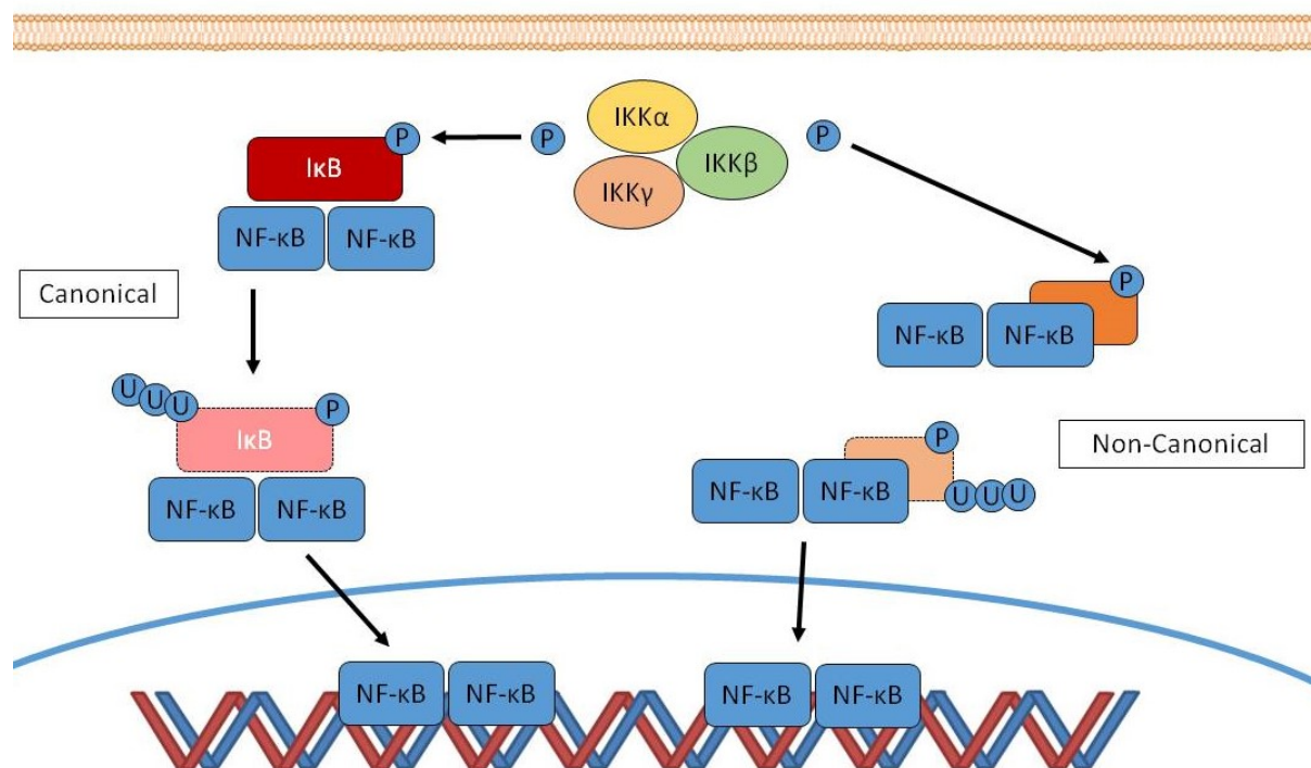
Figure 1.7 NF-κB pathway.
