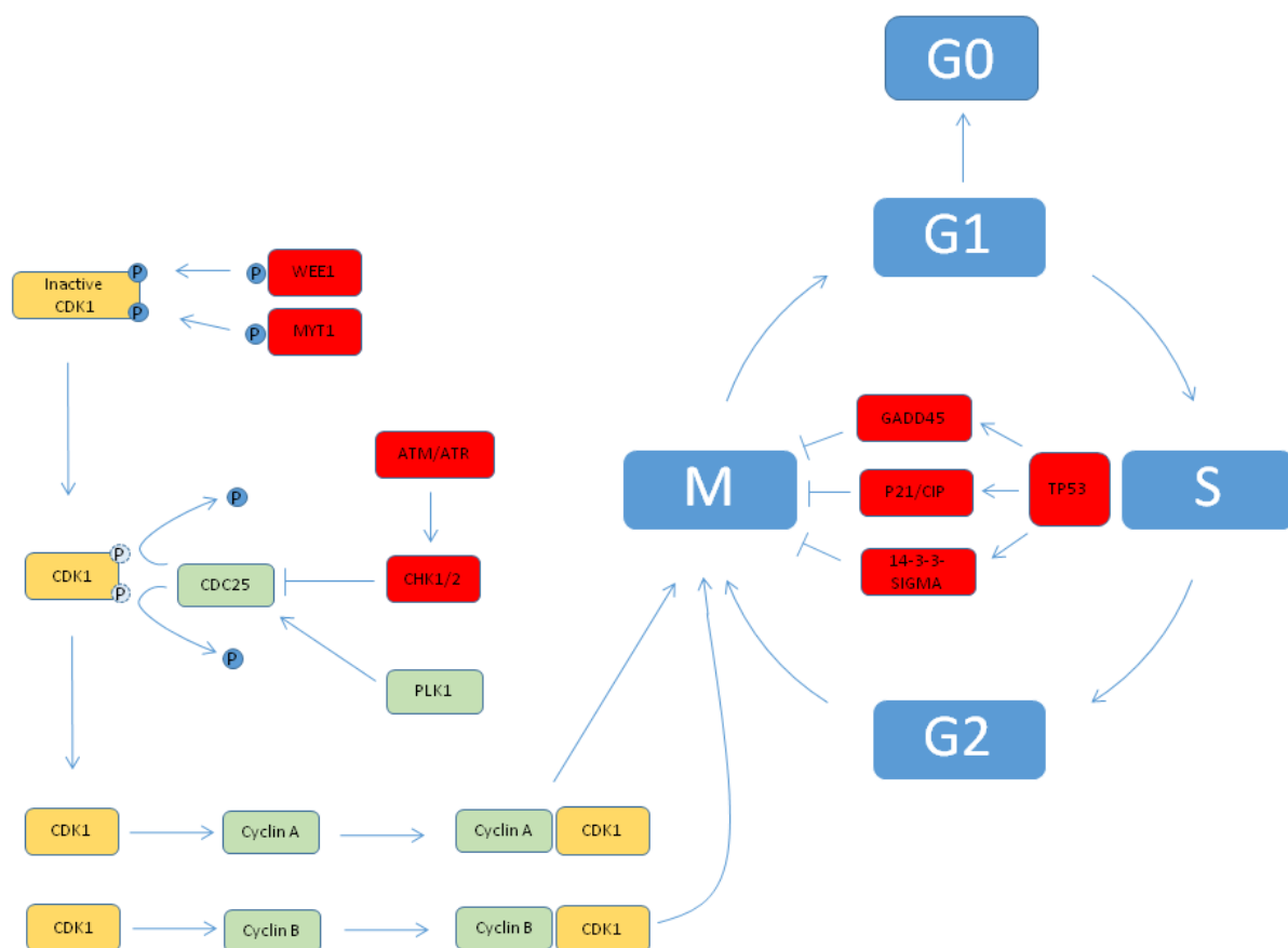
Figure 1.14 G2/M Regulation.
