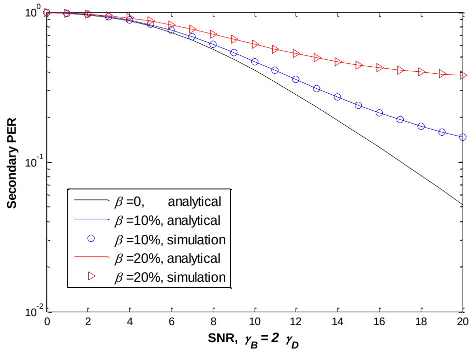
Fig. 3.15. Secondary PER vs. secondary SNR, unequal primary and secondary powers ( \bar{\gamma}_B = 2\bar{\gamma}_D ).
