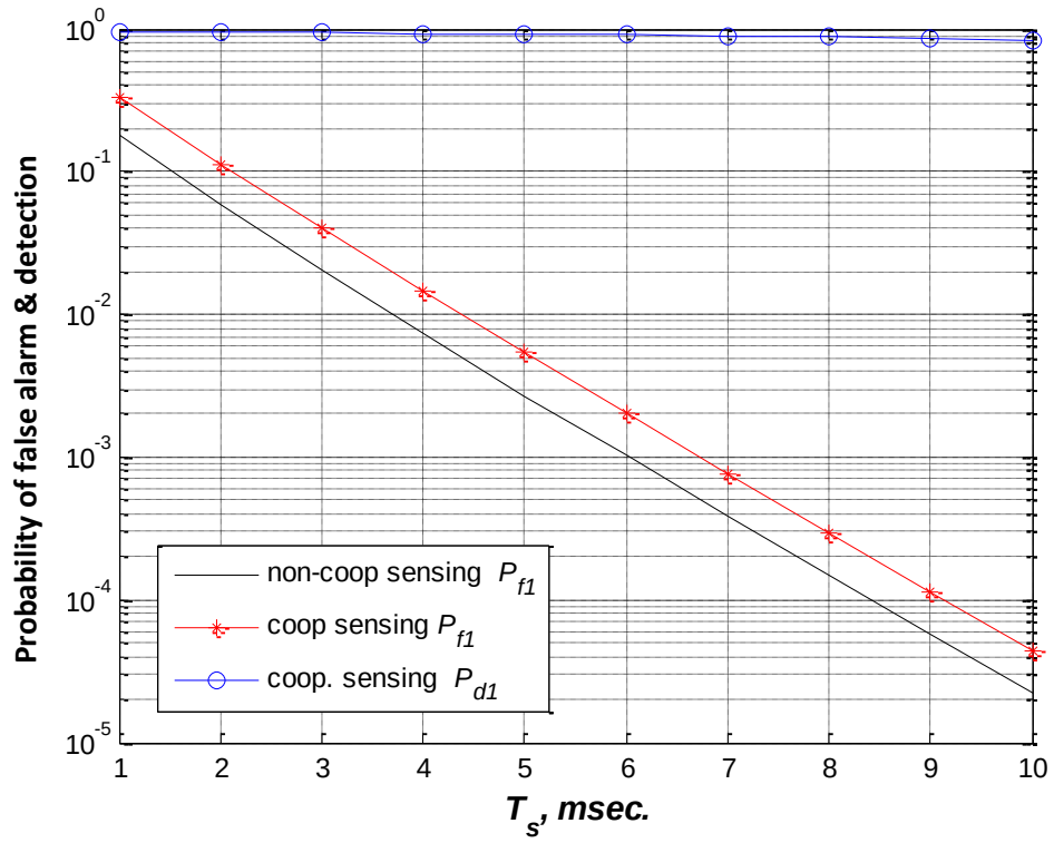
Fig. 4.7. Probability of false alarm ( P_{f1} ) and detection ( P_{d1} ) vs. sensing time duration T_s for cooperative and non-cooperative modes.
