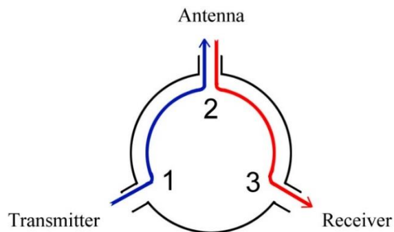
Figure 2.3. RF circulators used in shared antenna systems, like radars.
