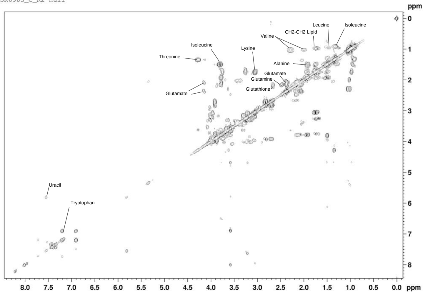
Figure 7.3. Representative 2D COSY ^1\text{H} HR-MAS NMR spectra of ROCK2 KO murine melanomas. A partial assignment is shown of identified metabolites. the spectrum was obtained on a 400 MHz Bruker spectrometer.
