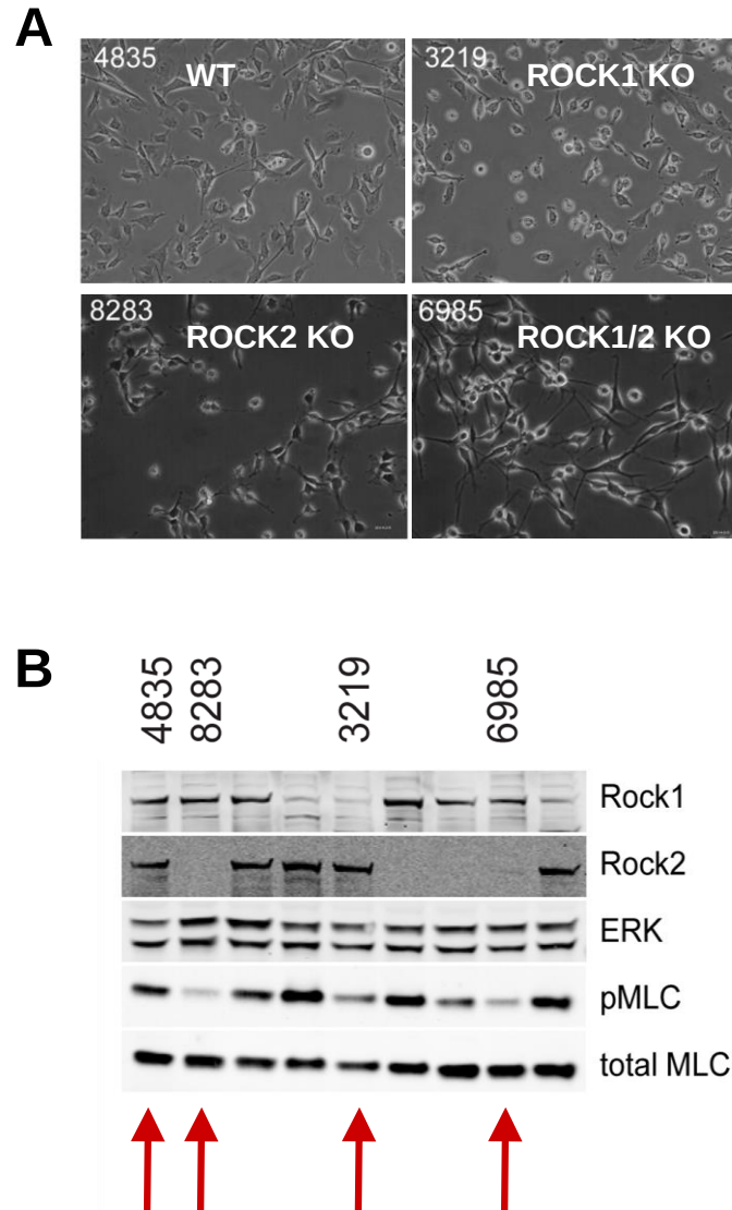
Figure 4.4. Cultured murine melanoma cells of with ROCK knocked out (KO) show a more elongated phenotype compared to wild type cells. A) Light microscopy images of wild-type, ROCK1 KO, ROCK2 KO and double KO melanoma cells. B) Western blot confirming KO and lowered levels of p-MLC compared to total-MLC. As double ROCK KO mice did not develop melanomas, the other isoform was knocked down in vitro for our studies. Figures provided by Dr. Sandra Kuemper.
