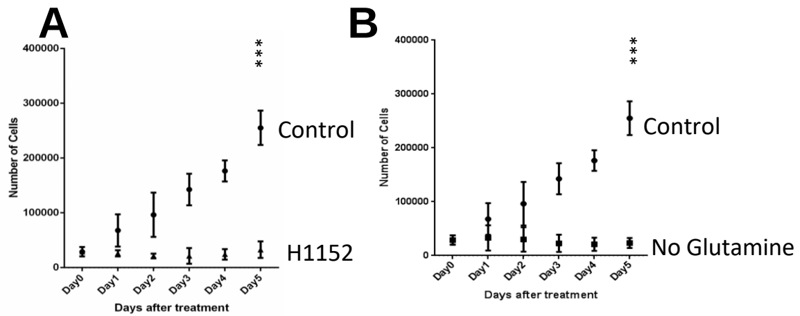
Figure 4.24. ROCK and exogenous glutamine are required for A375M2 melanoma proliferation in vitro . A) A375M2 cells treated every 24 hours with 5 \mu M H1152 over 5 days show near complete termination of proliferation. B) Cells cultured in glutamine free media also completely halt proliferation. experiments done in triplicate. data points are mean cell number and error bars represent Standard error of the mean. Student's t-test, *** p < 0.001 . Experiments are n=3 .
