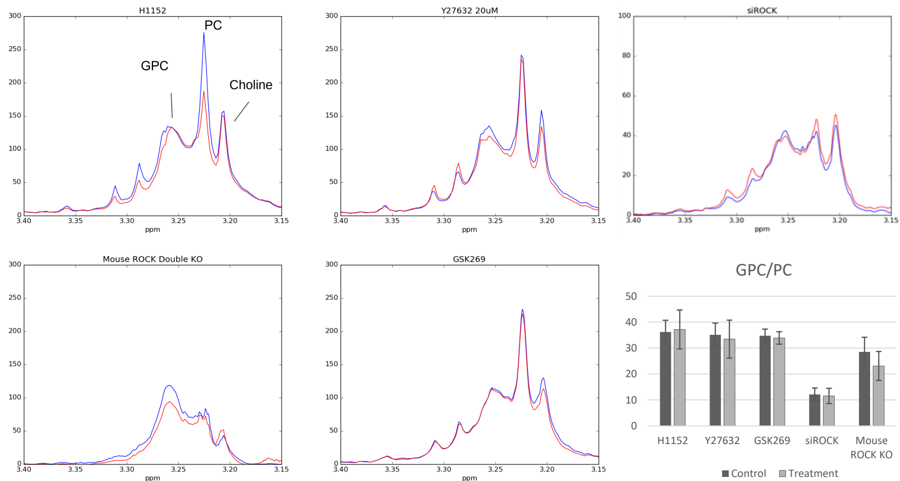
Figure 7.6 GPC/PC ratio of mouse melanoma cells decrease after KO of ROCK. Left) Mean PQN normalised ^1\text{H} HR-MAS NMR spectra of melanoma cells where ROCK activity has been interfered with. Control spectra are plotted in blue while treatment spectra re plotted in red. Spectra highlight the changes in choline, Phosphocholine (PC), and glycerophosphocholine (GPC). Right) The ratios between GPC and PC are shown between control cells and treatment cells. All experiments are n=3 with 3 internal replicates per experiment.
