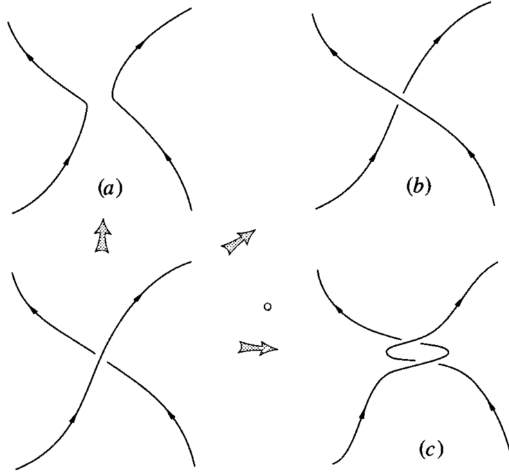
Figure 2.1: Three possible outcomes when strings intersect: (a) reconnect by exchanging legs, (b) passively pass through each other or (c) entangle. From [41, Figure 6.4].
