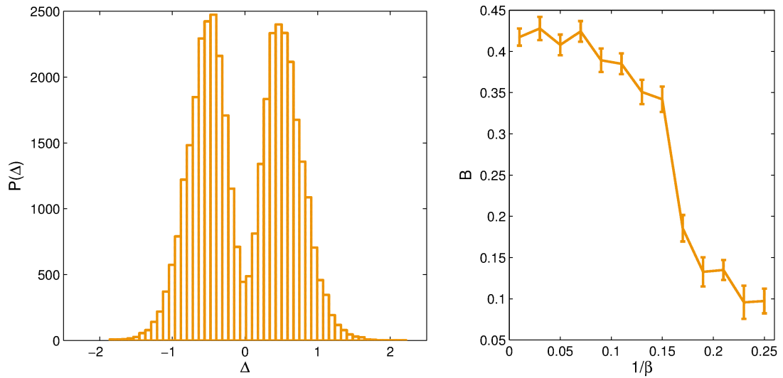
FIGURE 4.9: Segregation of informed traders in the Toth model. Left: Steady state distribution of informed traders with the forgetting rate r = 0.05 and intensity of choice \beta = 20 . Right: Binder cumulant of the steady state distribution for different values of intensity of choice \beta while r = 0.05 . The population consists of 400 traders of each information level L = 0 to L = 4 . We do not note different steady states of the subpopulations with different information levels that is why the overall attraction distribution is shown.
