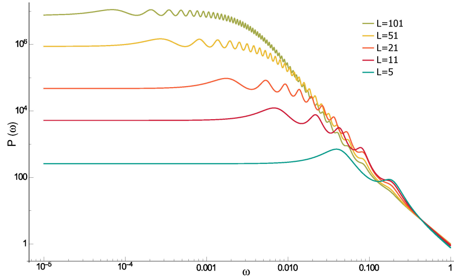
FIGURE 5.6: Power Spectra in 3-player APA game with variable number of strategies. The number of resonant frequencies (peaks in the power spectra) increases with number of available strategies, but the amplitude of some nose induced cycles decays with L , note specially amplitudes of the peaks at the largest \omega .
