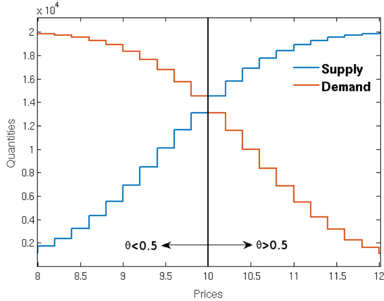
FIGURE 2.2: Illustration of the market mechanism - equilibrium trading price. The demand and supply curves, showing the number of orders to buy above (resp. sell below) a certain price. The vertical black line marks the equilibrium trading price, i.e. the price at which demand equals supply, while the arrows show how the trading price changes with \theta .
