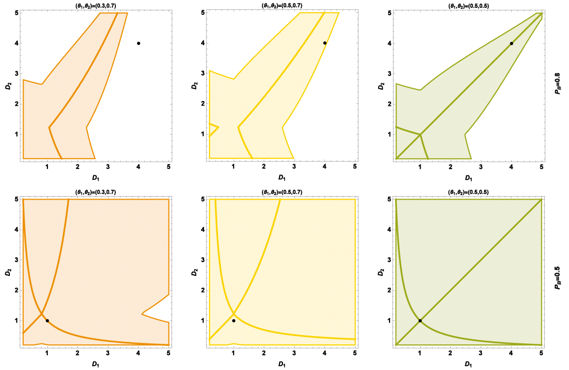
FIGURE 3.8: Single population steady state types in the space of market order parameters (D_1, D_2) . Top: population of buyers ( p_B = 0.8 ); Bottom: "indecisive" population ( p_B = 0.5 ); Left: symmetrically biased markets (\theta_1, \theta_2) = (0.3, 0.7) ; Middle: a fair and a biased market (\theta_1, \theta_2) = (0.5, 0.7) ; Right: two fair markets (\theta_1, \theta_2) = (0.5, 0.5) . Coloured regions represent domain of weakly segregated states in the r \rightarrow 0 limit. Their subsets, domains of strongly segregated states are represented with solid lines. White regions represent order parameters for which steady states are unsegregated.
