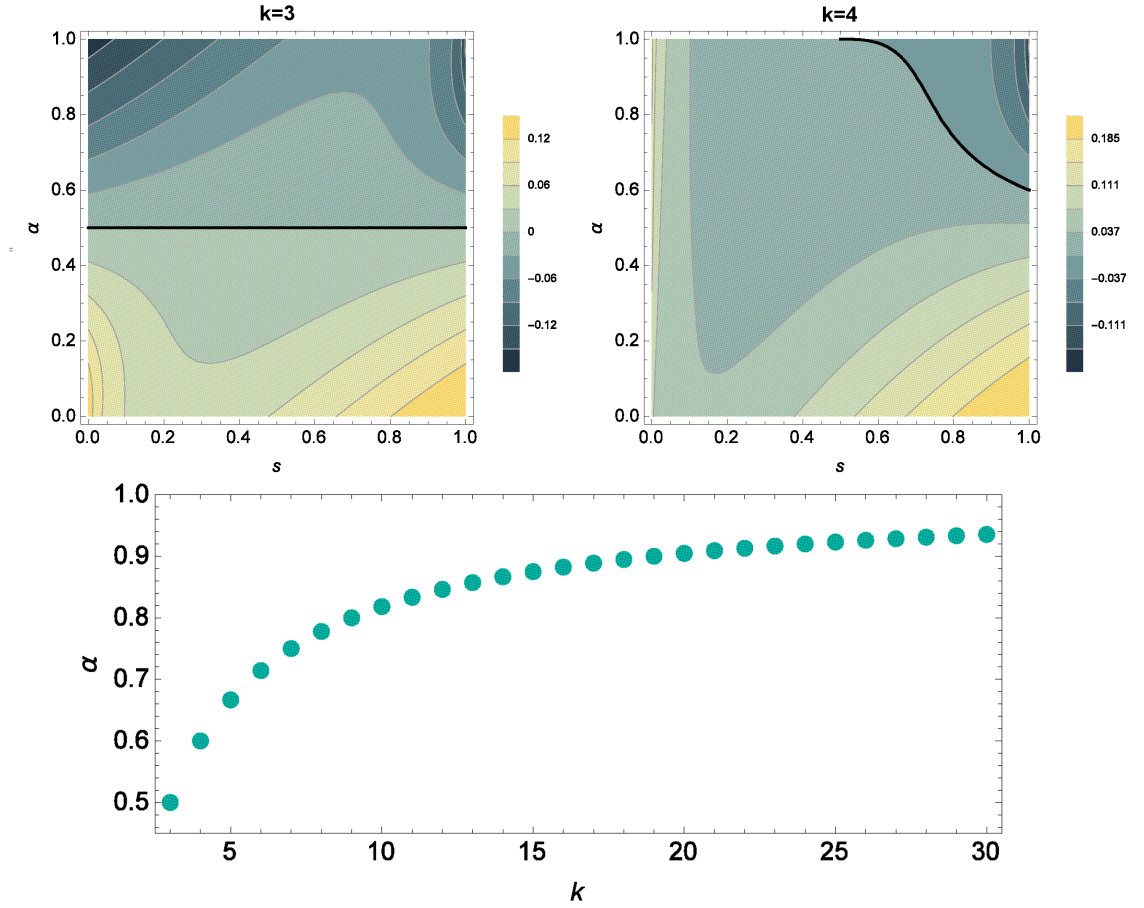
FIGURE G.1: Existence of the Evolutionary Stable Strategy. Top panels show contours of the f(s, \alpha, k) for k = 3 (left) and k = 4 (right) demonstrating that the sign of the function becomes negative for some s \in [0, V] when \alpha = 0.5 for k = 3 and \alpha = 0.6 for k = 4 , marking the inexistence of ESS for \alpha greater than those values. (Black line in both contour plots marks f(s, \alpha, k) = 0 contour.) Bottom panel shows \alpha_c dependence on k , for \alpha < \alpha_c there exist unique evolutionary stable strategy.
