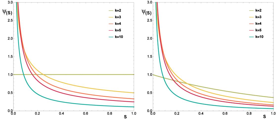
FIGURE 5.1: Fixed point mixed strategy distributions of evolutionary auction games with different number of players k . Left: all-pay biological auctions (APA); Right: Second-price all-pay biological auctions (SAPA). The reward value is V = 1 , note domain of APA games is [0, V] , while the strategy domain of SAPA games is [0, \infty) , only the [0, V] interval is shown for comparison with APA games.
