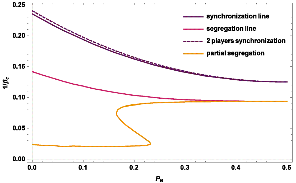
FIGURE 3.5: Four traders phase diagram when the group buy/sell roles are probabilistic. We note that both the segregation (purple line) and the synchronization (dark violet line) region shrink when the difference in agent's buy/sell preferences decreases, the trend we have observed in the two player system as well (dashed line). Below the orange line "partially" segregated fixed points exist too - one of the four agents have a preference for the opposite market.
