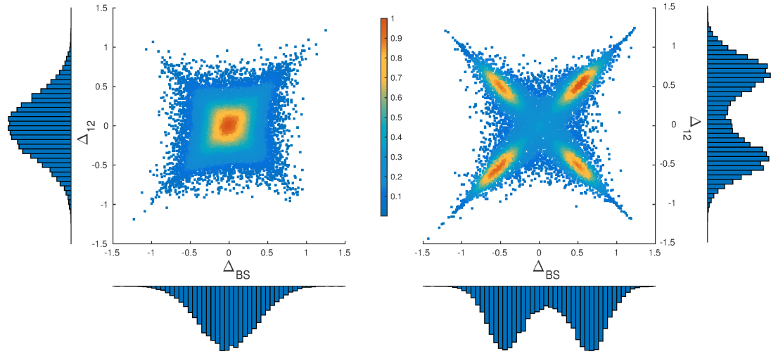
FIGURE 2.3: Steady states in numerical simulations. Steady state distributions of attractions for buying vs selling and for market 1 vs 2, respectively, for forgetting rate r = 0.1 . For low enough intensity of choice (left, \beta = 3.45 ), an unsegregated steady state arises, while higher \beta (right, \beta = 7.14 ) causes traders to segregate into four discernible groups. The histograms along the axes show the marginal distributions of \Delta_{BS} and \Delta_{12} , respectively. From the marginals we note that in the segregated state roughly half of the population specialize in buying (similarly half prefers market 1), although the fractions of buyers (sellers) at different markets are not the same. The data shown are taken from 100 trading periods of 100 independent runs (for more details on numerical simulations and system parameters, see D ). The colour scale in the central scatter plots shows the probability density of agents [83] .
