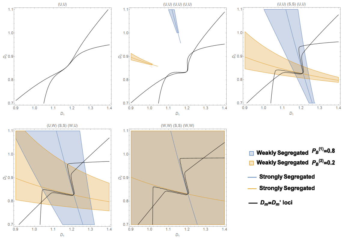
FIGURE 3.9: Steady states of the decisive population – (p_B^{(1)}, p_B^{(2)}) = (0.8, 0.2) – for different \beta in the r \rightarrow 0 limit. Top Row: Left - 1/\beta = 0.31 (U,U) solution; Middle - 1/\beta = 0.29 three (U,U) solutions; Right - 1/\beta = 0.265 (U,U), (S,S), (U,U) solutions. Bottom Row: Left 1/\beta = 0.245 , (U,W), (S,S), (W,U); Right 1/\beta = 0.2 , (W,W), (S,S), (W,W). U - unsegregated; W - weakly segregated; S - strongly segregated steady state.
