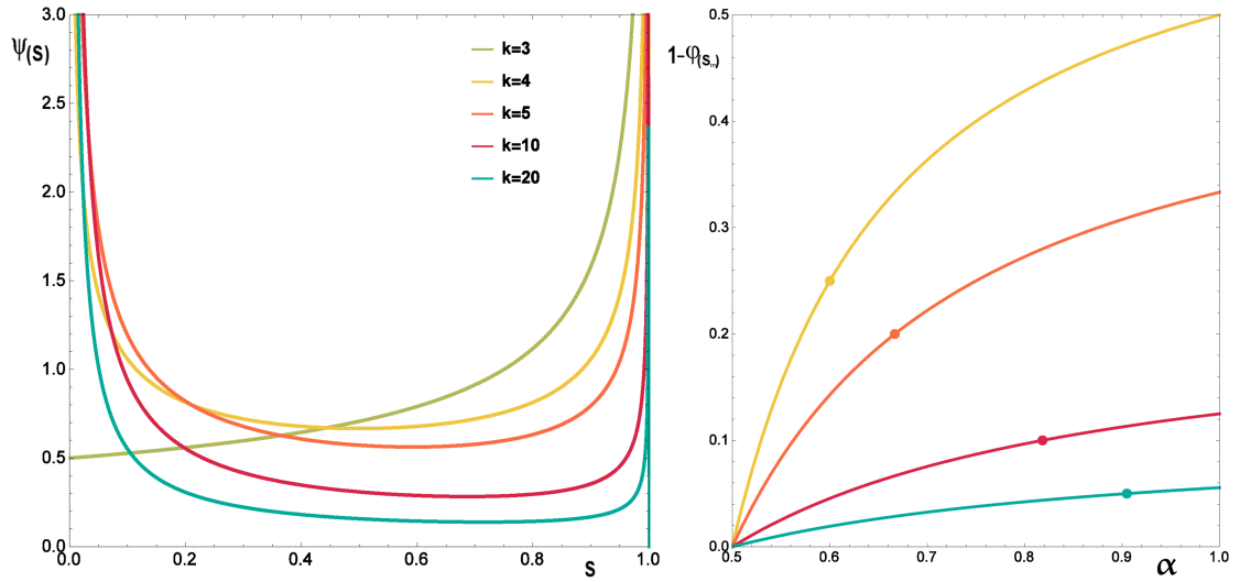
FIGURE 5.2: Fixed point distributions for the APA evolutionary game with two rewards and variable number of players k . Left: Fixed point distributions for \alpha = 1 ; Right: Fraction of players at the high bidding peak as function of reward ratio \alpha . Circles in the right panel show \alpha_c above which the bimodal fixed point distribution is not an evolutionary stable strategy.
