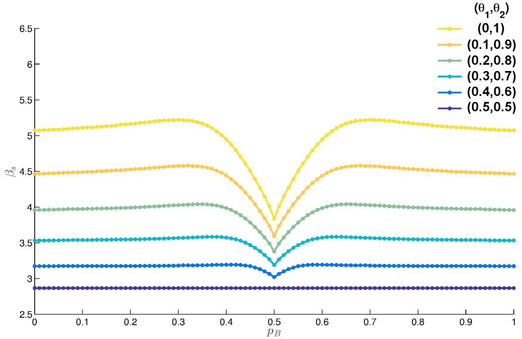
FIGURE 2.10: Segregation thresholds for different symmetric agent types, at different markets. Segregation threshold as a function of the first agent type's preference for buying p_B^{(1)} = p_B , assuming the other agent type has the opposite preference p_B^{(2)} = 1 - p_B . Different sets of symmetric market parameters are compared; non-trivially, the region of segregation is largest when both markets are fair.
