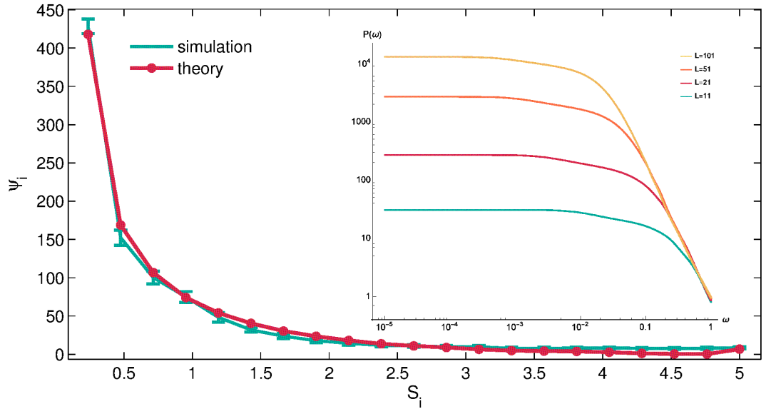
FIGURE 5.13: 3-player SAPA auction with discrete strategies from the [0, 5V] domain. Fixed point distribution of the 3 player SAPA game as predicted by the replicator equations in the discrete strategy space with L = 21 and as obtained by numerically simulated evolution of 1000 agents. The insert shows power spectra for different number of available strategies for the same 3-player SAPA game on [0, 5V] domain.
