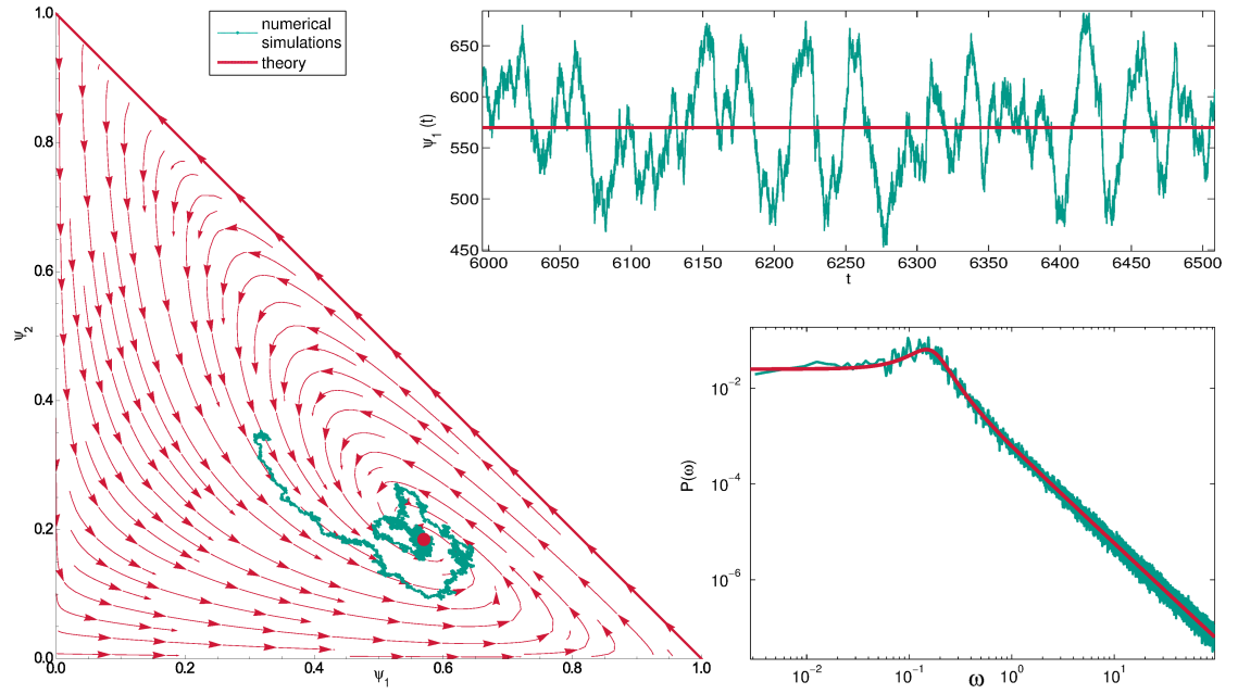
FIGURE 5.3: 3-player All-Pay Auction with 3 available strategies. Bottom left: Phase portrait of the corresponding replicator equations (pink) with a single realisation of the simulated birth-death process of N = 1000 players (cyan). Top: Time series of the number of players playing S_1 , we note noisy oscillations around the fixed point of the deterministic limit, pink line correspond to the fixed point present in the Bottom left panel. Bottom right: Power spectra of the numerically simulated system (cyan) and analytical prediction (pink), both showing a resonant frequency \omega_r \approx 0.145 corresponding to the oscillations of a period \approx 43 generations.
