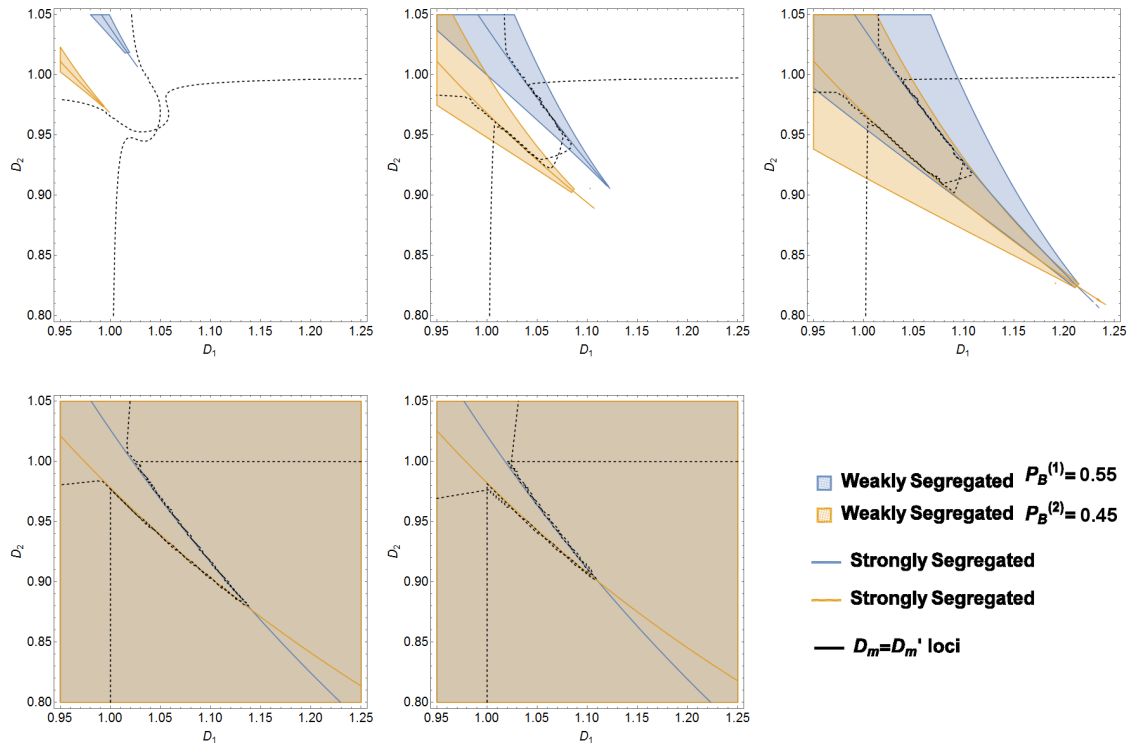
FIGURE 3.10: Steady state of the indecisive traders (p_B^{(1)}, p_B^{(2)}) = (0.55, 0.45) for different intensities of choice \beta in the large memory limit ( r \rightarrow 0 ). Top row: Left 1/\beta = 0.31 the unsegregated state; Middle 1/\beta = 0.295 unsegregated ( U, U ) and four partially segregated states ( U, S ); Right 1/\beta = 0.28 weakly segregated ( W, W ) and four partially segregated states ( W, S ). Bottom row: Left 1/\beta = 0.1 strongly segregated ( S, S ) and two partially segregated states ( W, S ); Right: 1/\beta = 0.05 strongly segregated ( S, S ) and two weakly segregated states ( W, W ). U - unsegregated; W - weakly segregated; S - strongly segregated steady state.
