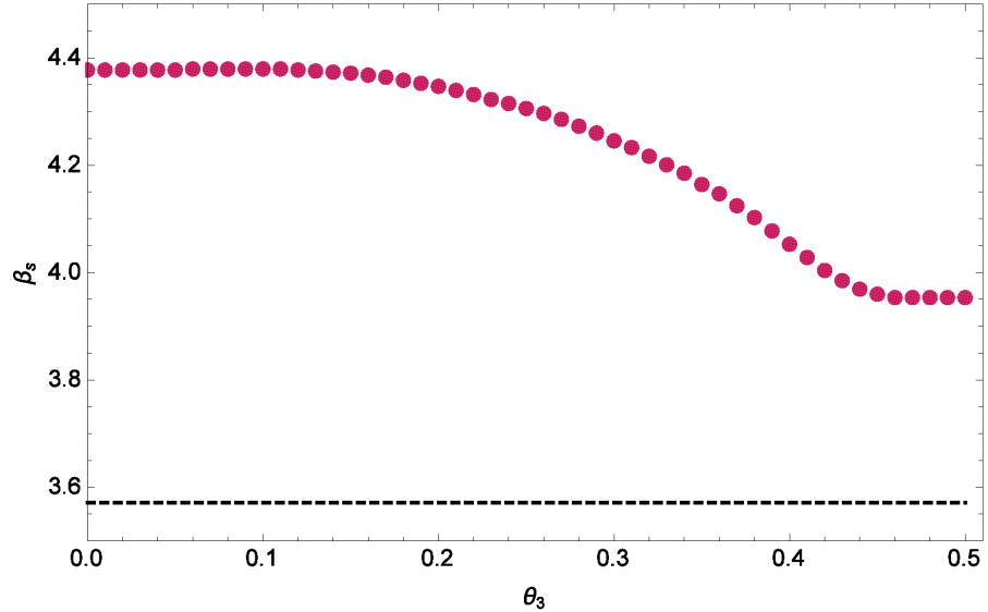
FIGURE 4.4: Segregation threshold \beta_s as a function of the third market bias , where other parameters are those of a typically studied system (p_B^{(1)}, p_B^{(2)}, \theta_1, \theta_2) = (0.2, 0.8, 0.3, 0.7) . The dashed black line shows segregation threshold of the two market system.
