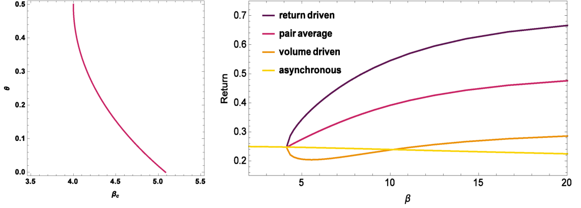
FIGURE 3.2: 2 players (\theta, \beta) phase diagram and returns. Left: Critical \beta as a function of symmetric market bias \theta . Right: Returns for different \beta for market bias \theta = 0.3 . At the critical ( \beta_s = 4.16 ), the return average of the pair is better than staying at the continuation of low \beta fixed point, but one of the agents needs to settle for less.
