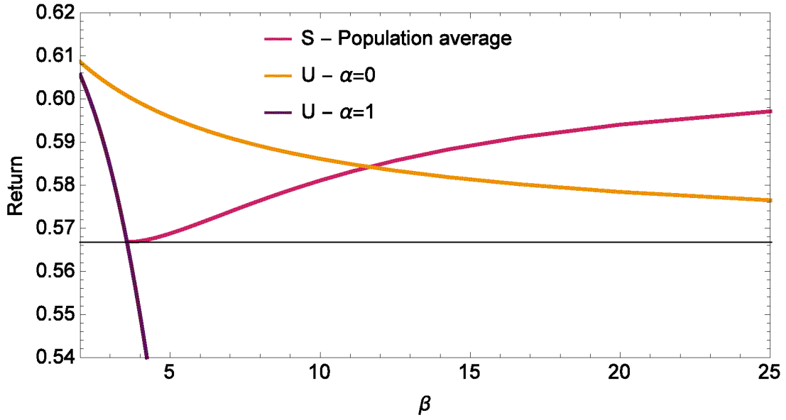
FIGURE 4.3: Return of the unsegregated state \alpha = 0 against intensity of choice \beta . We show average population return of the population consisting of decisive traders (p_B^{(1)}, p_B^{(2)}) = (0.8, 0.2) who don't forget attractions of unplayed actions ( \alpha = 0 ). We compare these returns against typically studied \alpha = 1 strongly segregated state and low \beta unsegregated state.
