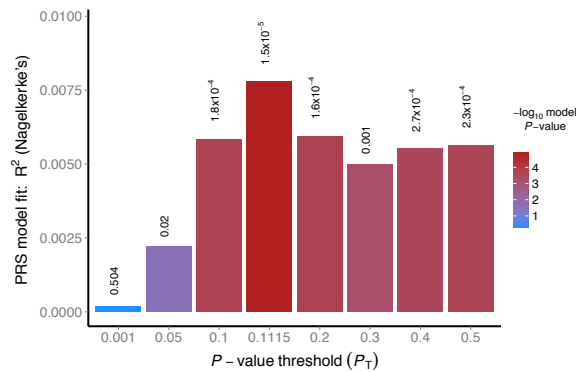
Figure S1a: ‘Ever smoked’: PRS using GWAS from the Tobacco and Genetics (TAG) consortium for ‘ever smoked’ as base phenotype data ( N = 74053 ), and the RADIANT-UK MDD data as target phenotype data. SNPs in linkage equilibrium, adjusting for population structure using two principal components, show substantial evidence for shared genetic aetiology between smoking and MDD.
