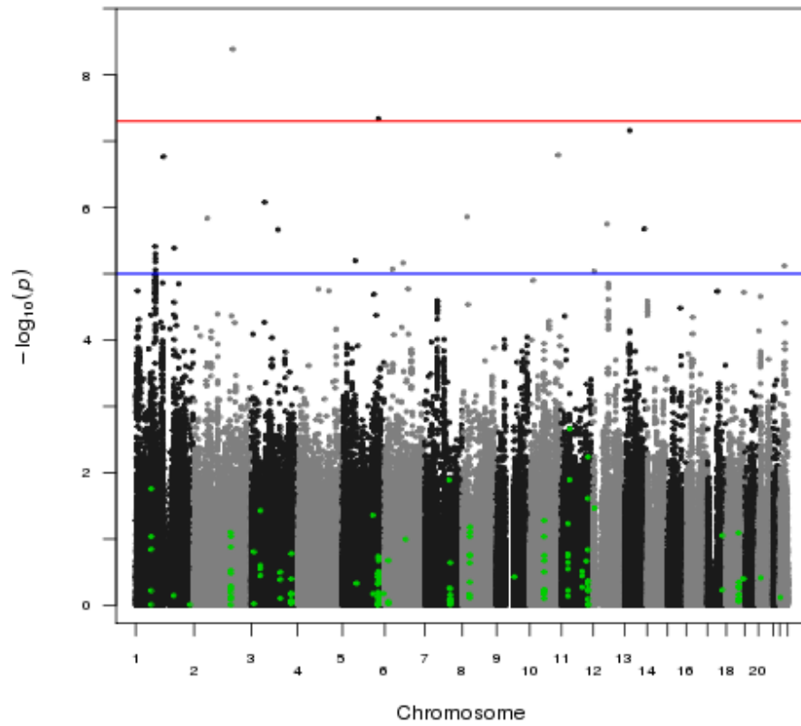
Figure S6: Manhattan plot of imputed SNPs in RA case-control analysis. GPRS542 SNPs and their proxies are highlighted in green.
