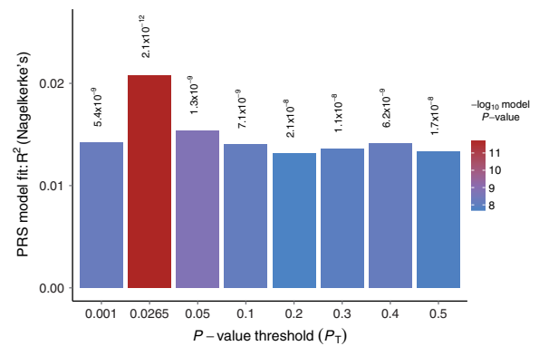
Fig. 1. Bar plot from PRSize showing results at broad P -value thresholds for Schizophrenia PRS predicting MDD status. A bar for the best-fit PRS from the high-resolution run is also included
