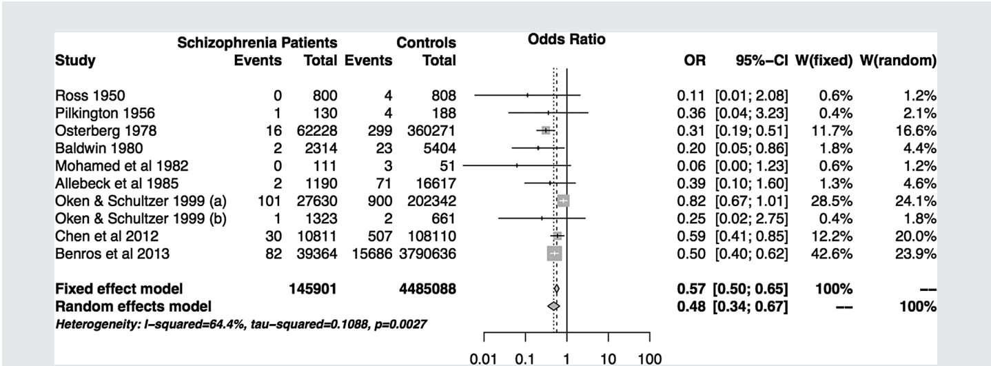
FIG. 1. Meta-analysis results. We identified 10 studies reported in 9 papers. Oken & Schultzer (a) compares schizophrenia vs other psychiatric patients in Canada meanwhile Oken & Schultzer (b) compares a similar sample in New York State. We present the RA prevalence (events) in SCZ cases vs controls across studies. W: weight for each study under random and fixed effects analysis.
