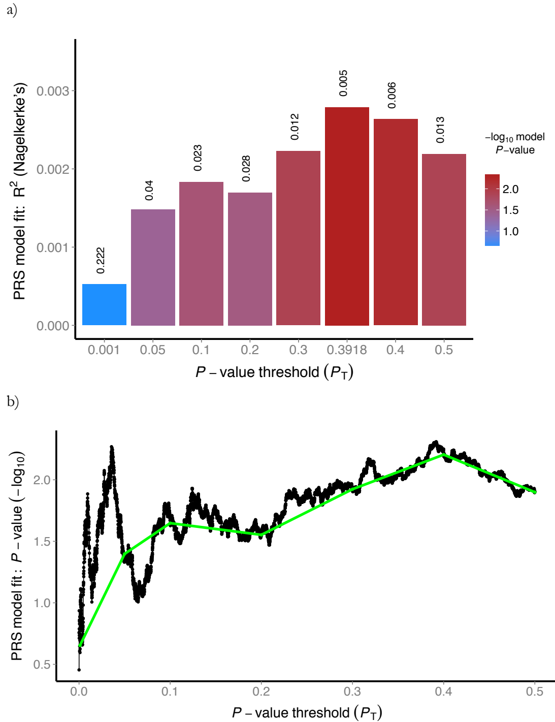
Figure A1: PRS for Schizophrenia predicting rheumatoid arthritis case-control status across thresholds. Results using high-resolution scoring are presented (a) as a bar chart and (b) as a point-plot with the results of PRS at a limited number of thresholds superimposed in green to demonstrate the increased resolution allowed by PRSice .
