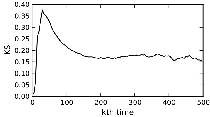
Figure 4.5 Kolmogorov-Smirnov Statistic for Action Times
