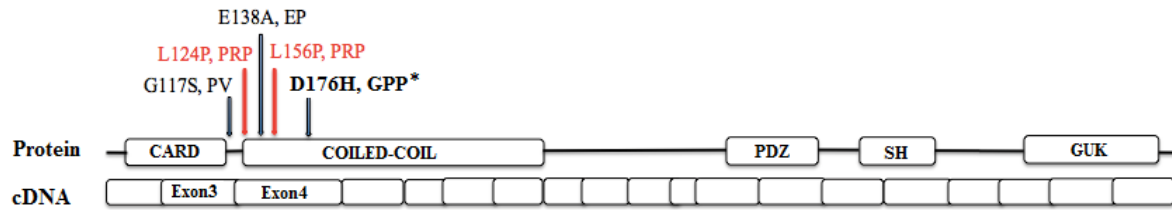
Figure 4.1. Localisation of the main CARD14 mutations in the protein and cDNA sequence
