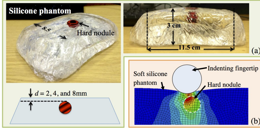
Fig. 3.1 (a) A soft silicone phantom fabricated using soft clear silicone elastomer gel with a spherical plastic bead of size 15 mm diameter embedded inside at the depth of d = 2, 4 , and 8 mm. (b) Example of the finite element simulation of soft silicone phantom with an embedded hard nodule being palpated using a an indenting fingertip [132].
