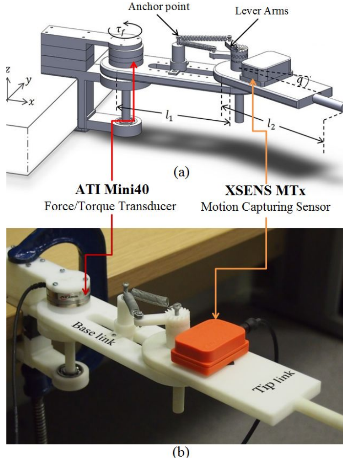
Fig. 5.1 (a) a design of two-links planar manipulator with a variable stiffness joint (VSJ). The rotational displacement of the tip link, q , is recorded using an XSENS MTx Motion Capturing sensor; whereas the torque experienced at the base of the manipulator during such movement is measured by ATI Mini40 6-axis Force/Torque Transducer, (b) a photo of the experimental platform attached on the table with a clamp.
