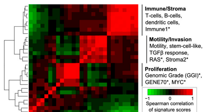
Figure 6. Intertumour heterogeneity of gene expression profiles associated with cellular processes and disease progression. Unsupervised hierarchical clustering showing pair-wise correlations of a panel of gene signature scores across primary breast tumour tissue samples (234 patients). Representative signatures are indicated for each cluster: T-cells, B-cells and dendritic cells, Immune1*, Motility, stem-cell-like, tumour growth factor \beta (TGF \beta ) response, RAS*, Stroma2*, GGI*, Gene70*, MYC* (*signature curated by Ignatiadis et al. 112 ). Recent studies report expression-based prognostic and predictive stratification of primary breast tumours, which are phenotypically similar according to current clinical methods. 111,113,114 Images should be viewed in the online format.
