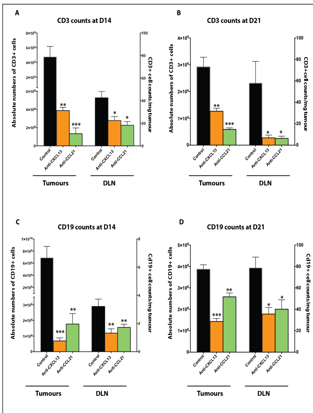
Figure 5-7: Effect on T-/B-cell recruitment following in vivo chemokine (CXCL13/CCL21) neutralization within the 4T1.2 tumour model.
