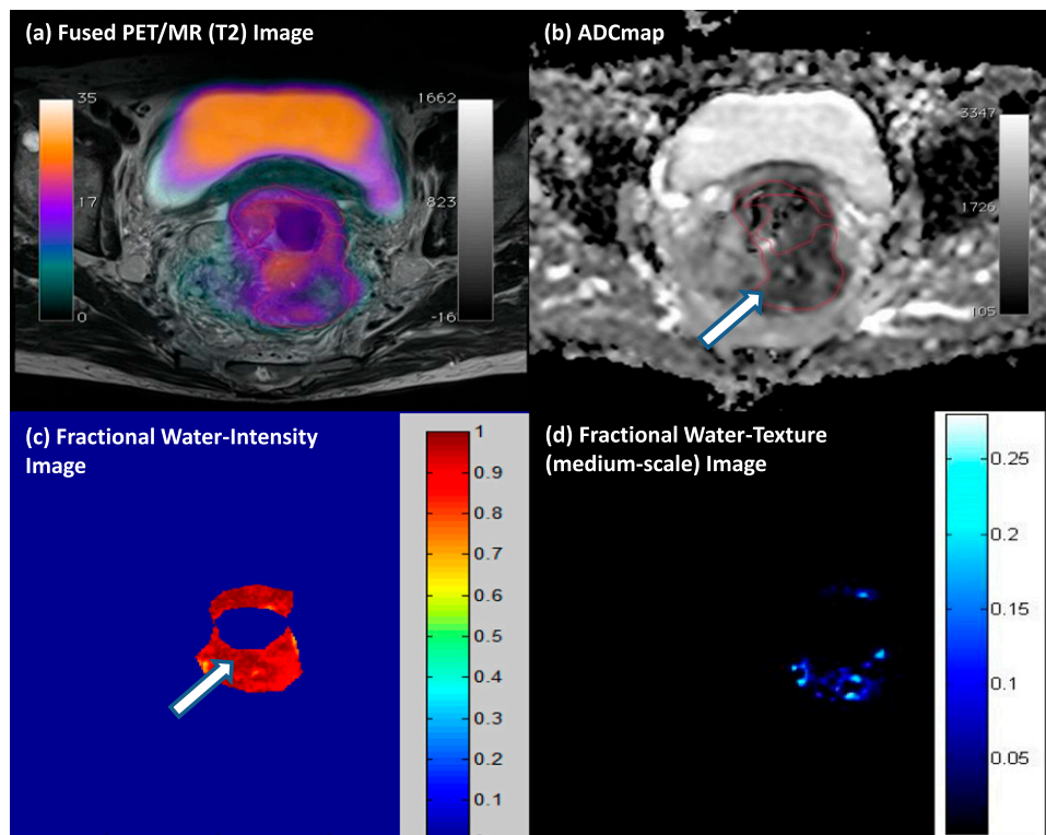
Figure 5. Multiparametric positron emission tomography (PET)/MRI of a rectal cancer. (a) High ^{18}\text{F} -fluorodeoxyglucose uptake on fused PET/ T_2 MRI, with (b) a correspondingly patchy reduced apparent diffusion coefficient (ADC) in keeping with pockets of high cellularity within the tumour and (c) a fractional water image derived from source fat and water Dixon images of the same tumour confirms that areas of increased cellularity correlate with relatively increased water content (white arrows). (d) Application of a medium coarse textural filter highlights 3- to 4-mm bright objects on the fractional water image (medium texture map). Images should be viewed in the online format. ( www.texrad.com , Radstock, UK.)
