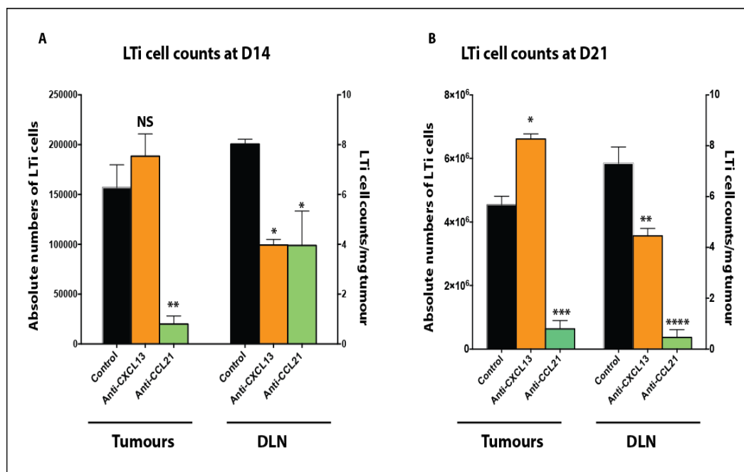
Figure 5-6: Effect on LT \alpha i recruitment following chemokine (CXCL13/CCL21) neutralization within the 4T1.2 tumour model in vivo.
