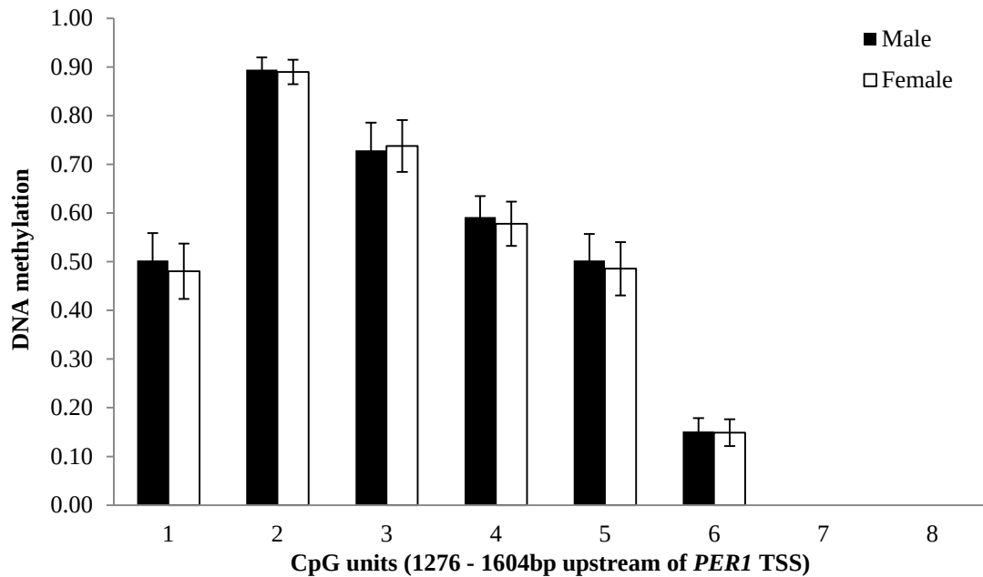
Figure 4-6 DNA methylation in PER1 upstream (Mean \pm SD). The DNA methylation of 8 CpG units located 1276-1604bp upstream of PER1 TSS was analysed by the Sequenom® MALDI-TOF mass spectrometry (N = 330 in male, N = 355 in female). DNA methylation at CpG units 7 and 8 were not detectable.
