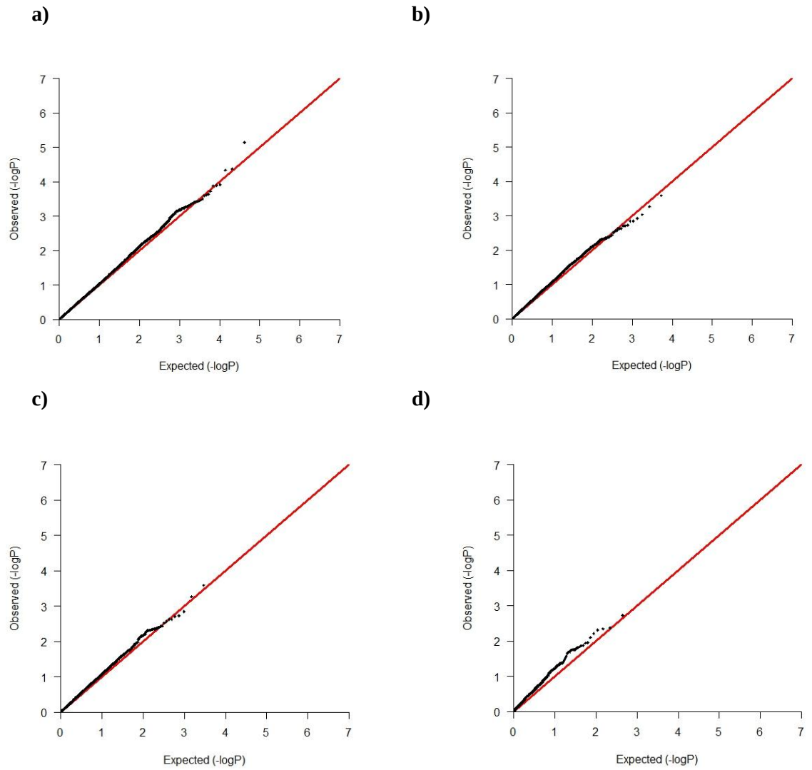
Figure 5-7 Q-Q p -value plots of genetic associations of past 12 month alcohol use in 16-year- old adolescents with a) stress genes; b) circadian genes; c) overlap stress x circadian genes; and d) neurotransmitter stress x circadian genes. \lambda = 1.05 in the stress gene list; \lambda = 1.16 in the circadian gene list; \lambda = 1.15 in the overlap stress x circadian gene list; \lambda = 1.3 in the neurotransmitter stress x circadian gene list. All red lines indicate x = y .
