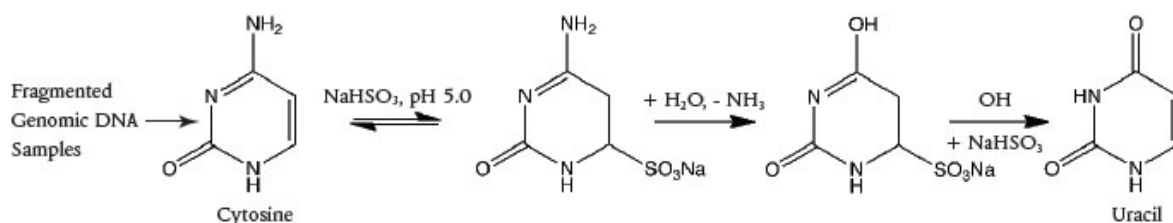
Figure 4-1 Mechanism for sodium bisulfite conversion. Cytosine is susceptible to sodium bisulfite conversion into uracil whereas 5'-methylcytosine remains non-reactive.
