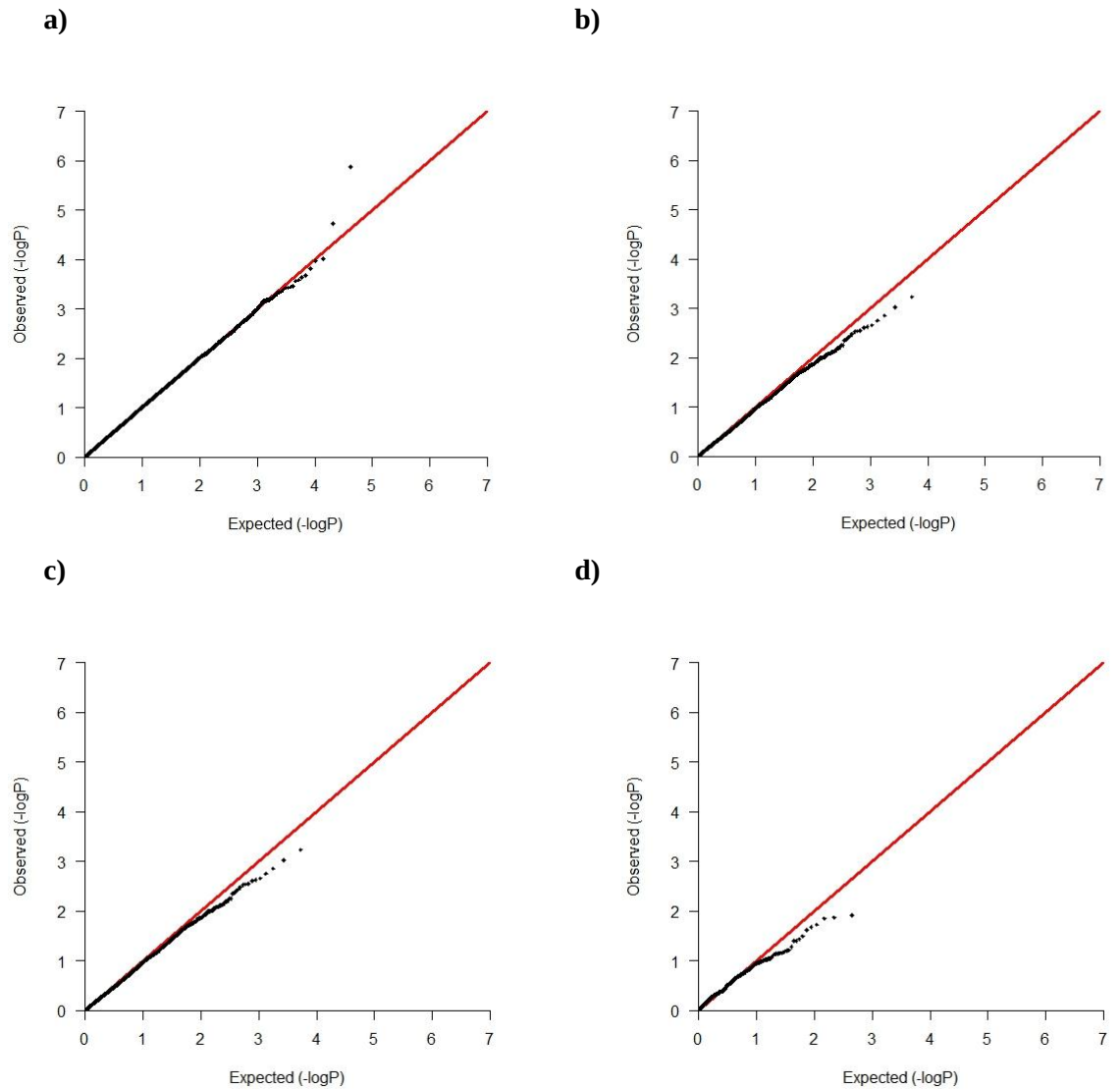
Figure 5-8 Q-Q p -value plots of genetic associations of lifetime tobacco use in 16-year-old adolescents with a) stress genes; b) circadian genes; c) overlap stress x circadian genes; and d) neurotransmitter stress x circadian genes. \lambda = 1.01 in the stress gene list; \lambda = 1 in the circadian gene list; \lambda = 1 in the overlap stress x circadian gene list; \lambda = 1.12 in the neurotransmitter stress x circadian gene list. All red lines indicate x = y .
