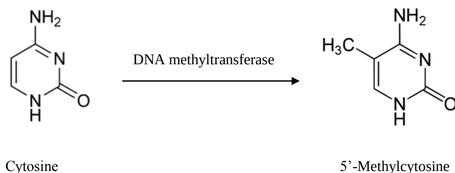
Figure 1-3 5'-cytosine methylation. The conversion of cytosine to 5'-cytosine methylation (DNA methylation) is catalysed by DNA methyltransferases. All known DNA methyltransferases use S-adenosyl methionine (SAM) as the methyl donor.
