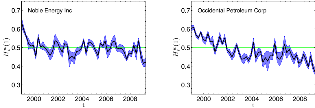
FIGURE 2.18: Weighed Generalized Hurst exponent H^w(q = 1) as a function of time for: Left panel - Noble Energy Inc.; Right panel - Occidental Petroleum.
