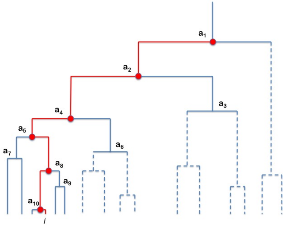
FIGURE 4.1: Example of hierarchical structure. The path highlighted in red is \Gamma_i , while the thick red bullets are the nodes a_m , m \in \gamma_i , which correspond to the risks stock i is exposed to. Note that the risk a_1 is common to all stocks, while other risks affect groups of stocks only. The dashed branches of the dendrogram indicate an arbitrary hierarchy.
