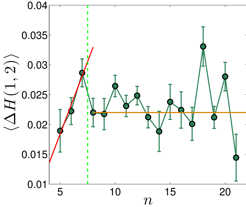
FIGURE 4.9: Correlation between multifractality and hierarchical order after detrending for stocks traded in TSE. We plot in green circles the average \langle \Delta H(1, 2) \rangle for each observed hierarchical order against the corresponding n . Error bars are standard errors on the mean, computed as s/\sqrt{N_n} , with N_n the number of stocks having order n and s the standard deviation on the mean. The red line is the best linear fit on the averages for n \in [5, 7] , while the orange line is the fit for n \in [8, 21] . The dashed line marks the end of the initial increasing trend.
