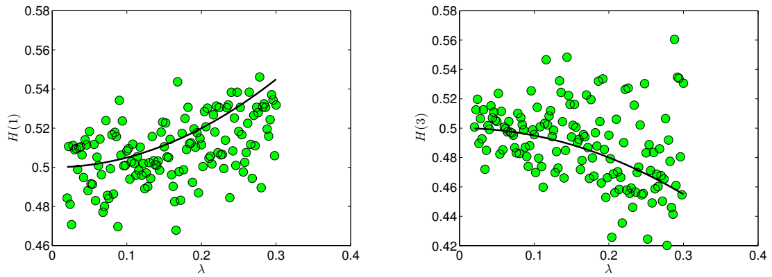
FIGURE 3.3: We plot the H(q) vs \lambda for q = 1 (left) and q = 3 (right). The dots refer to the H(q) 's values obtained from the MRW-simulated time series with \lambda ranging in [0.01, 0.3] , T = 500 and \sigma = 1 . The black solid lines are the theoretical relations (3.11) for q = 1, 3 . The GHE have been obtained with \tau_{max} varying between 10 and 30, whereas \Delta t has been set to \Delta t = 1 .
