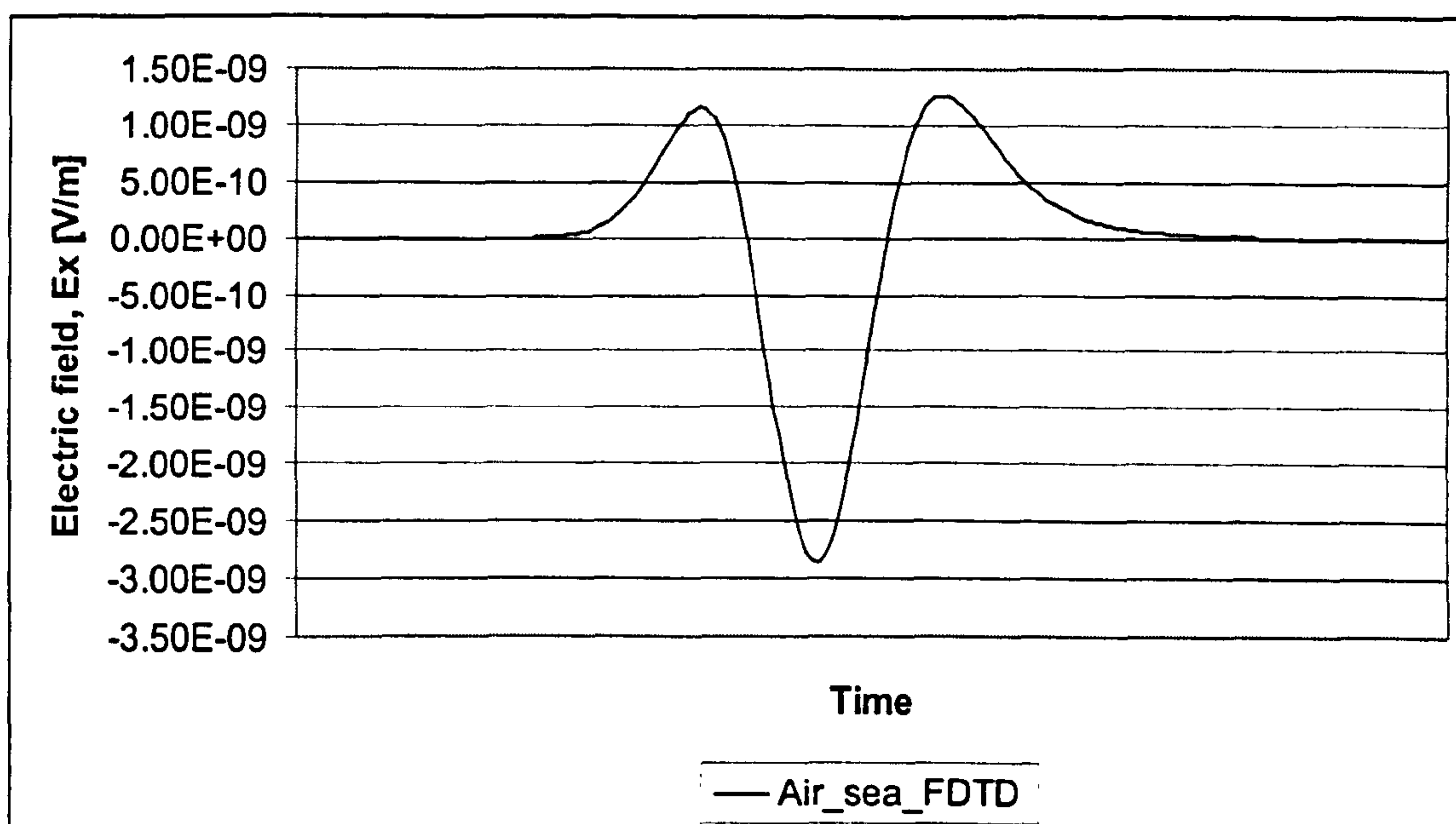
Figure B.5: FDTD solution for HED source at air-sea interface
