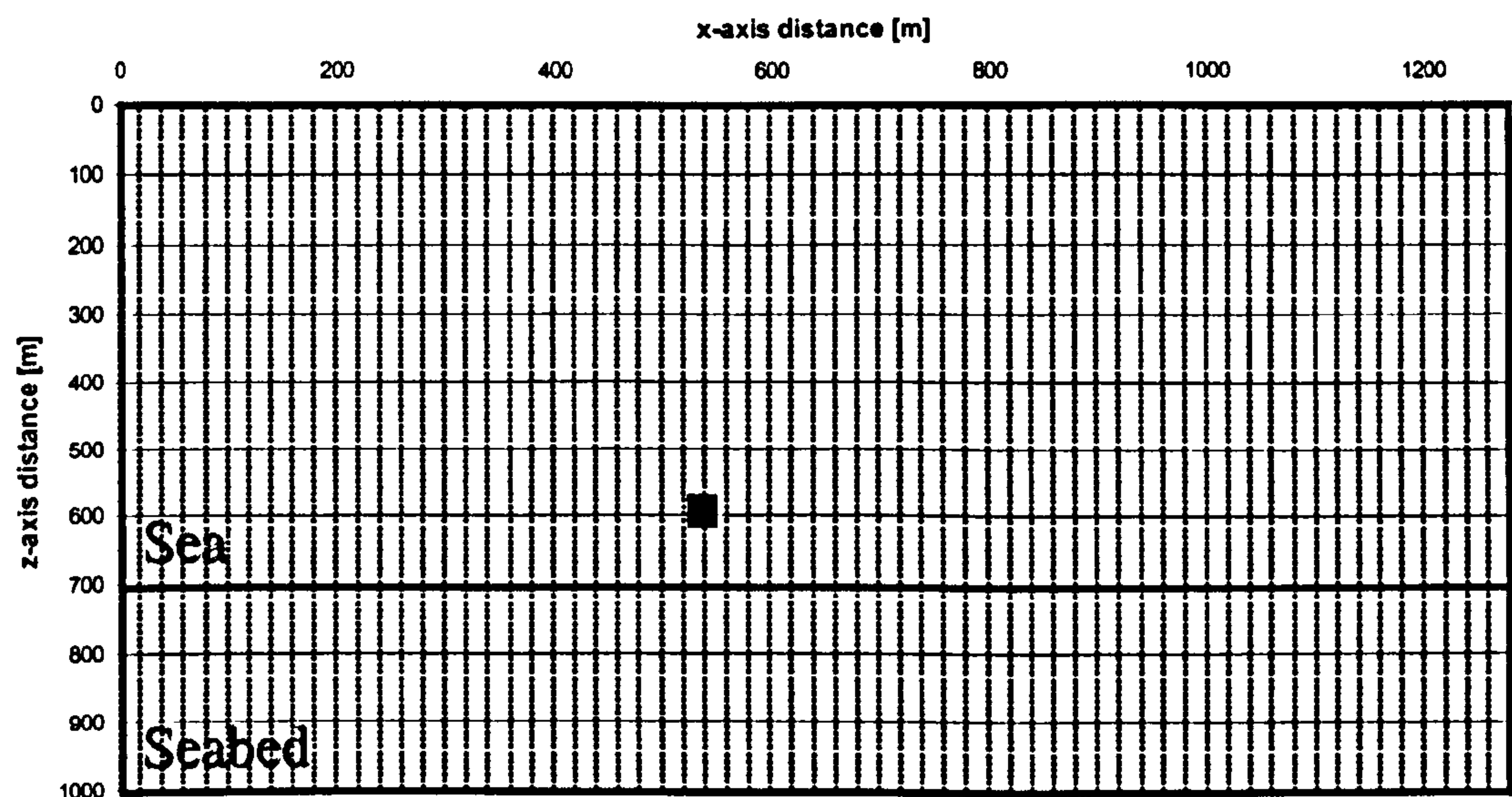
Figure 6.5: Transformed geometry
