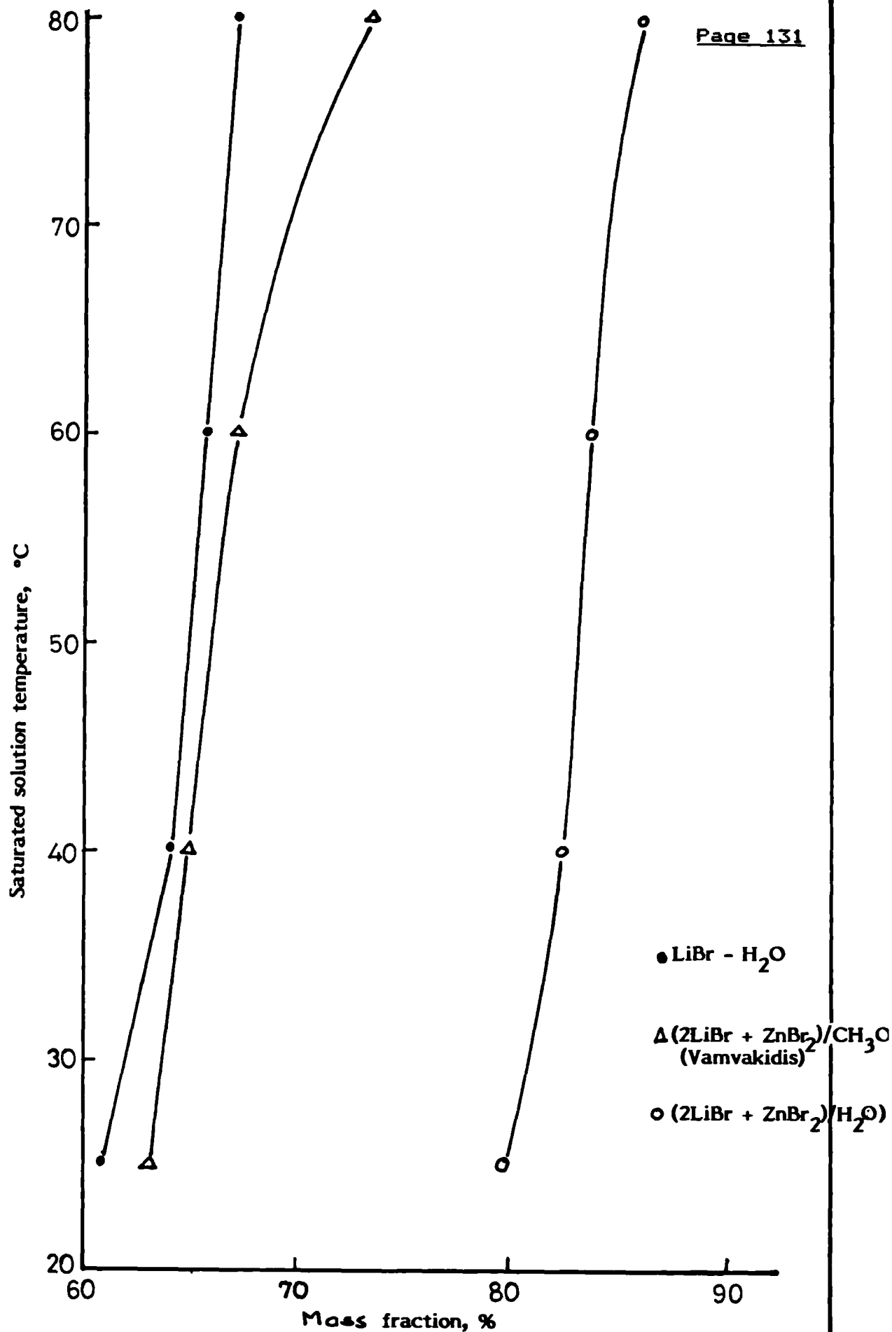
Fig. 4.4 Solubility of LiBr in H 2 O and (2LiBr + ZnBr 2 ) in H 2 O and in CH 3 OH
