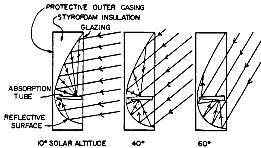
Fig. 2.4 Schematic of the Hot-Line Concentrator
