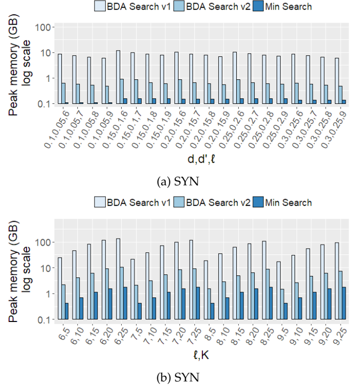
Fig. 11: Peak memory usage (GB) vs. (a) d, d', \ell , for K = 20 , and (b) \ell, K , for d = 0.15 and d' = 0.1 .
