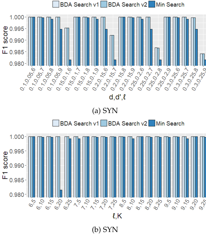
Fig. 9: F1 score vs. (a) d, d', \ell , for K = 20 , and (b) \ell, K , for d = 0.15 and d' = 0.1 .
