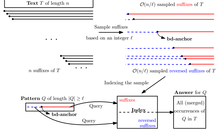
Fig. 1: An informal overview of our techniques: Given a text T of length n , we consider all of its n positions and sample them for a given integer \ell using the bd-anchors mechanism. The selected positions (bd-anchors) imply a set of \mathcal{O}(n/\ell) suffixes and a set of \mathcal{O}(n/\ell) reversed suffixes of T . We then index these strings, so as to answer pattern matching queries for patterns of length at least \ell . When such a pattern Q is given, we find any of its bd-anchors, which implies a suffix and a reversed suffix of Q , and query those using our index. Our index efficiently merges the partial results (i.e., occurrences of suffixes and reversed suffixes), and returns all occurrences of Q in T in nearly-optimal time.
