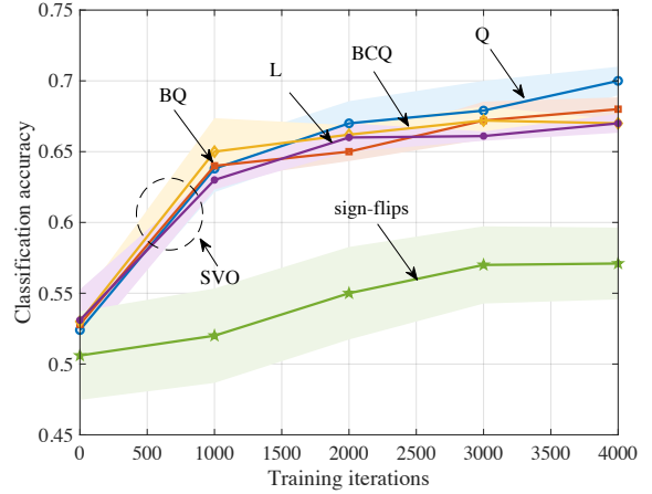
Fig. 2: Classification accuracy as a function of the training iteration for the benchmark sign-flips scheme [14] and the proposed SVO-based procedure for the BAS data set. The results are averaged over 5 independent trials.
