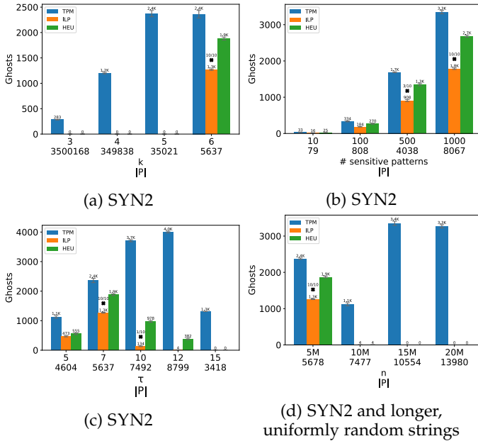
Fig. 5: Number of \tau -ghosts for varying: (a) k , (b) |S| , (c) \tau , and (d) n . An \star with ratio x/10 corresponds to an instance in which ILP was stopped after 1 hour to produce a feasible solution in x out of 10 runs.
