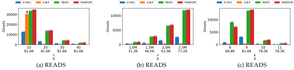
Fig. 6: Number of \tau -ghosts for varying: (a) \tau , (b) input string length n , and (c) k . The * symbol in (a) corresponds to an instance in which G-ILP was stopped after 1 hour to produce a feasible solution . ( \delta is the total number of #'s.)
