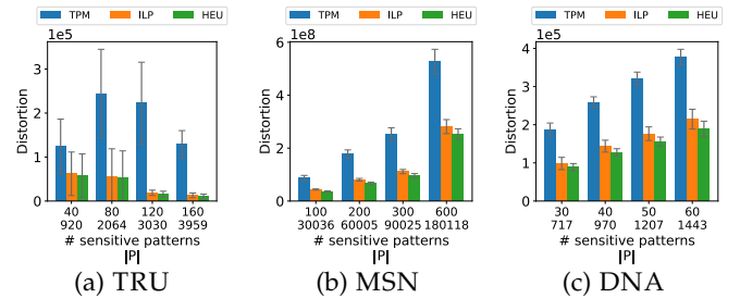
Fig. 3: Distortion for varying |\mathbf{S}| .
