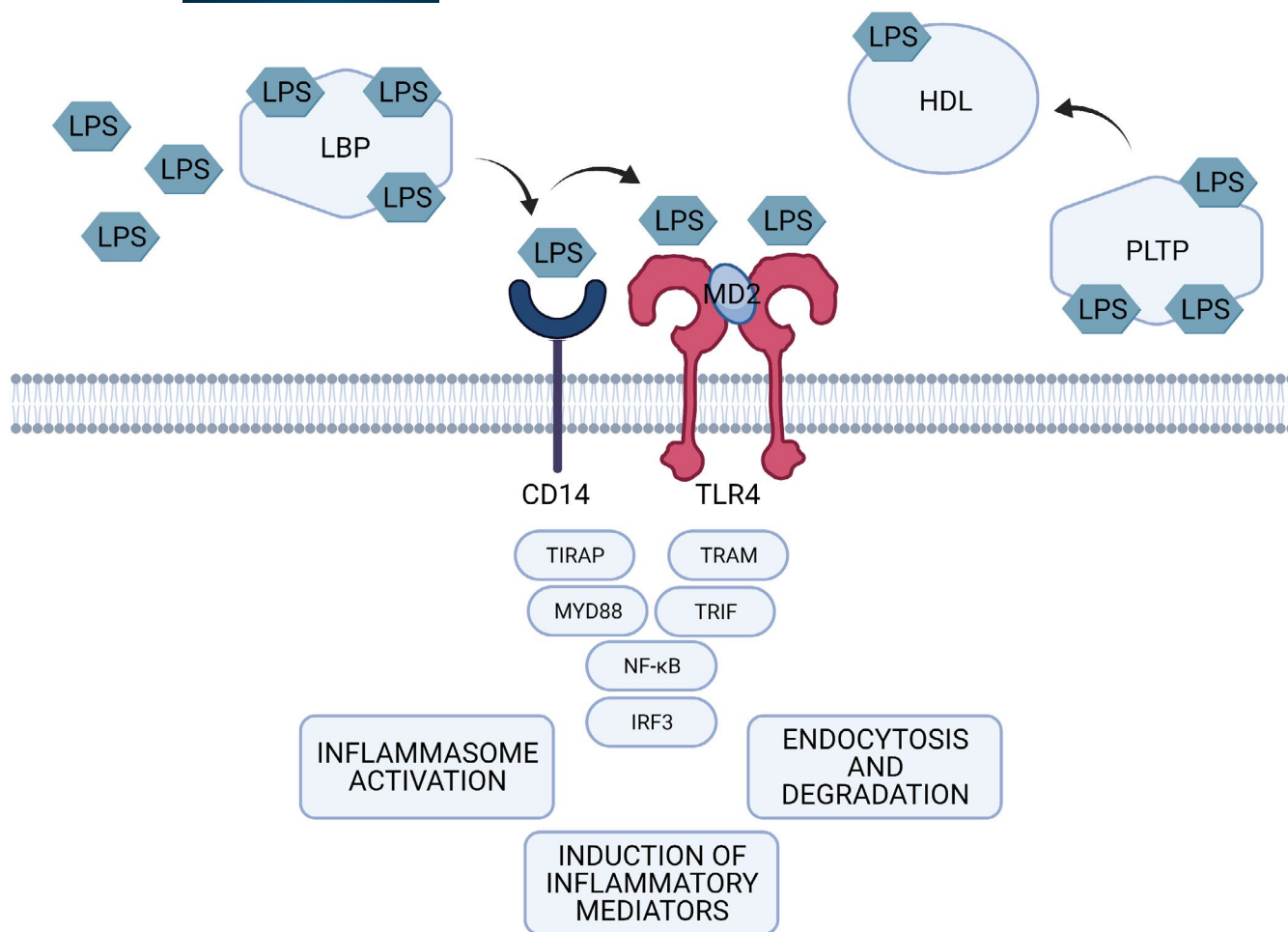
FIGURE 2 Lipopolysaccharide (LPS)-toll-like receptor 4 (TLR4) signaling. Lipopolysaccharide is recognized by the complex of toll-like receptor 4, cluster of differentiation 14 (CD14), and myeloid differentiation 2 (MD-2). Toll-like receptor 4 activation leads to the recruitment of additional effector proteins, including myeloid differentiation primary response protein 88 (MYD88), toll/interleukin-1 receptor domain-containing adapter protein (TIRAP), toll/interleukin-1 domain-containing adapter protein inducing interferon-beta-related adaptor molecule (TRAM), and toll/interleukin-1 domain-containing adapter protein inducing interferon-beta (TRIF). These further trigger a cascade enabling nuclear factor-κB (NF-κB) and interferon regulatory factor 3 (IRF3) to diffuse into the nucleus and to activate the transcription of cytokines, especially tumor necrosis factor alpha, interleukin-1beta, interleukin-6, and interleukin-8, and interferons, aiming at eliminating pathogens. In the circulation, lipopolysaccharide is transported by lipopolysaccharide binding protein (LBP), phospholipid transfer protein (PLTP), and by lipoproteins. Under standard physiologic conditions, lipopolysaccharide preferentially associates with high-density lipoprotein (HDL), which contributes to its clearance via the liver and bile
