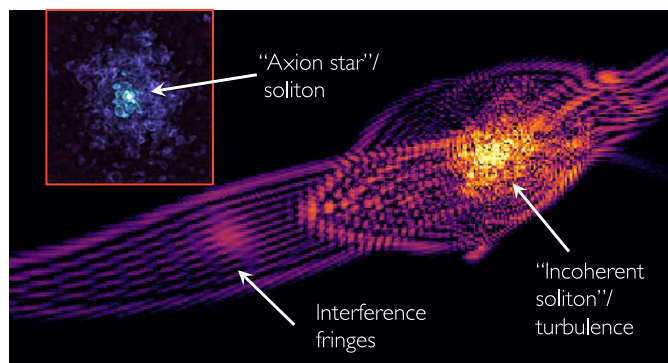
Fig. 5. Zoom in to part of the cosmic web formed by gravitational interactions and the interference of axion waves. The dense, almost spherical nodes of the web are DM halos, which host galaxies such as our own. The inset shows a volume rendering of such a halo. Notice the interference of coherent waves outside of DM halos forming interference fringes. Inside halos, there are self-bound solitonic objects at high density (“axion stars”) and turbulent waves in the outer regions (“incoherent solitons”). To make the unique wave effects visible on cosmic scales (kiloparsecs), a very low-particle mass, m_a \approx 10^{-22} eV, is used in this simulation. The same physics operates, and the same effects occur, however, for all types of bosonic DM, with the length scale set by the particle de Broglie wavelength. Figure adapted from work presented in (61, 62).
