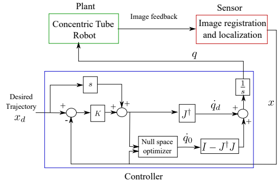
Fig. 2. Block diagram of the control loop.
