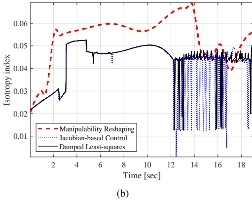
Fig. 3. Simulation results for CTR steering on a circular trajectory in 3 scenarios. (a) A comparison between the desired trajectory and actual trajectory. (b) A comparison of the isotropy index.
