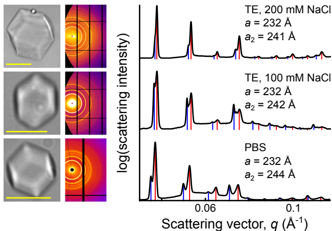
Figure 3: Self-assembly at low ionic strength. (left) Bright field images show rhombic-dodecahedral single crystals formed by l = 28 bp C-stars in low ionic strength buffers. (centre) 2D diffraction patterns. (right) Radially-averaged profiles. Red lines mark the best fit to the Bragg peaks of a BCC lattice with identical lattice parameter as for the frameworks formed by l = 28 bp C-stars in 300 mM NaCl (2b). Blue lines mark best fit to Bragg peaks of a secondary BCC phase with lattice parameter a_2 . Scale bars 10 \mu\text{m} .
