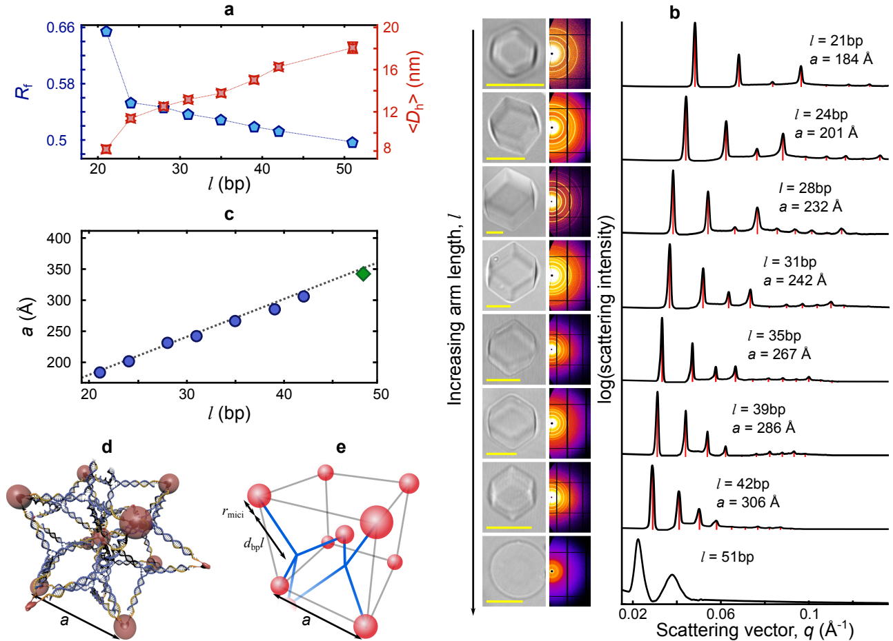
Figure 2: Controlling lattice parameter in C-star crystals. a , Structural characterization of individual nanostars lacking cholesterol functionalization. Increasing l leads to lower migration distance R_f and larger mean hydrodynamic diameter \langle D_h \rangle . b , (left) Bright field images show rhombic-dodecahedral single crystals for l = 21-42 bp, and spherical aggregates for l = 51 bp. Scale bars are 10 \mu\text{m} . SAXS powder diffraction patterns reveal that C-stars with arm length l = 21-42 bp form BCC crystalline phases. (Centre) 2D diffraction patterns. (Right) Radially-averaged profiles. Red lines mark best fit to Bragg peaks of a BCC lattice. C-stars with l = 51 bp (bottom) form an amorphous phase. c , Measured lattice parameter increases with l , and closely follows the expected value from geometrical arguments (dashed line). Blue circles indicate conventional C-stars, the green diamond the responsive design (Fig. 6). d , Plausible arrangement of C-stars in a BCC unit cell. 32 e , Abstracted view of unit cell. Here, solid blue lines represent DNA duplexes and red spheres represent micelles. For ease of visualization, only 2 nanostars are shown.
