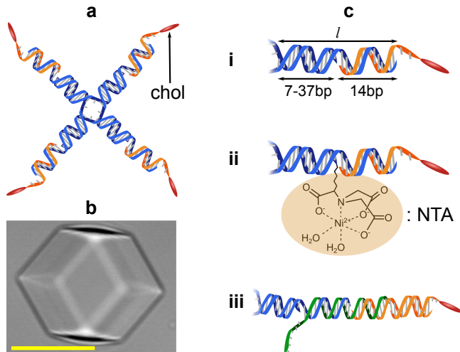
Figure 1: Topology preserving modifications in amphiphilic C-stars . a , C-stars are composed of 4 core-forming oligonucleotides (blue) and 4 cholesterol-functionalized strands (orange). b , Slow cooling of C-star samples leads to the formation of single crystals. Scale bar 30\ \mu\text{m} . c , Topology-preserving modifications include; (i) controlling arm length, (ii) inclusion of functional groups, here nitrilotriacetic acid (NTA), (iii) inclusion of DNA strand-displacement motifs.
