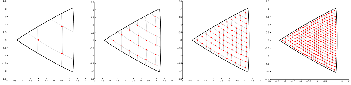
FIGURE 2. The lines expressing the quantization conditions (1.24) and the zeros of the polynomial \hat{Q}_n(x) computed numerically, for n = 2, 6, 12, 24 (from left to right). As can be seen, the zeros of \hat{Q}_n(x) form a regular pattern, a feature which was first observed in [5].
