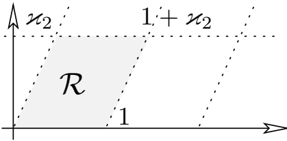
FIGURE 15. The fundamental region \mathcal{R}
