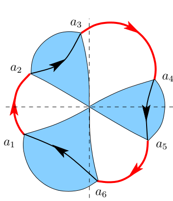
FIGURE 11. Deformation of the jump contour \gamma to the union of \mathcal{B} \cup \mathcal{L} . The branch cuts \mathcal{B} are indicated in red and \mathcal{L} in black. The picture corresponds to one possible choice of x \in \mathbb{C} : \text{dist}(x, \mathbb{C} \setminus \Delta) \geq \delta > 0 with \Re x > 0, \Im x > 0 .
