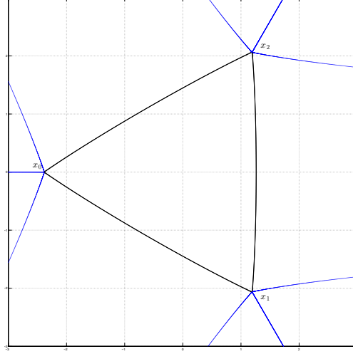
FIGURE 1. The star shaped region \bar{\Delta} = \Delta \cup \partial\Delta . The boundary \partial\Delta is given as the union of the three black solid curves.
