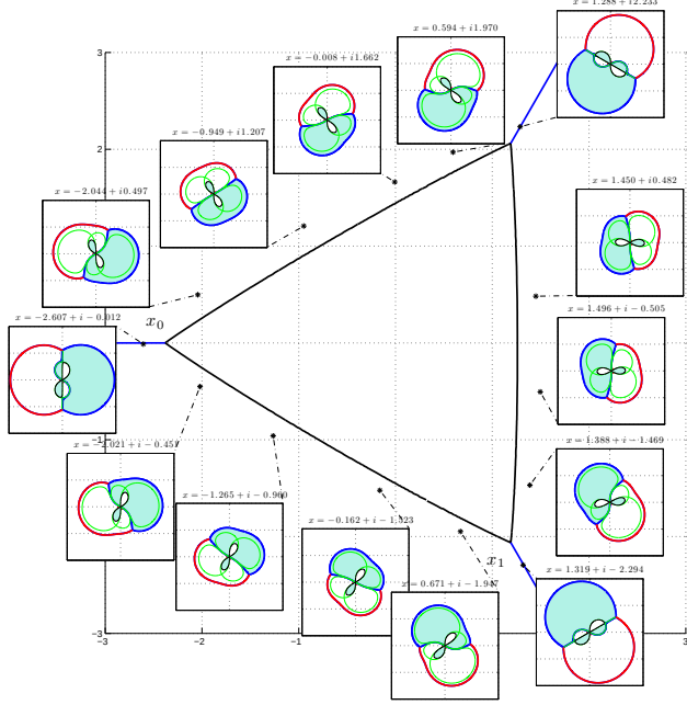
FIGURE 4. We plot the branch cut \mathcal{B} in red for several choices x \in \mathbb{C} : \text{dist}(x, \overline{\Delta}) \geq \delta > 0 . The level sets \Phi(z) = \Re \varphi(z) = 0 are shown as solid blue lines and the shaded regions indicate where \Phi(z) > 0 . In the white regions we have \Phi(z) < 0 and along the green lines \Phi(z) \equiv \Phi(\pm(2a)^{-\frac{1}{2}}) .
