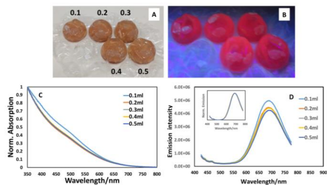
Figure 3 – a) Photograph of \text{CuInS}_2 quantum dots after various volumes (numbers shown in mL) of ZnS precursor had been added; b) Photograph of materials in previous figure under 365 nm excitation; c) Normalised absorption spectra of \text{CuInS}_2/\text{ZnS} quantum dots prepared using different amounts of ZnS precursor; d) Emission spectra of \text{CuInS}_2/\text{ZnS} quantum dots prepared using different amounts of ZnS precursor. Inset, normalised spectra showing spectral position. The data shows that addition of varying amounts of shell precursor had little effect on the optical properties of \text{CuInS}_2/\text{ZnS} .
