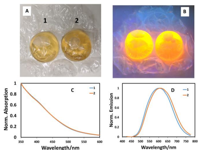
Figure 2 – a) Photograph of two sets of \text{CuInS}_2/\text{ZnS} quantum dots prepared by a stand-alone method in two adjacent bubbles using the optimised conditions (Cu:In ratio of 1:10, followed by addition of 0.2 mL ZnS precursor solution); b) Photograph of \text{CuInS}_2/\text{ZnS} quantum dots used in previous figure excited at 365 nm; c) Normalised absorption spectra of the two samples shown in previous figures; d) Normalised emission spectra of the two samples shown in previous figures. This data shows that \text{CuInS}_2/\text{ZnS} quantum dots can be simply prepared using sequential precursor addition in a bubble, and that the method is reproducible.
