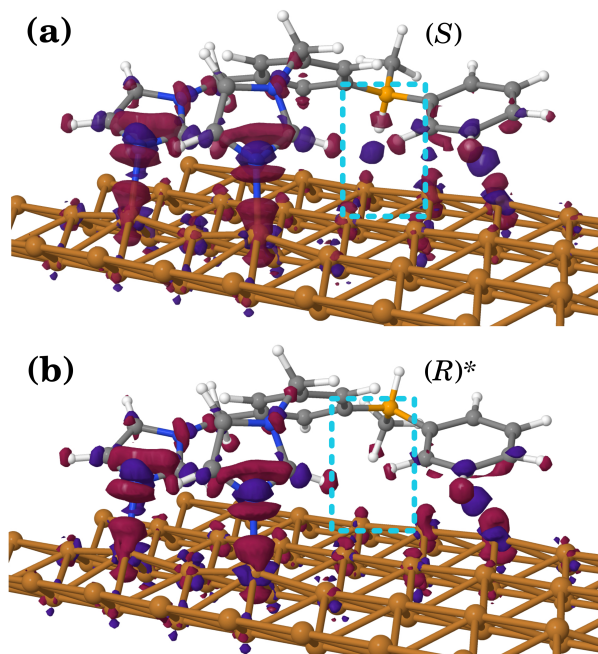
Figure 3: Comparison of the electronic density difference maps between the ( S ) (a) and ( R )* (b) conformers of the BIPEB molecule adsorbed on the Cu (110) surface. Red (negative) and purple (positive) isosurfaces correspond to \pm 0.003 electron/ \text{\AA}^3 . White, grey and blue balls stand for H, C and N atoms, respectively. The orange ball represents the stereogenic carbon atom, responsible for the different orientations of the methyl group and of the H atom of the enantiomers on the surface. The region where the interaction of the molecule with the surface differs is highlighted by the cyan dashed boxes.
