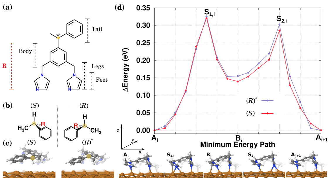
Figure 1: (a) BIPEB molecule. The chiral centre is highlighted in yellow. (b) The ( S ) and ( R ) enantiomers representation in their 3D projection. Dashed line indicates a mirror plane. (c) Two relaxed geometries considered here, as viewed from the tail to show the chiral centre (yellow). The shown geometry of ( S ) is the most energetically favourable. The considered relaxed geometry ( R )*, that is related to enantiomer ( R ) as one of its conformers, is by 0.1 eV less stable than ( R ) (which mirrors ( S ) exactly), and hence represents a metastable structure. (d) Top: DFT CI-NEB calculated change of the PES of the two enantiomers, ( S ) and ( R )* along the diffusion path. Bottom: a legs view of selected geometries (the minima and saddle points) of the ( R )* enantiomer during its 1D diffusion along the Cu row. The ( S ) or ( R )* molecules go through a set of equivalent geometries with the corresponding difference due to their centre of chirality as shown in (c).
