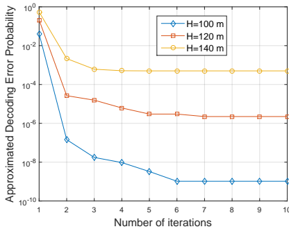
Fig. 3: Convergence behaviour of Algorithm 3 for various H .
