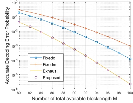
Fig. 4: Performance comparison for various algorithms.
