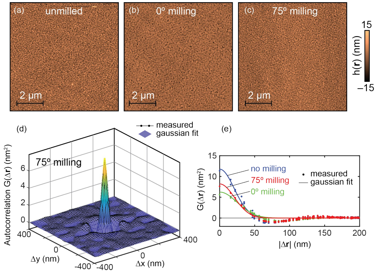
Fig. 4. AFM topography of the three aluminium surfaces (a) unmilled, (b) 0° milled and (c) 75° milled. (d) 2D correlation function corresponding to the image (c) fitted with a Gaussian. (e) 2D correlation function for the three measurements (a-c), projected into the radial displacement variable.
