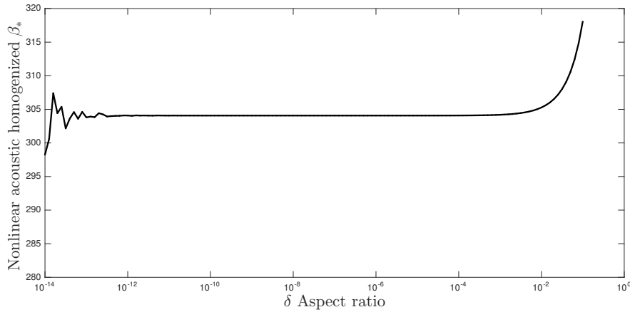
Figure 5: Illustrating the variation in the effective compressive nonlinearity coefficient of the cracked medium \beta_* as a function of the crack aspect ratio \delta . It is noted that this parameter is relatively insensitive to variations in \delta for 10^{-12} < \delta < 10^{-2} .
