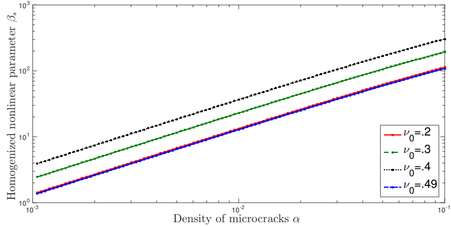
Figure 4: Illustrating the variation in the effective compressive nonlinearity coefficient of the cracked medium \beta_* as a function of the crack density parameter \alpha , as defined by (54). The four curves relate to different host medium Poisson ratios. Here it should be noted that two orders of magnitude change in \alpha leads to two orders of magnitude change in \beta_* . This is in stark contrast to the variation in \mathcal{E}_* with \alpha as noted in Figure 3.
