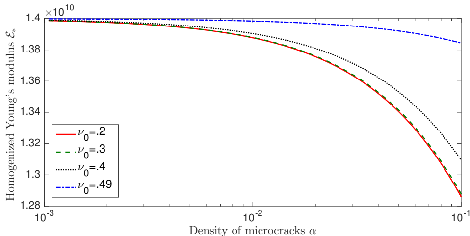
Figure 3: Illustrating the variation in the linear elastic Young's modulus of the cracked medium \mathcal{E}_* as a function of the crack density parameter \alpha , as defined by (53). The four curves relate to different host medium Poisson ratios. In particular it should be noted that two orders of magnitude change in \alpha leads to a very small change in the predicted \mathcal{E}_* .
