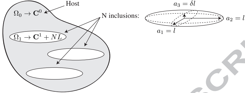
Figure 1: Outline of the considered medium: dispersion of nonlinear spheroidal inclusions in a linear isotropic host with distribution of microcracks defined by density \alpha = \phi/\delta where \phi is the volume fraction.
