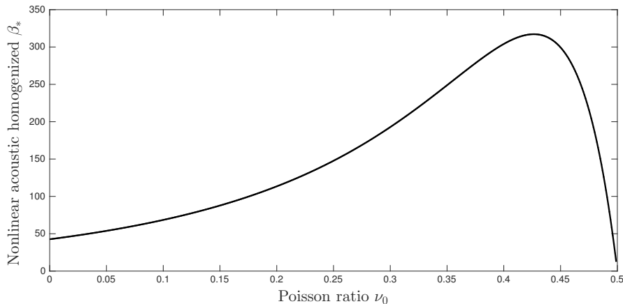
Figure 6: Illustrating the variation in the effective compressive nonlinearity coefficient of the cracked medium \beta_* as a function of the host Poisson ratio \nu_0 . It is noted that for bone \nu_0 \approx 0.4 , meaning that this is close to where \beta_* reaches a maximum.
