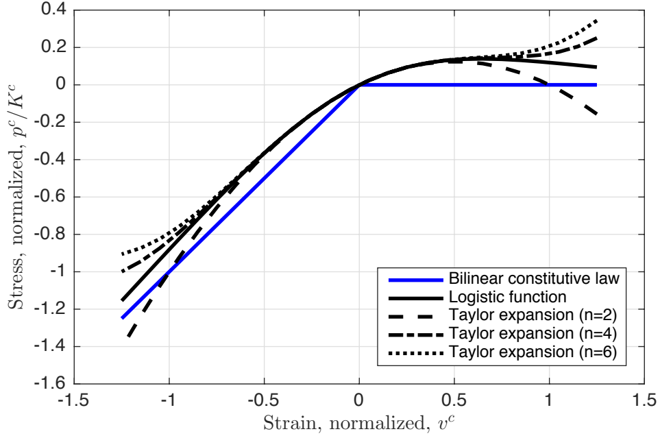
Figure 2: Illustration of the exact bilinear constitutive law, its approximation via the logistic function and associated Taylor expansions, employing the fitting parameter combination \delta^2 \mathcal{N} = 7.2 \times 10^4 .
