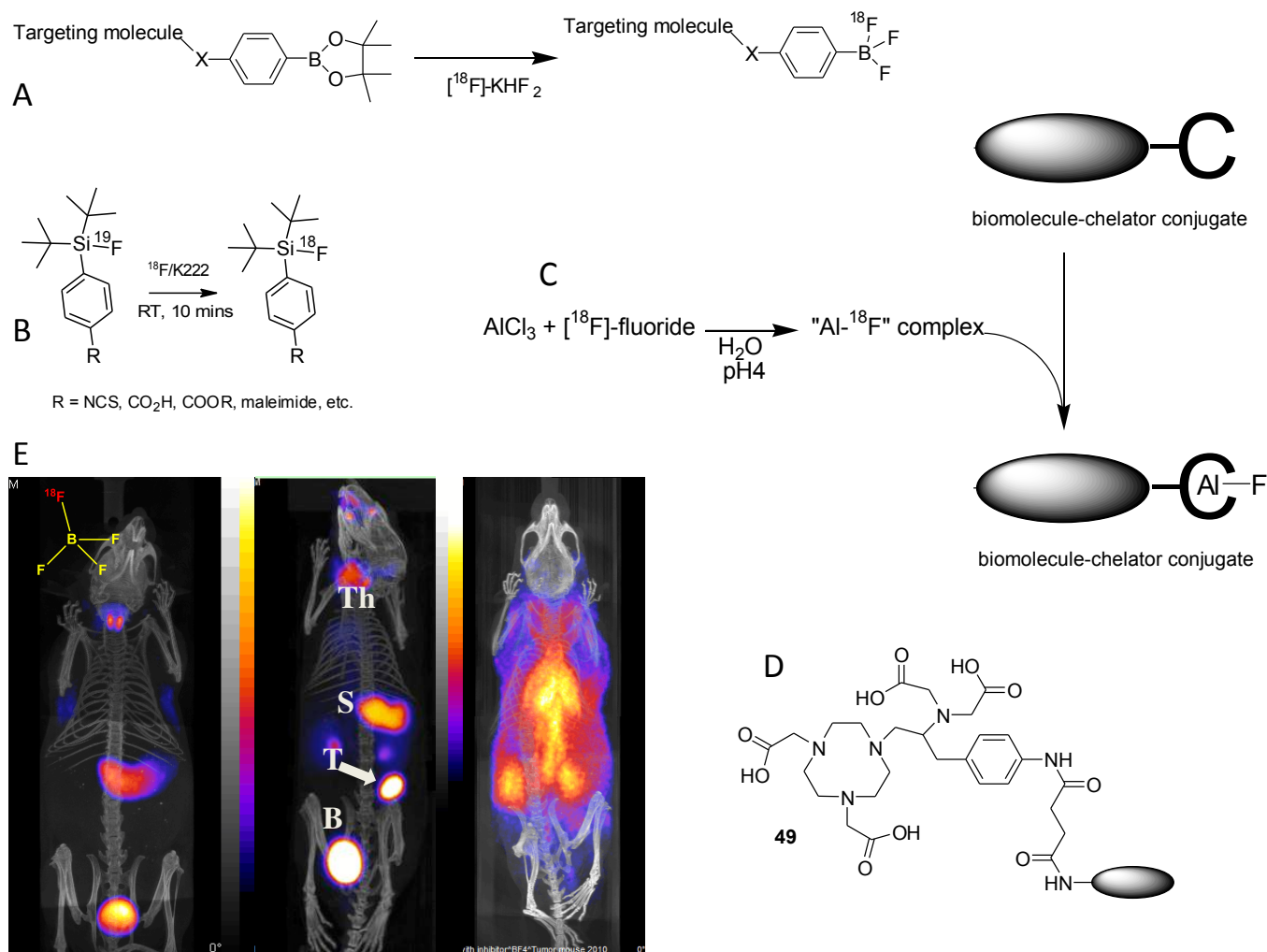
Figure 18: A: Nucleophilic radiolabelling of boronic ester prosthetic group; B: Isotopic exchange labelling of fluorosilane prosthetic group; C: Use of coordinatively unsaturated aluminium complex as a binding site for fluoride ions in biomolecule labelling; D: currently favoured ligand for chelation of \text{Al}^{3+} and labelling with ^{18}\text{F} -fluoride; E: PET-CT imaging of sodium/iodide symporter (NIS) activity mouse using NIS substrate ^{18}\text{F} - \text{BF}_4^- , 30 min post-injection. Left: normal mouse showing thyroid and stomach uptake and excretion into bladder; Centre: mouse with implanted NIS-expressing breast tumour showing tumour (T) uptake as well as thyroid (Th) and stomach (S) uptake; right: normal mouse pre-injected with perchlorate to block NIS activity, showing radioactivity largely confined to blood pool.
