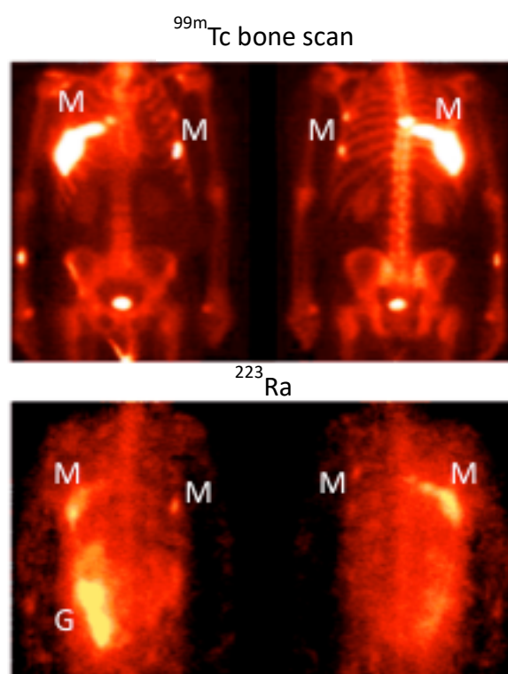
Figure 3: Biodistribution of ^{223}\text{Ra} in a patient with metastatic prostate cancer after i.v. administration of ^{223}\text{RaCl}_2 . 5 The anterior (left) and posterior (right) views show specific uptake in the sites of bone metastases indicated by the ^{99\text{m}}\text{Tc} bone scan (M), and activity in the gut (G) indicating radioactivity that has undergone hepatobiliary excretion. The gamma camera image was possible by virtue of a low abundance gamma emission from ^{223}\text{Ra} accompanying the alpha decay. (Adapted with permission from ref. 5).
