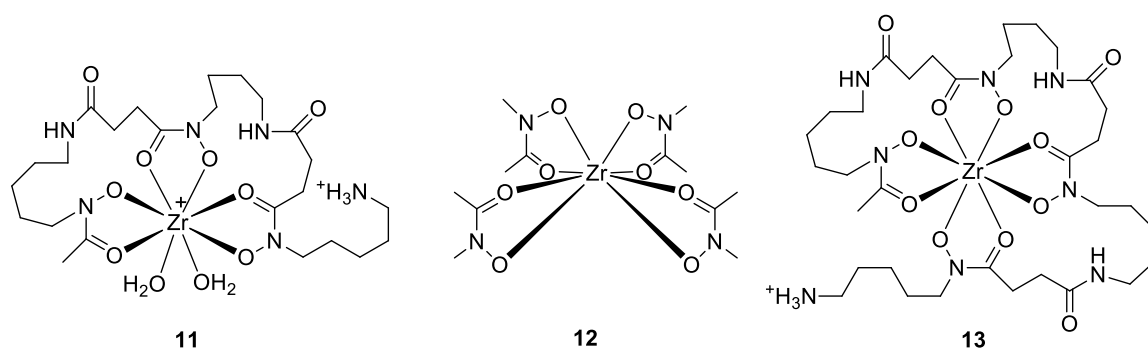
Figure 5: Left: Modelled coordination of \text{Zr}^{4+} by DFO ( 11 ); 20 Centre: Schematic structure of \text{ZrL}_4 ( \text{HL} = N -methylacetohydroxamic acid) ( 12 ), serving as a template for the design of new octadentate chelators for \text{Zr}^{4+} (note that disorder in the C and N orientations of the hydroxamate rings precludes determination of their preferred relative orientation and suggests that any such preferences are weak); 22 Right: Schematic structure of \text{Zr}^{4+} complex 13 of an octadentate DFO homologue. 23
