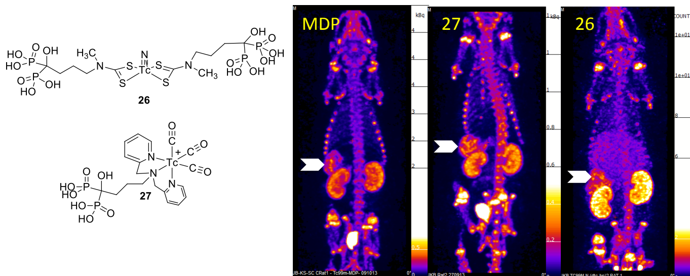
Figure 10: SPET images (maximum intensity projection) of vascular calcification in a mouse model 30 min after injection with [ ^{99m}\text{Tc} ]-MDP, [ ^{99m}\text{Tc} ]-27 and [ ^{99m}\text{Tc} ]-26. Arrows indicate uptake in calcified mesenteric arteries. Uptake in bone and clearance via kidneys and bladder is also evident.
