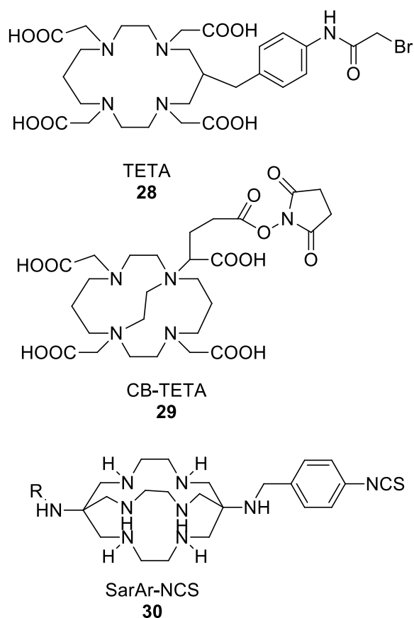
Figure 12: Selection of chelators for radioisotopes of Cu 2+ ; others of significance include 1 and 5 from Fig. 4.
