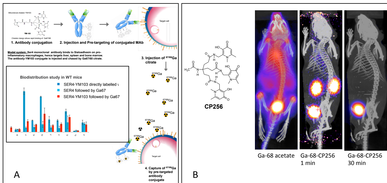
Figure 15: A. Concept of pre-targeting by in vivo transchelation of ^{68}\text{Ga} , which is feasible with YM103 ( 4 in Fig. 4) because of its ability to transchelate \text{Ga}^{3+} from transferrin in plasma and in vivo . Inset: Uptake of ^{68}\text{Ga} in most organs (including spleen which is the location of the macrophages expressing sialoadhesin, the SER4 antibody target) when given as a chase after administration of antibody-YM103 conjugate, is intermediate between that of the pre-labelled antibody and the distribution of ^{68}\text{Ga} given as a chase after administration of unconjugated antibody. The exception is bone, which is the target of unchelated ^{68}\text{Ga} (see part B, left image). This suggests that ^{68}\text{Ga} is able to find and bind to the pre-targeted antibody-YM103 conjugate in vivo . B: Demonstration that the tris(hydroxypyridinone) chelator CP256 (non-derivatised form of YM103) can bind to ^{68}\text{Ga} in vivo and excrete it rapidly via kidney. Left: Biodistribution of ^{68}\text{Ga} administered in unchelated form; centre and right: biodistribution of ^{68}\text{Ga} -CP256 complex 1 min and 30 min post-injection respectively, showing rapid renal excretion in progress and completed. Similar images are obtained if the ^{68}\text{Ga} is administered first, followed by the CP256 ligand.
