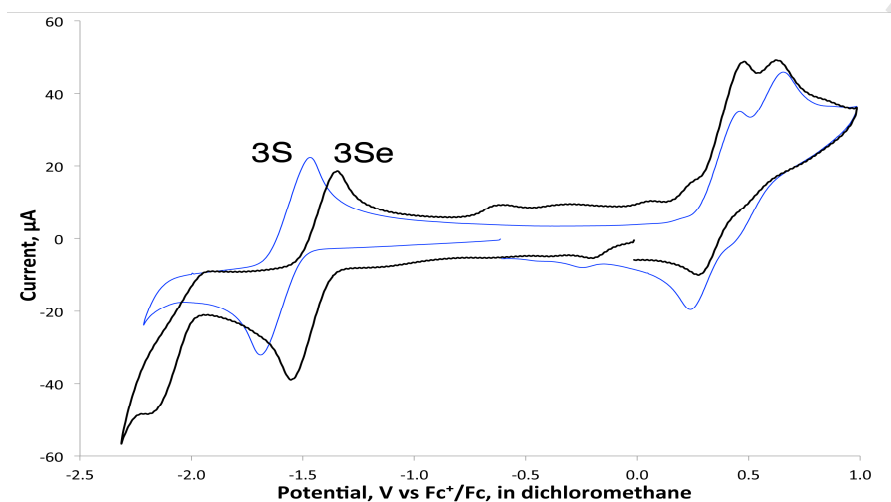
Figure 7. CVs of [\text{Fe}_3(\text{CO})_7(\mu_3\text{-S})_2(\mu\text{-dppm})] ( 3S ) (blue) and [\text{Fe}_3(\text{CO})_7(\mu_3\text{-Se})_2(\mu\text{-dppm})] ( 3Se ) (black) in \text{CH}_2\text{Cl}_2 (1 mM solution, supporting electrolyte [\text{NBu}_4][\text{PF}_6] , scan rate 0.25 \text{ V s}^{-1} , glassy carbon electrode, potential vs \text{Fc}^+/\text{Fc} ).
