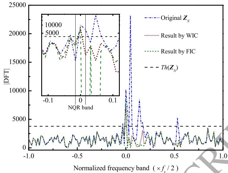
FIG. 15. (Color online) The spectra of a run of the original data and the interference canceled data of the experimental test. “|DFT|” means the absolute value of Discrete Fourier transformation of data. The embedded subgraph zooms in the area around NQR band, with its vertical axis of logarithm to the base 10.
