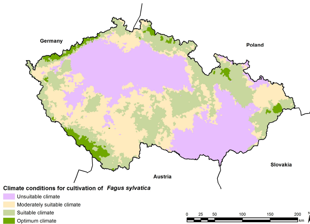
Figure 5. Visualization of predicted distribution of climate conditions for the European beech in the Czech Republic in 2070.
