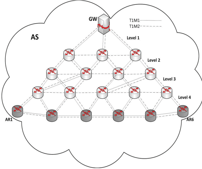
Fig. 1: Autonomous system comprised of 19 nodes and 32/41 links. Average node degree: 3.36/4.32. Total capacity: 11.94/15.34 (Gb). 4 and 5 RPs respectively.
