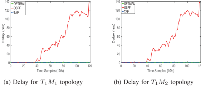
Fig. 2: Delay for our investigated topologies
