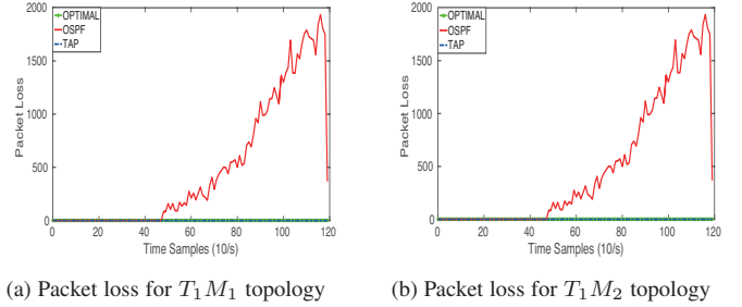
Fig. 4: Packet Loss for our investigated topologies
