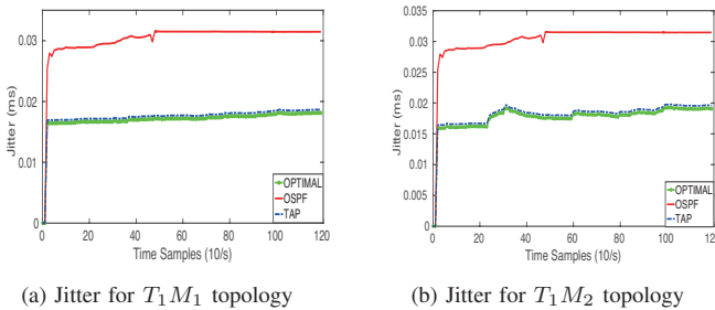
Fig. 3: Jitter for our investigated topologies
