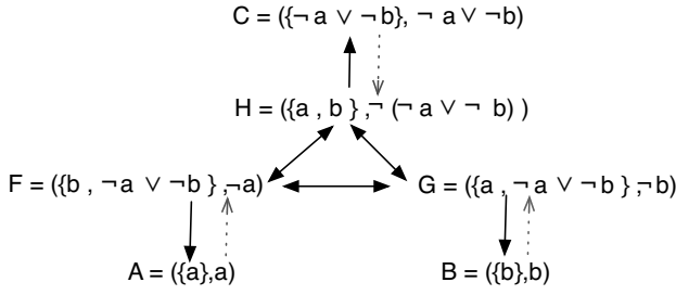
Figure 1. Attacks on premises are solid arrows. Dotted arrows are additional attacks if attacks can target conclusions.
