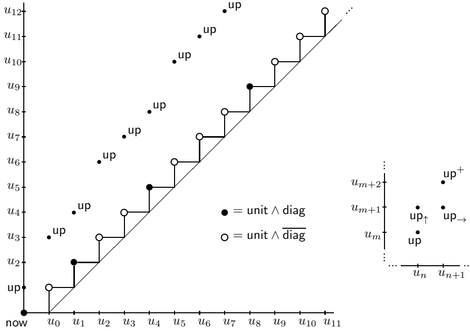
Fig. 9. Encoding the n\omega \times \omega -grid in an \mathcal{HS} -model: version 1.
