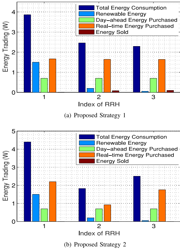
Fig. 7. Optimal energy trading for proposed strategies at \gamma = 30 dB.
