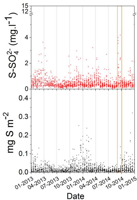
5 Figure 9 UK Precip-Net data: All fortnightly site data for 2013 and 2014; Upper panel: S-SO 4 2- concentrations; Lower panel: Sulfur deposition (mg S m -2 ); Note fortnightly data with data plotted using the start date of the measurement period. (Data downloaded from UK-Air on 25/06/2015 and 02/02/2016).
