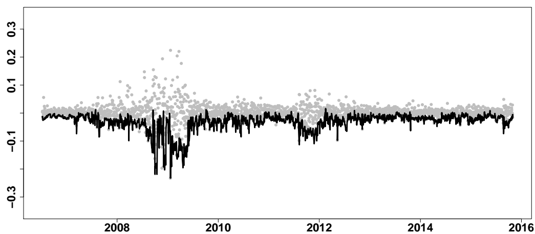
Figure 9: Log returns of JPM (grey) and VaR of log returns of JPM (black), \tau = 0.05 , T = 2335 , window size n = 126 , refer to (5.2).
