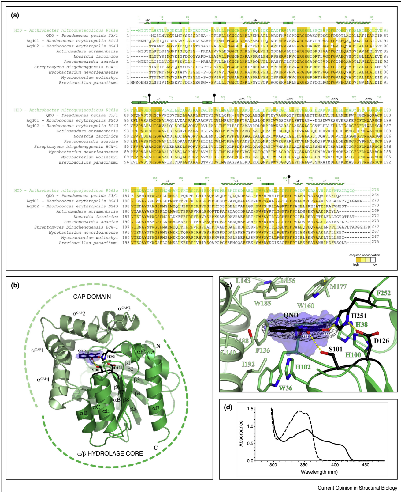
Carbon monoxide (CO)-forming cofactor-independent 2,4-dioxygenases. (a) Sequence alignment of various bacterial proteins exhibiting high similarity to A. nitroguajacolicus Rù61a 1-H-3-hydroxy-4-oxoquinaldine 2,4-dioxygenase (HOD). Residues are highlighted in different shades of
