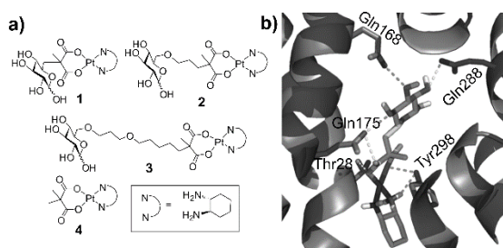
Figure 1. (a) Structures of Glc-Pts 1-3 and their aglycone 4 . (b) The hydrogen-bonding interactions present in the docking model of 1 into XylE (PDB 4GBZ). [9] The protein is shown as grey ribbons with the sidechains of key residues depicted as sticks. Complex 1 is shown as sticks and polar hydrogen atoms are explicitly portrayed. Hydrogen-bonding interactions are illustrated with dashed lines (See Figure S23 for the colored version of the docking model).
