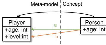
Fig. 2. Example of two different valid bindings of the same meta-model and a model concepts.
