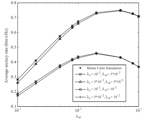
Fig. 6. The average secrecy rate versus \lambda_{ap} . P_{ap} = 30 dBm, M = 2 , \rho_s = 0.01 , \rho_{ap} = 0.1 , \alpha = 2.8 , \beta = 3.2 , \lambda_e^s = \lambda_e^{ap} = 5 \times 10^{-3} .
