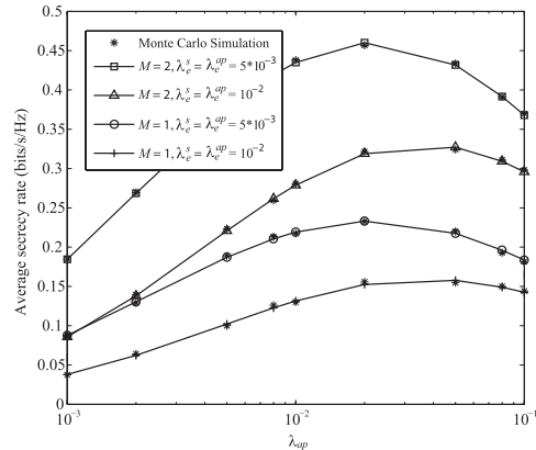
Fig. 7. The average secrecy rate versus \lambda_{ap} . P_{ap} = 30 dBm, \rho_s = 0.01 , \rho_{ap} = 0.1 , \alpha = 2.8 , \beta = 3.2 , \lambda_s = \lambda_{sk} = 10^{-2} .
