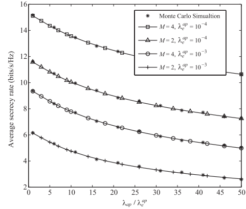
Fig. 4. The average secrecy rate versus \frac{\lambda_{ap}^{ap}}{\lambda_{ap}} . \rho_{ap} = 0.1 , \lambda_{sk} = 10^{-2} , \beta = 3.5 , P_{ap} = 15 dBm.
